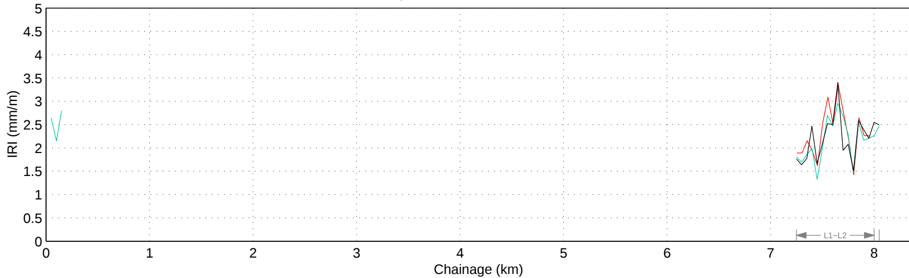
Hwy 1A:08 Mean IRI – Right Lane
