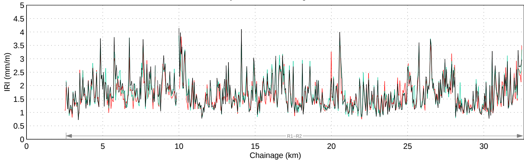
Hwy 1:02 Mean IRI – Right Lane
