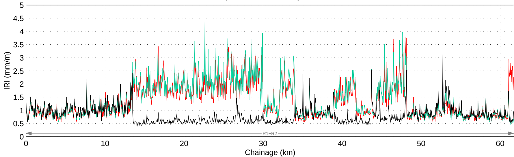
Hwy 1:14 Mean IRI – Right Lane
