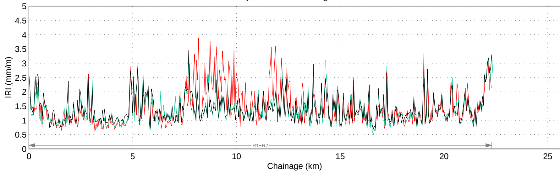
Hwy 1:04 Mean IRI – Right Lane
