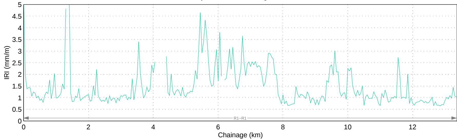
Hwy 1:21 Mean IRI – Right Lane
