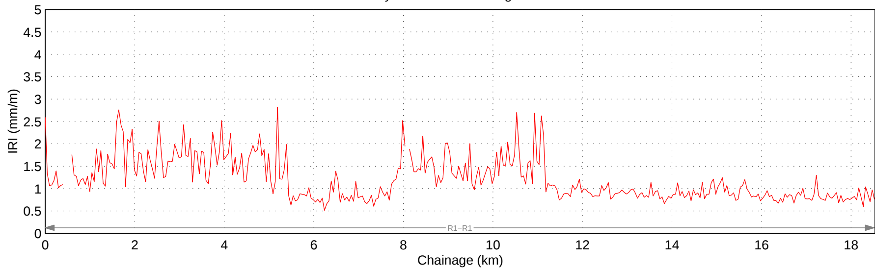
Hwy 1:10 Mean IRI – Right Lane
