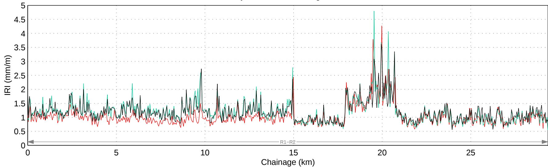
Hwy 1:12 Mean IRI – Right Lane
