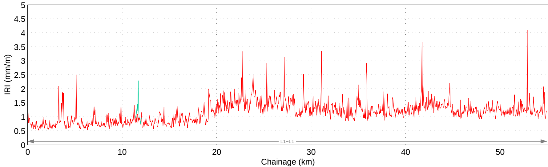
Hwy 1:18 Mean IRI – Right Lane
