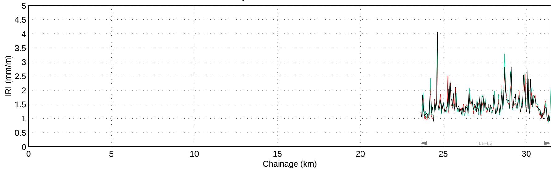
Hwy 1A:06 Mean IRI – Right Lane
