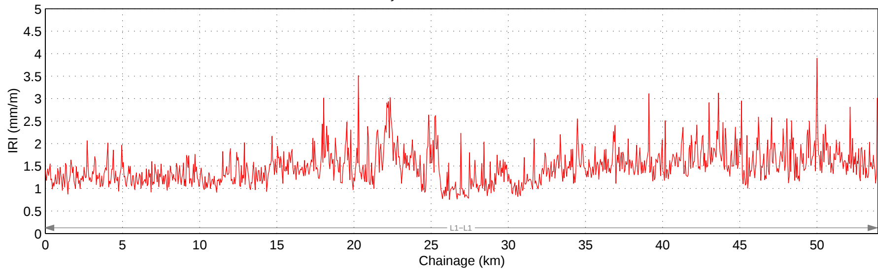
Hwy 1:20 Mean IRI – Right Lane
