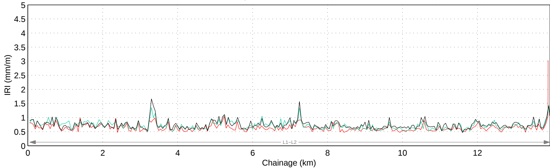
Hwy 1:08 Mean IRI – Right Lane
