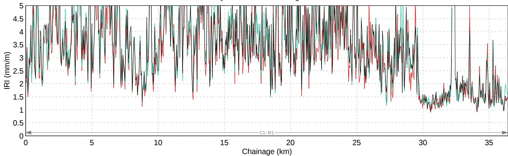
Hwy 1A:04 Mean IRI – Right Lane
