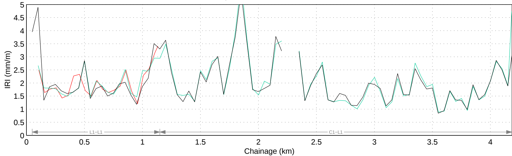
Hwy 1X:02 Mean IRI – Right Lane
