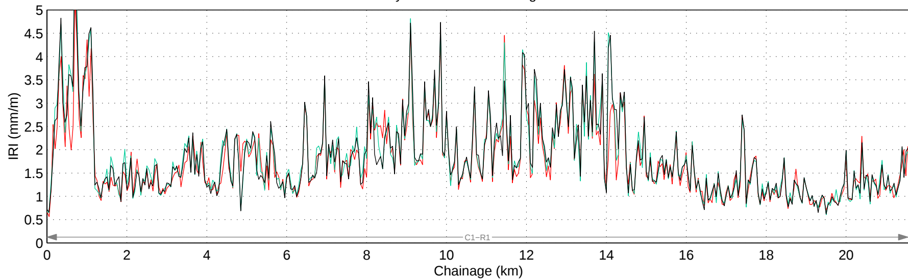
Hwy 1A:02 Mean IRI – Right Lane
