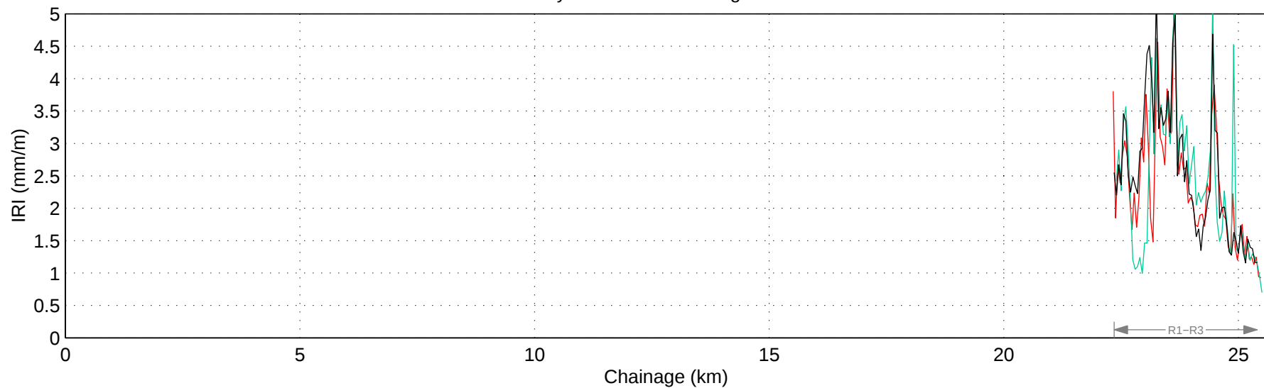
Hwy 1:04 Mean IRI – Right Lane
