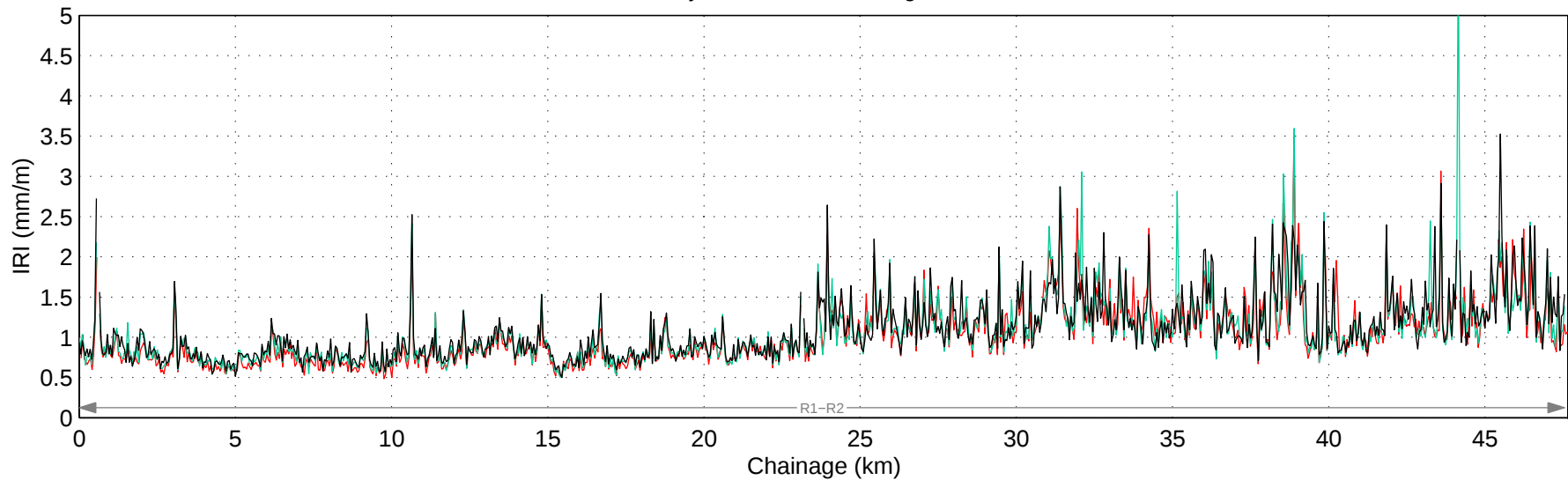
Hwy 1:22 Mean IRI – Right Lane
