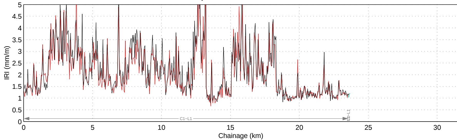
Hwy 1A:06 Mean IRI – Right Lane
