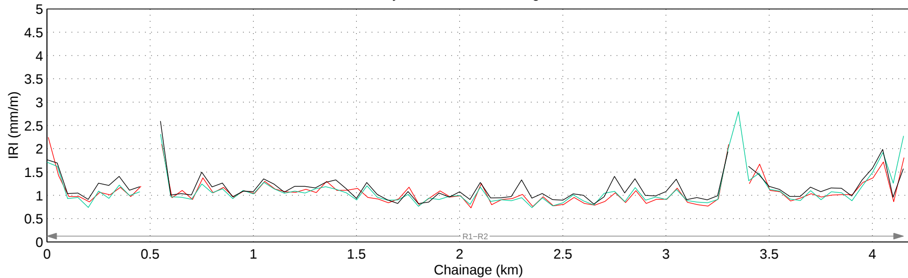
Hwy 100:02 Mean IRI – Right Lane
