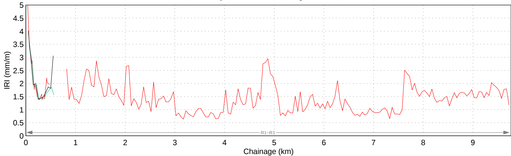
Hwy 216:04 Mean IRI – Right Lane
