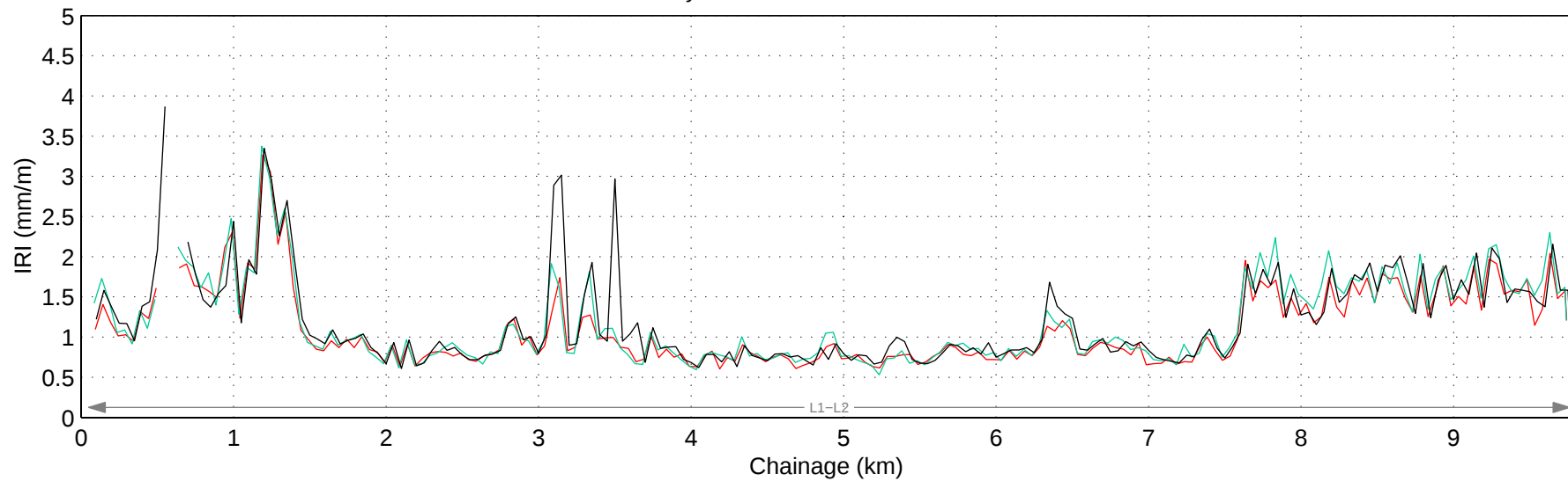
Hwy 216:04 Mean IRI – Right Lane
