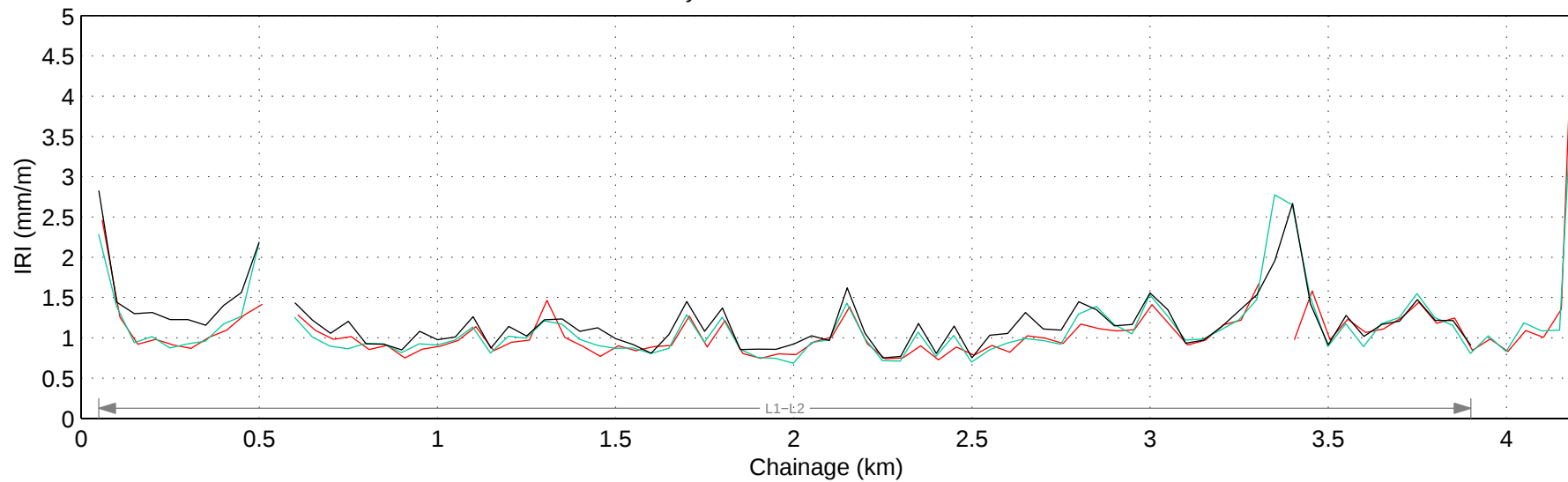
Hwy 100:02 Mean IRI – Right Lane
