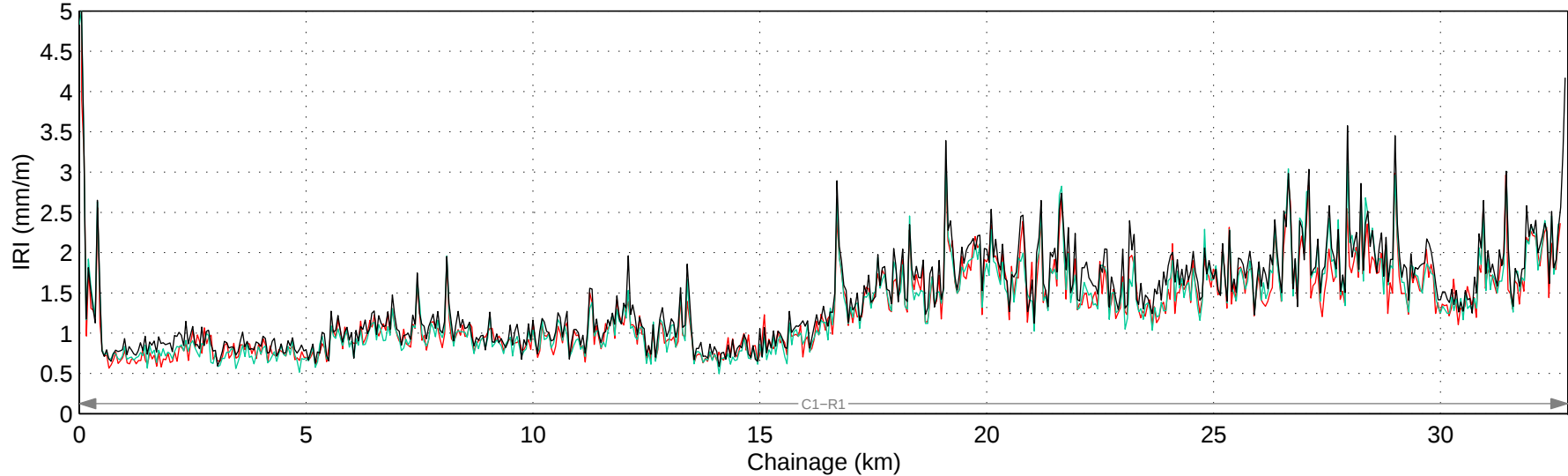
Hwy 520:04 Mean IRI – Right Lane
