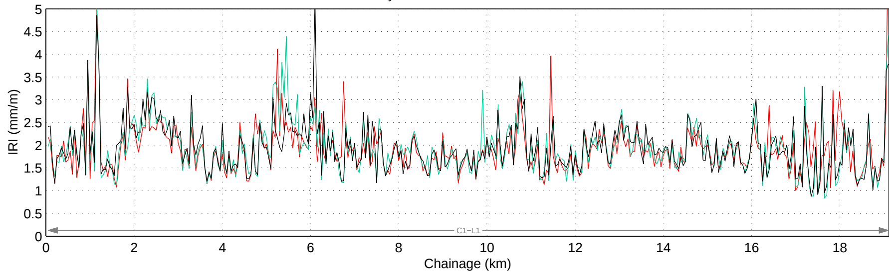
Hwy 556:02 Mean IRI – Right Lane
