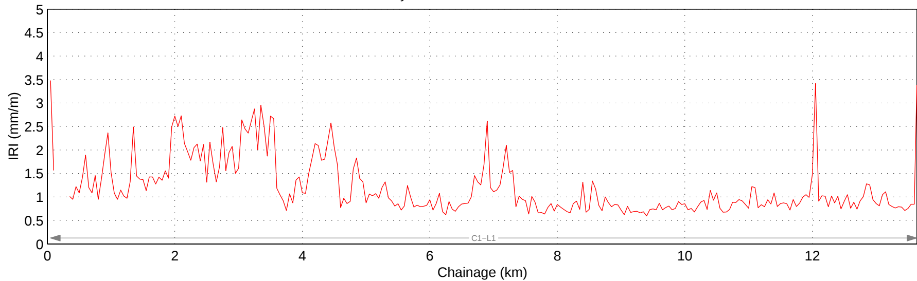
Hwy 562:02 Mean IRI – Right Lane
