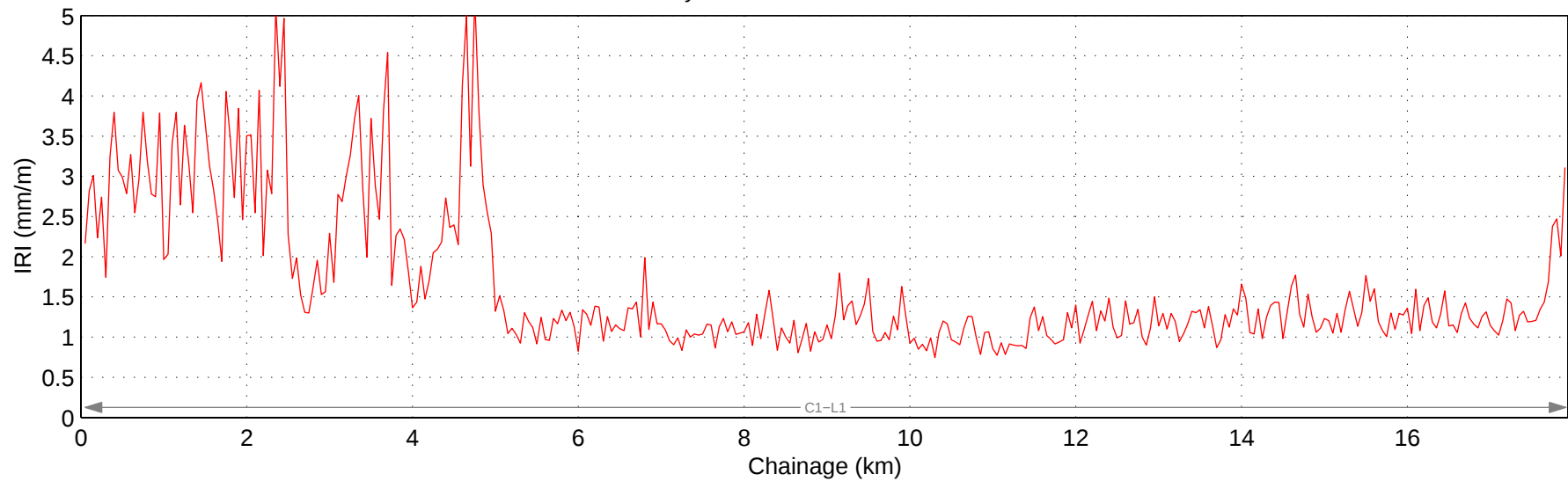
Hwy 531:02 Mean IRI – Right Lane
