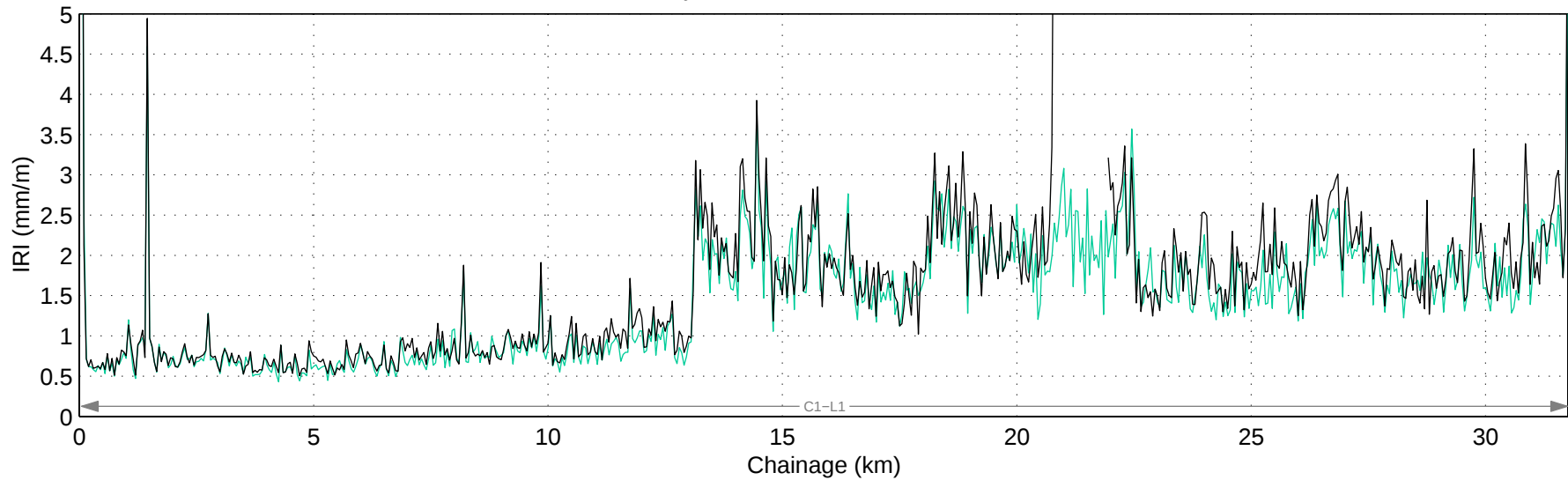
Hwy 519:02 Mean IRI – Right Lane
