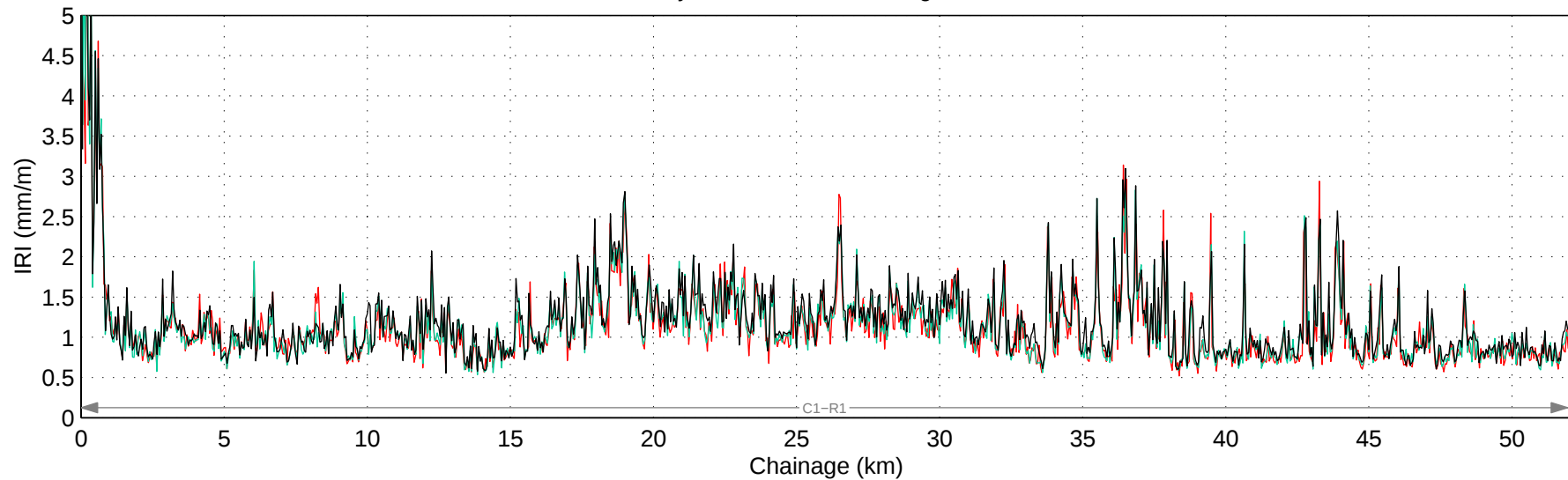
Hwy 501:06 Mean IRI – Right Lane
