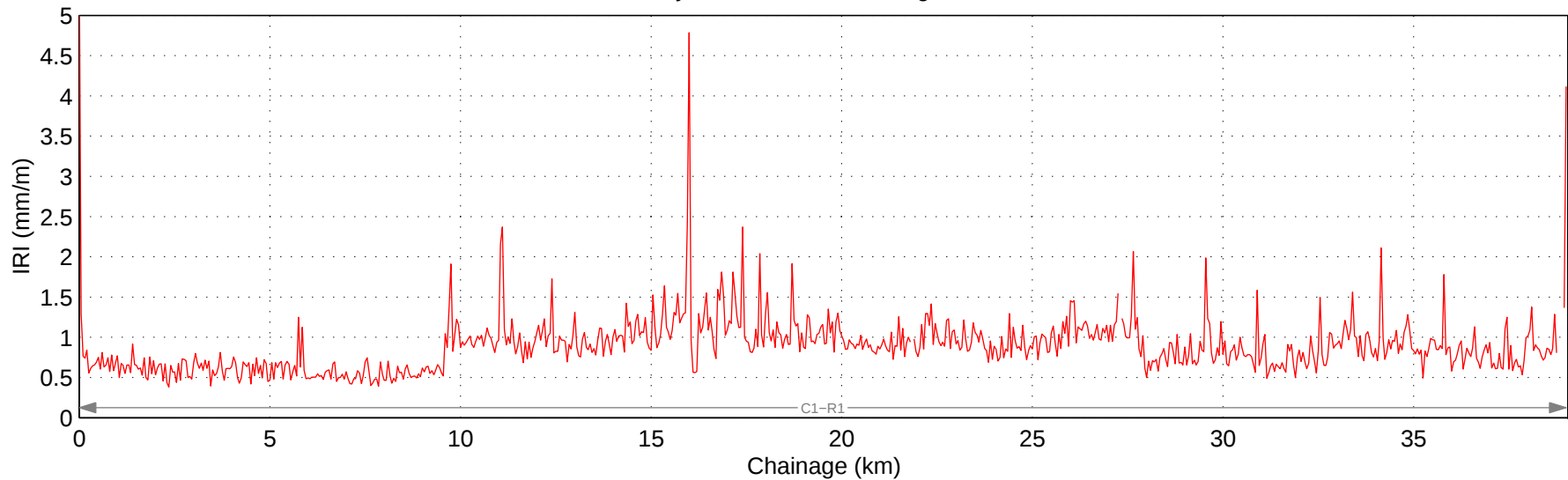
Hwy 526:02 Mean IRI – Right Lane
