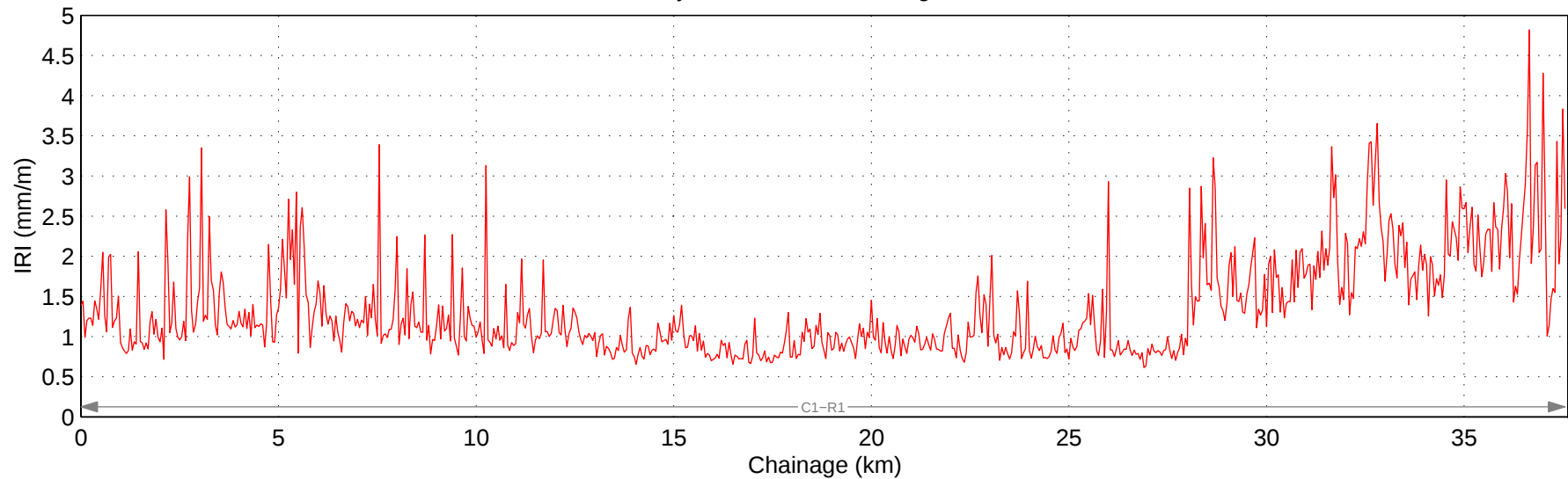
Hwy 533:02 Mean IRI – Right Lane
