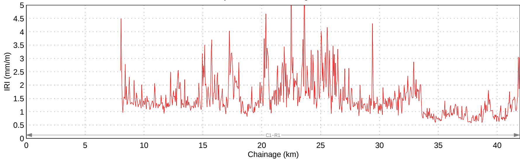
Hwy 584:02 Mean IRI – Right Lane
