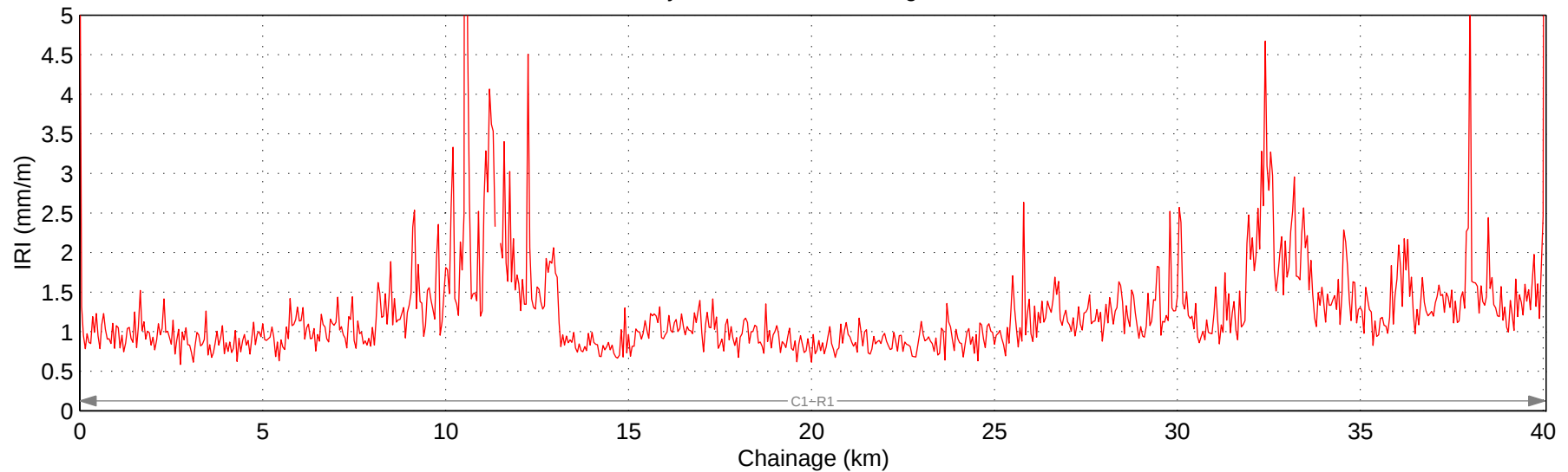
Hwy 567:04 Mean IRI – Right Lane
