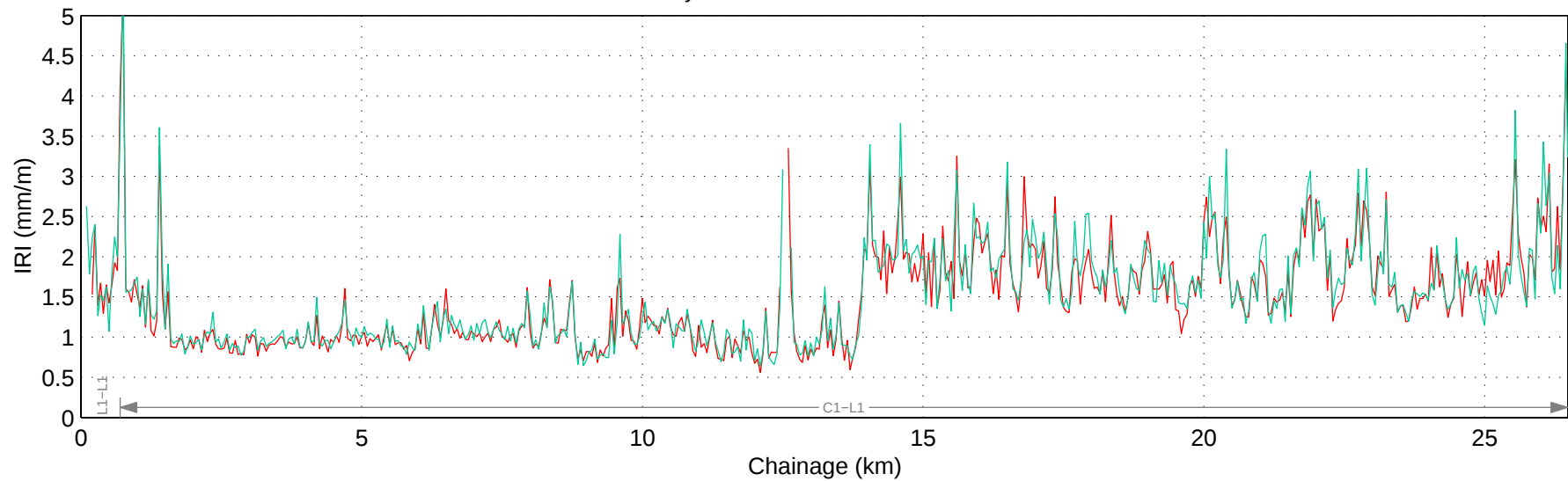
Hwy 552:02 Mean IRI – Right Lane
