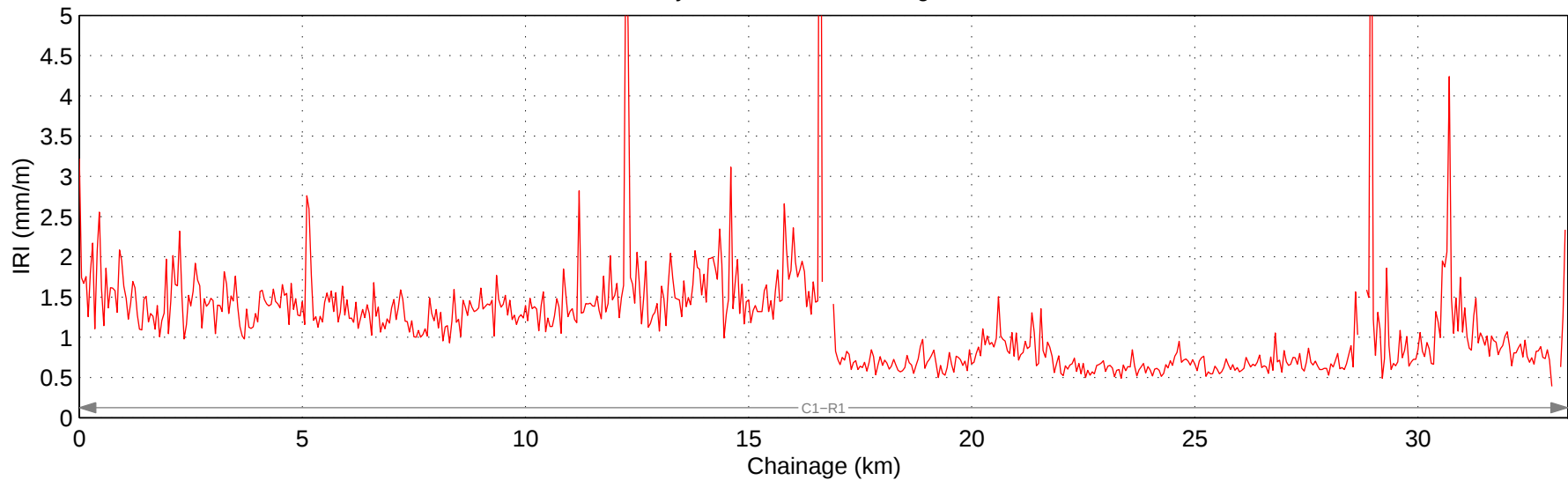
Hwy 547:04 Mean IRI – Right Lane
