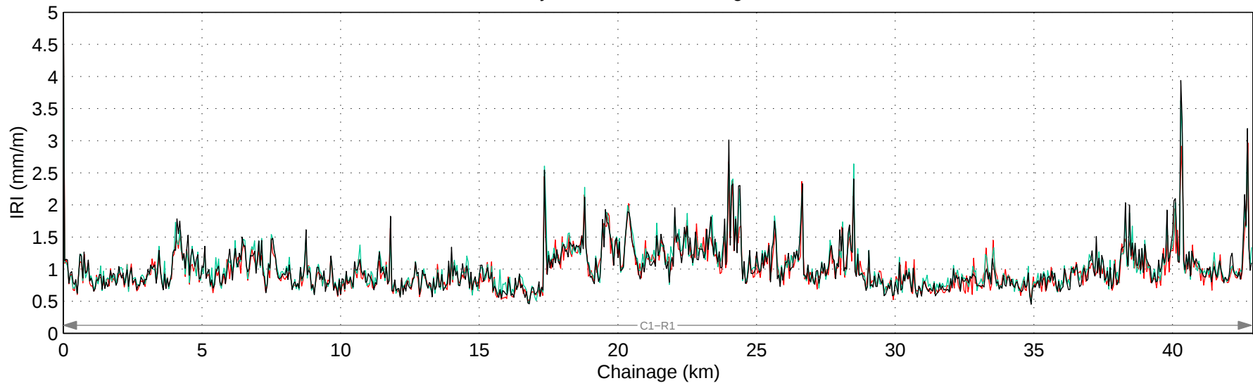
Hwy 555:02 Mean IRI – Right Lane
