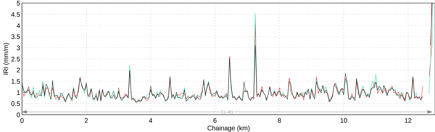
Hwy 552:01 Mean IRI – Right Lane
