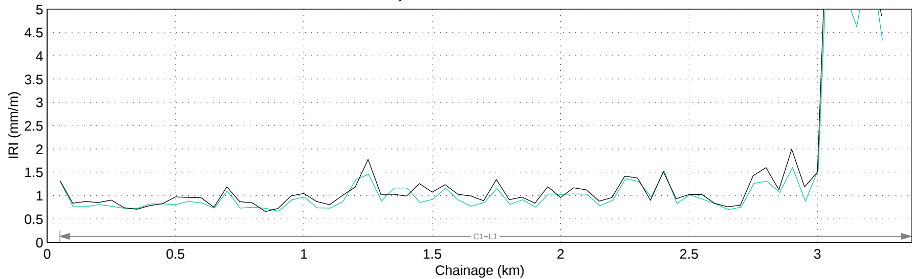
Hwy 580:04 Mean IRI – Right Lane
