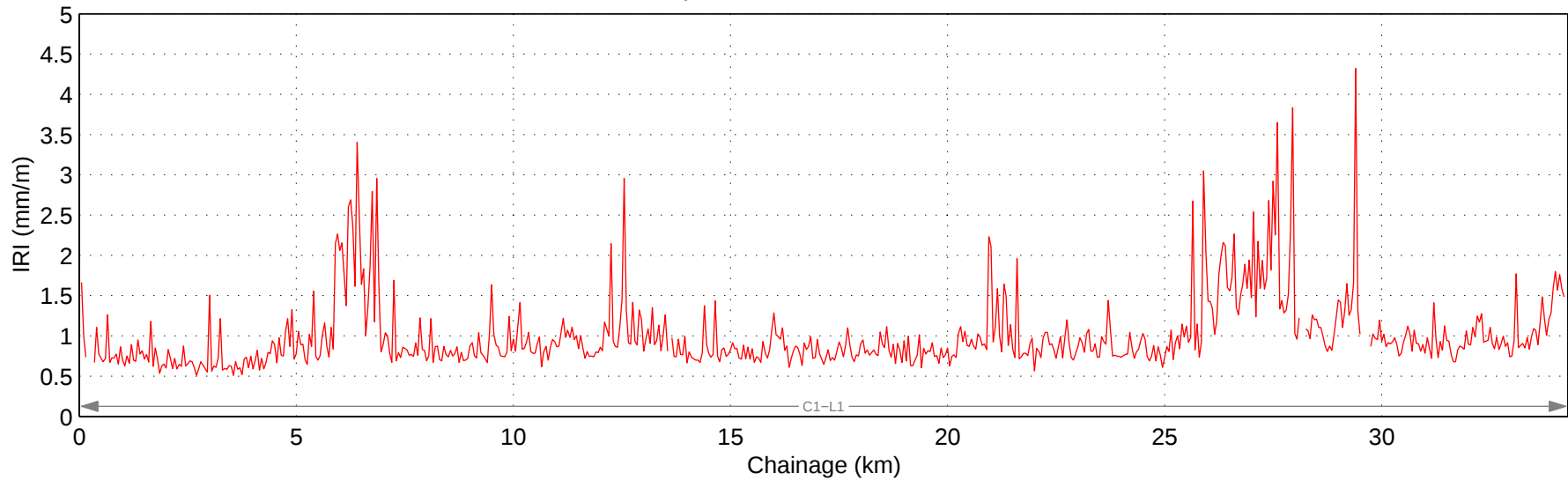
Hwy 582:02 Mean IRI – Right Lane
