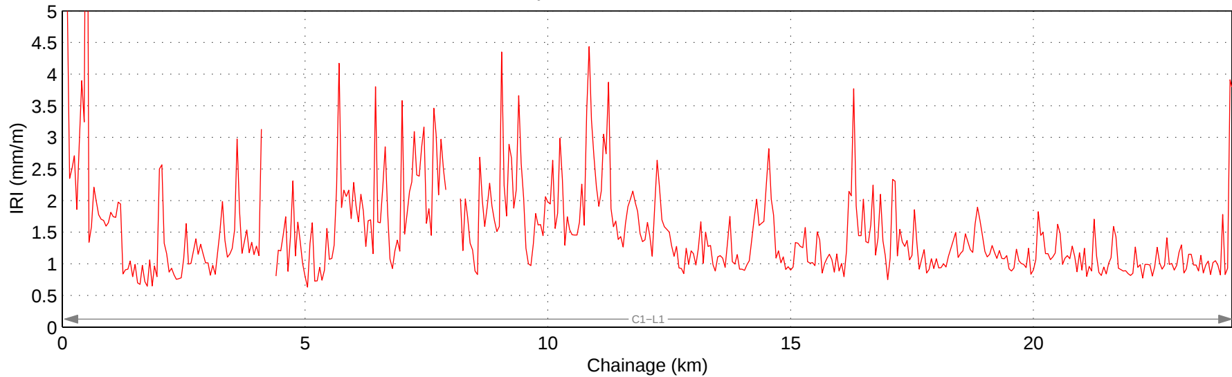
Hwy 510:02 Mean IRI – Right Lane
