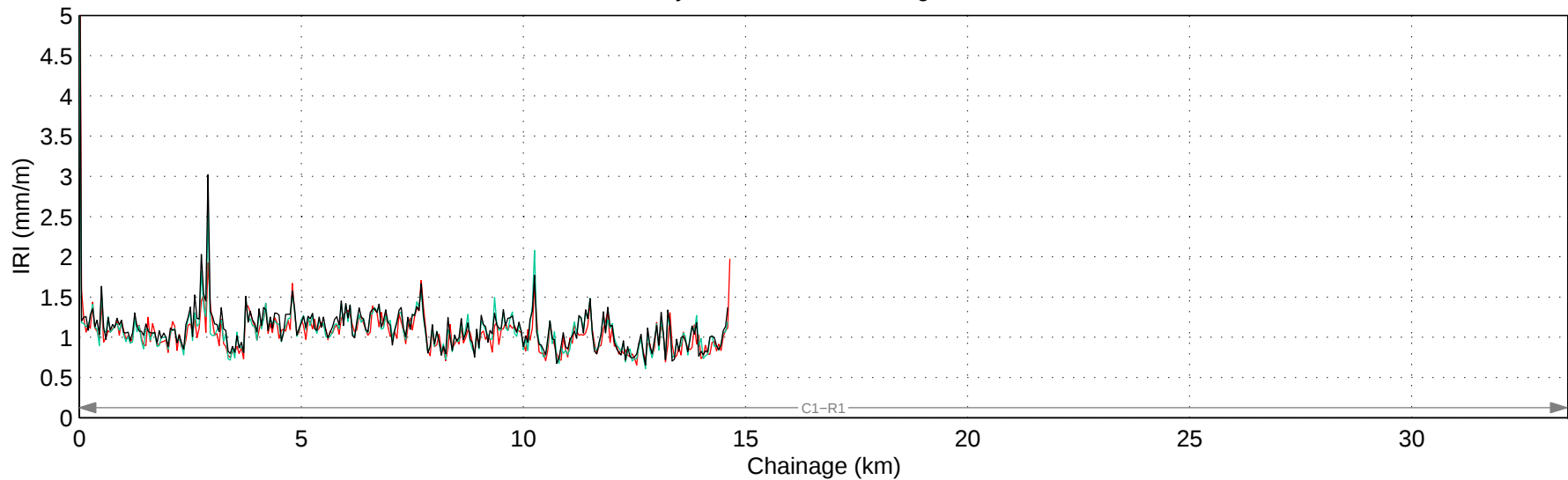
Hwy 564:10 Mean IRI – Right Lane
