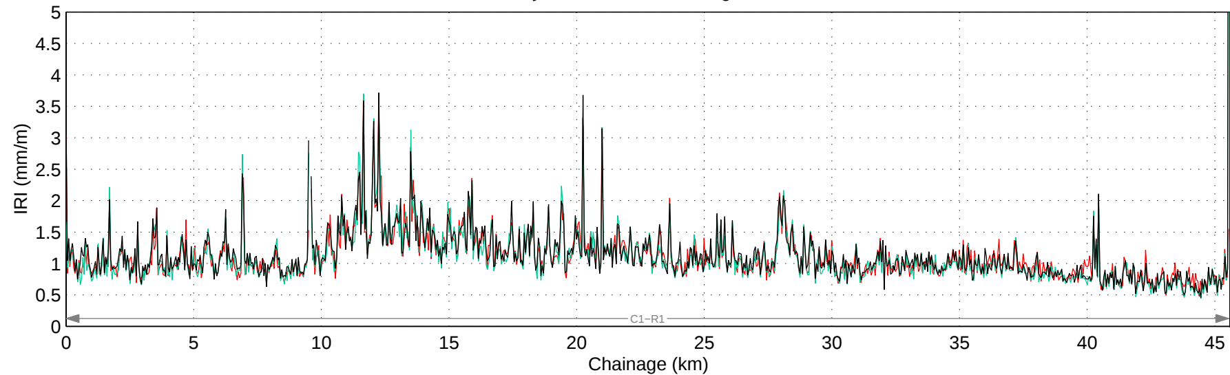
Hwy 501:02 Mean IRI – Right Lane
