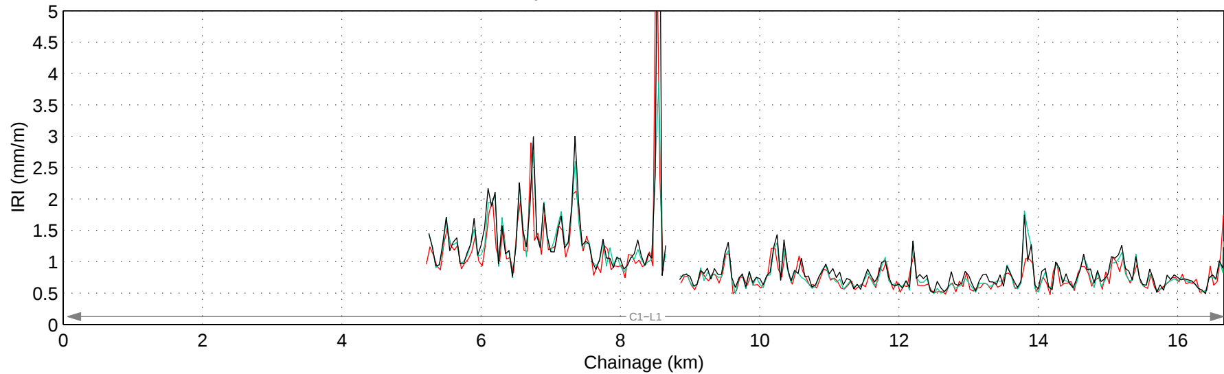
Hwy 535:02 Mean IRI – Right Lane
