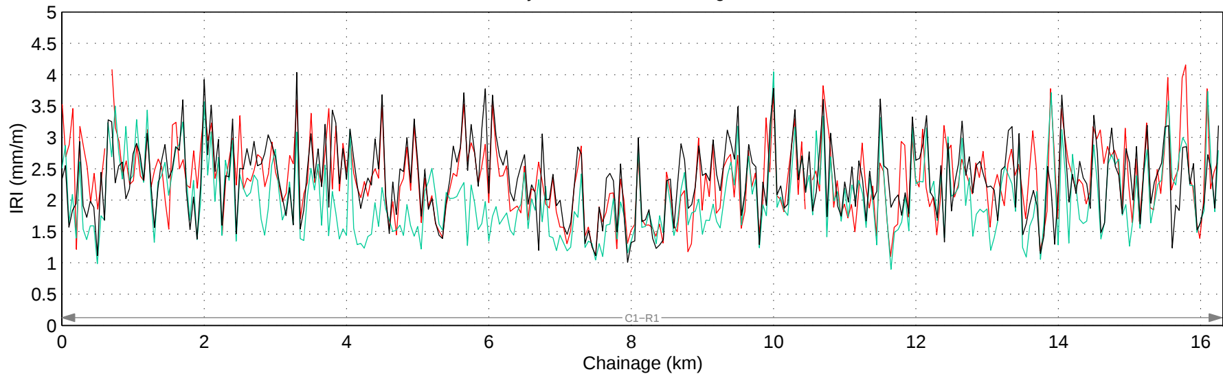
Hwy 560:02 Mean IRI – Right Lane
