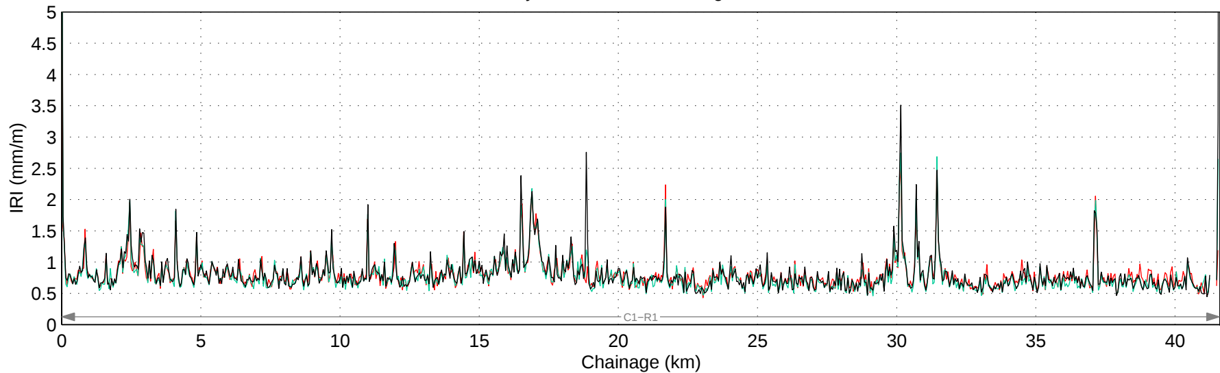
Hwy 599:06 Mean IRI – Right Lane
