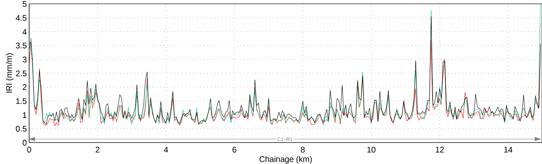
Hwy 587:03 Mean IRI – Right Lane
