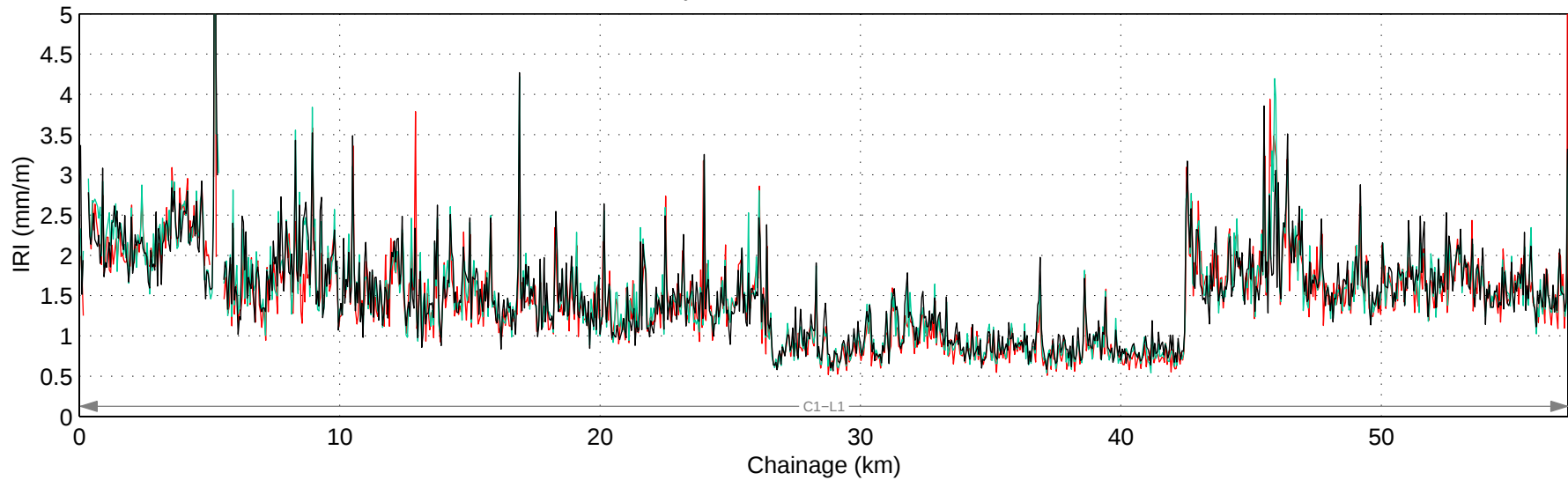
Hwy 544:02 Mean IRI – Right Lane
