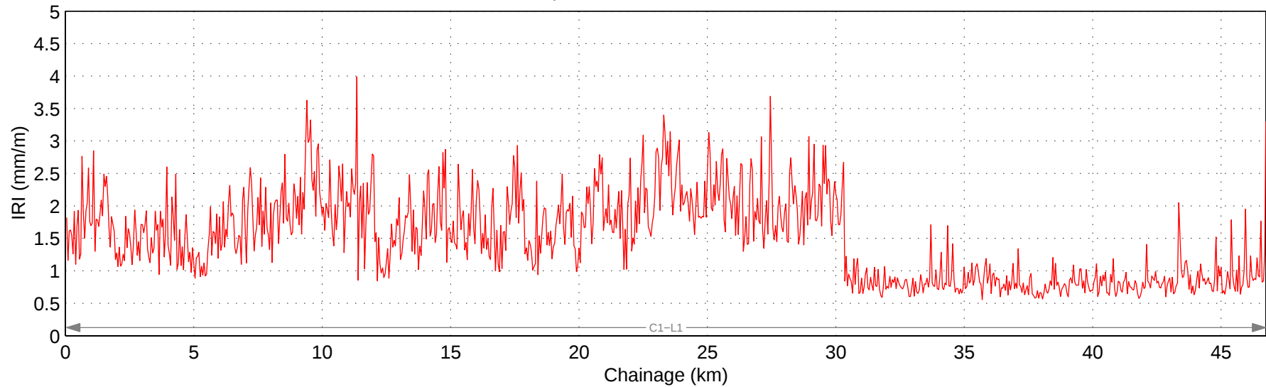
Hwy 590:02 Mean IRI – Right Lane
