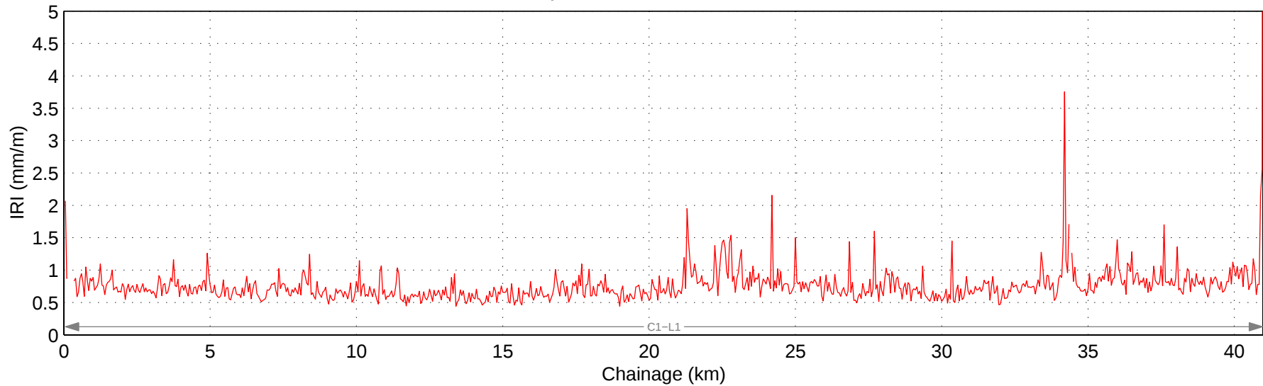
Hwy 575:02 Mean IRI – Right Lane
