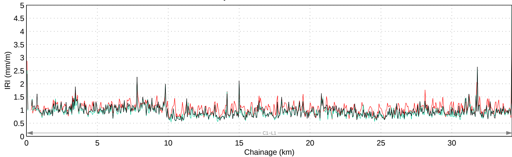
Hwy 513:02 Mean IRI – Right Lane
