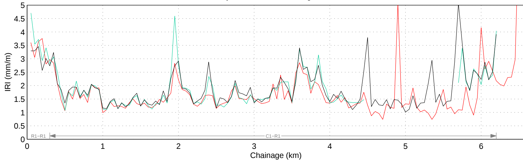
Hwy 563:02 Mean IRI – Right Lane
