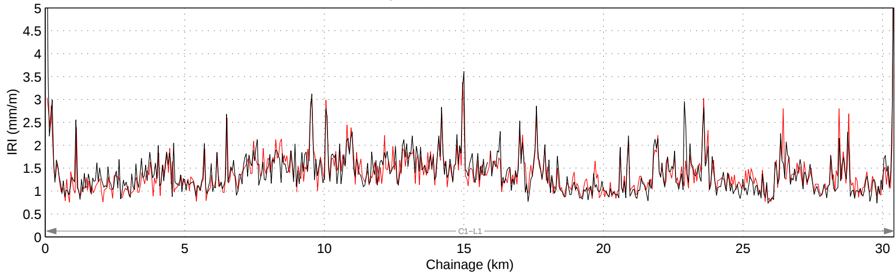
Hwy 561:02 Mean IRI – Right Lane
