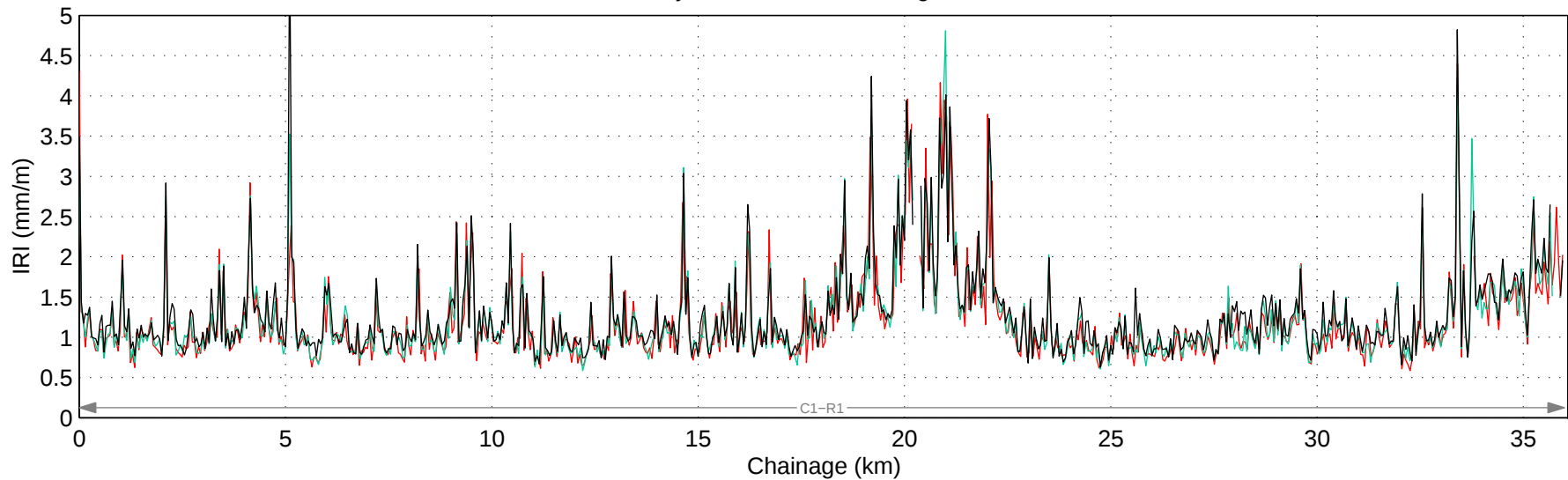
Hwy 590:04 Mean IRI – Right Lane
