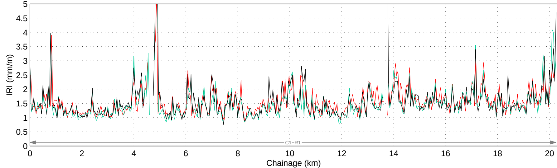
Hwy 592:02 Mean IRI – Right Lane
