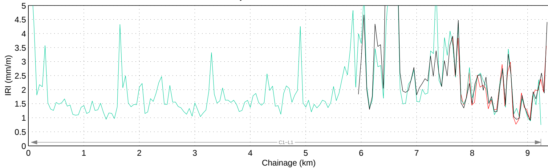
Hwy 524:02 Mean IRI – Right Lane
