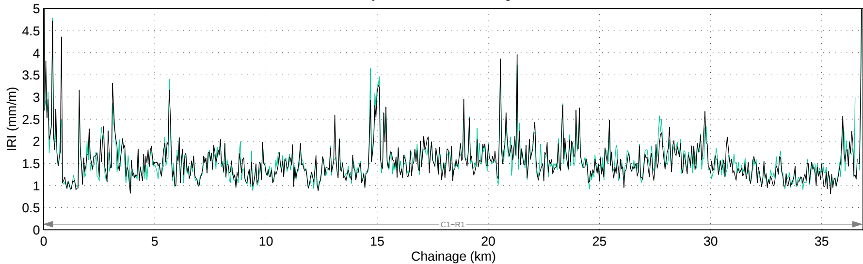
Hwy 507:04 Mean IRI – Right Lane
