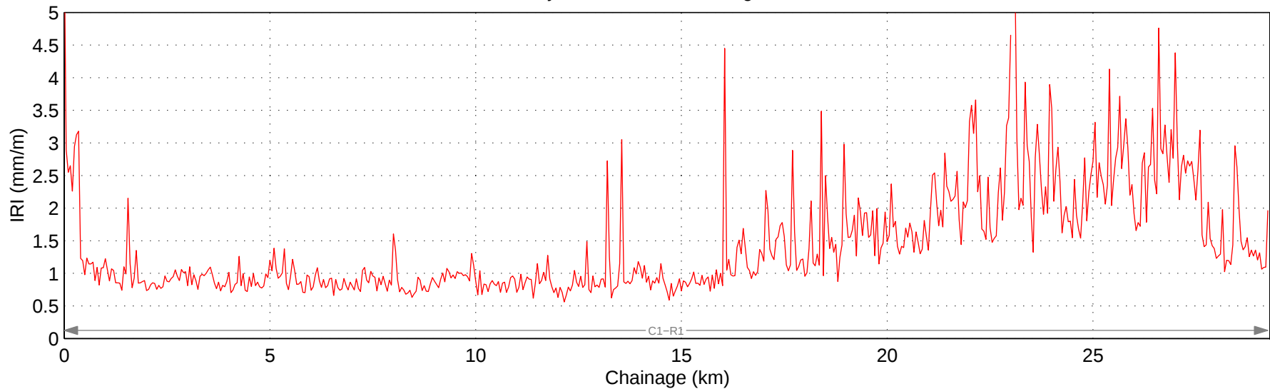
Hwy 542:02 Mean IRI – Right Lane
