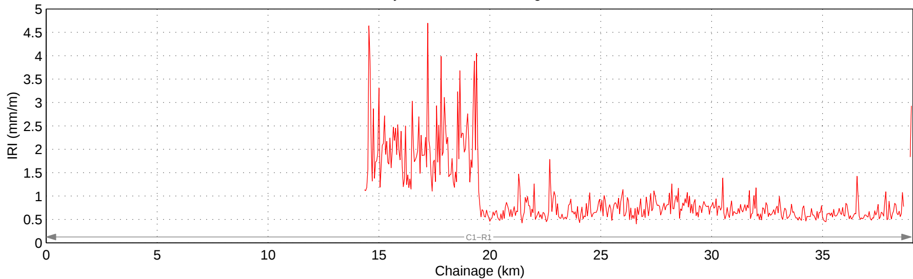
Hwy 587:04 Mean IRI – Right Lane
