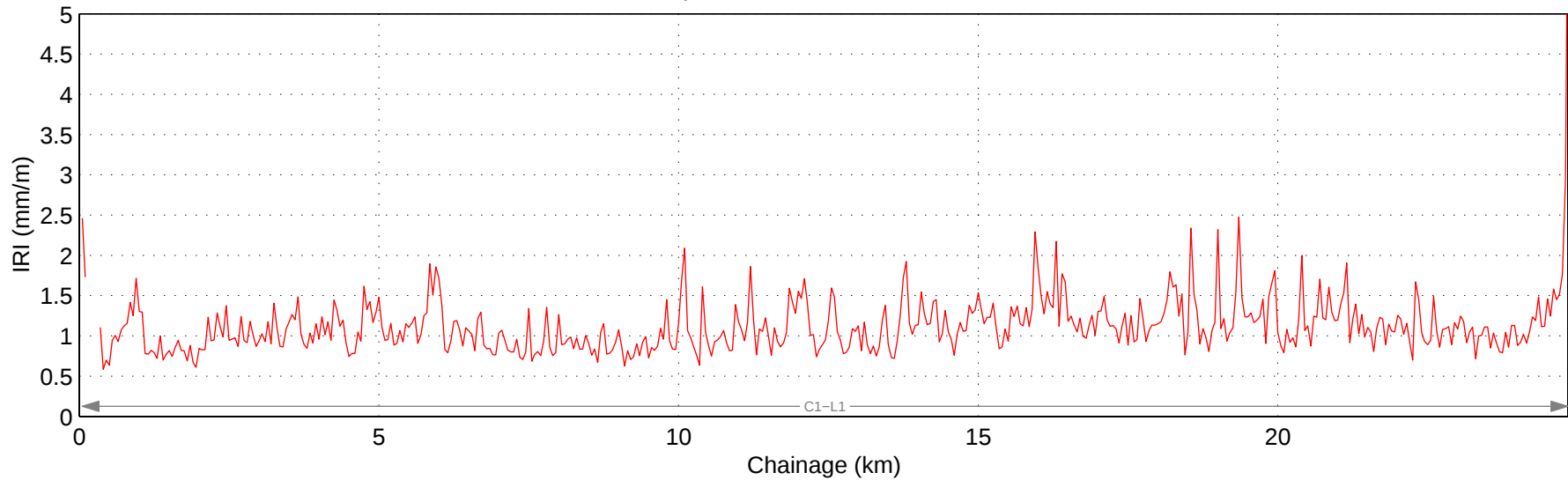
Hwy 543:02 Mean IRI – Right Lane
