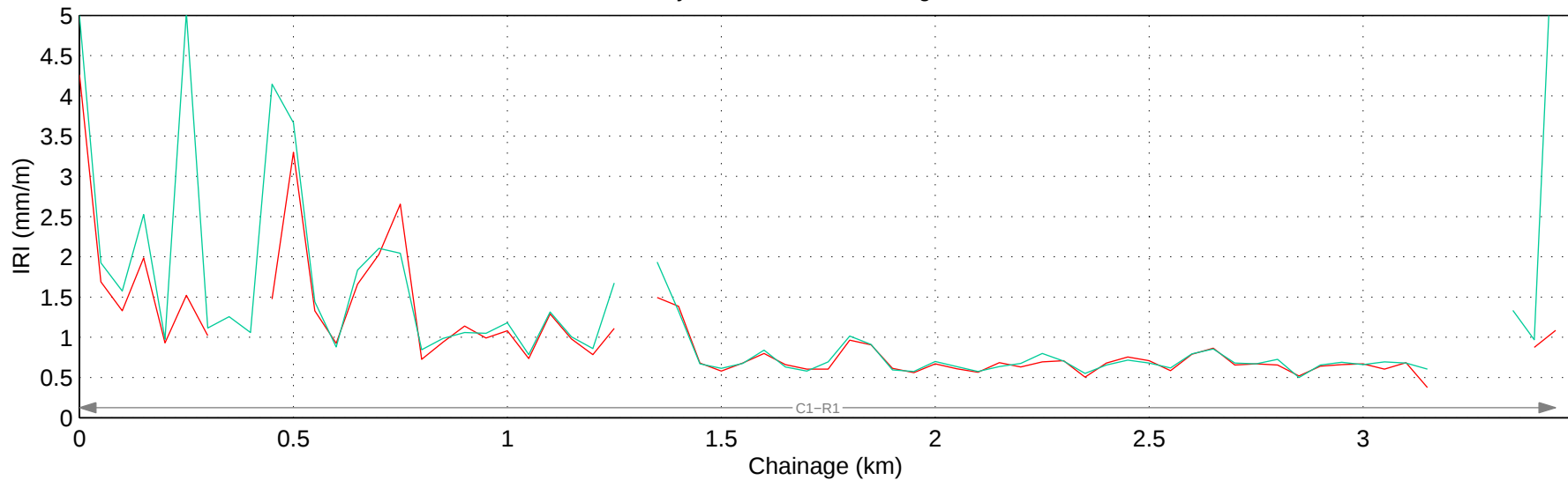
Hwy 599:02 Mean IRI – Right Lane
