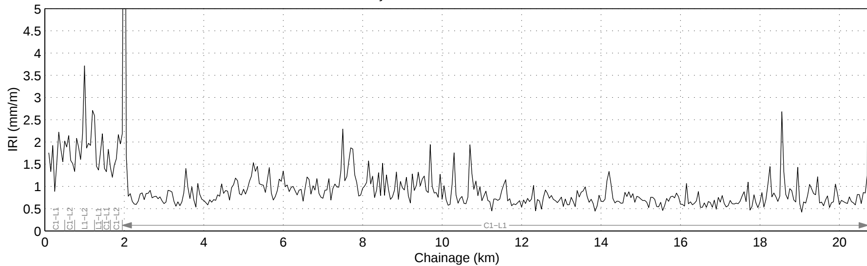
Hwy 597:02 Mean IRI – Right Lane
