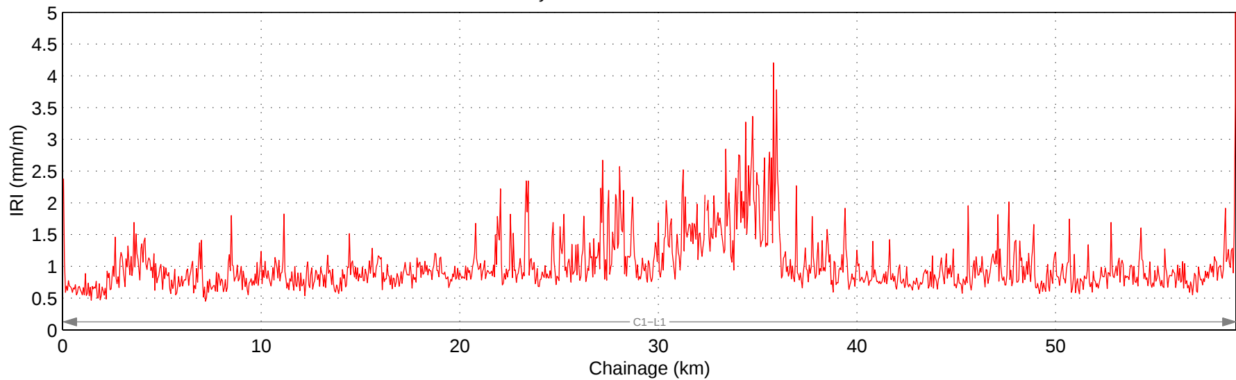
Hwy 501:04 Mean IRI – Right Lane
