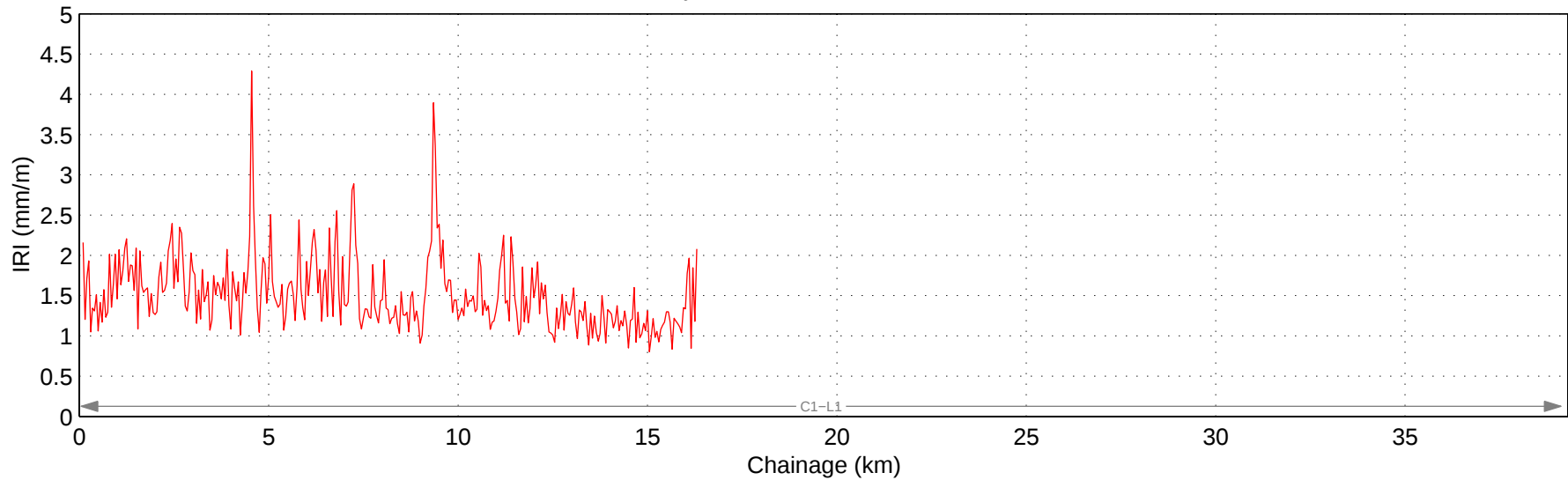
Hwy 529:04 Mean IRI – Right Lane
