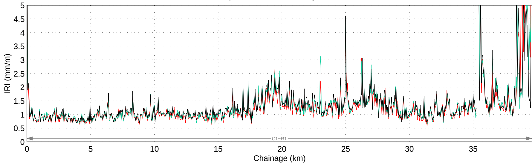
Hwy 550:02 Mean IRI – Right Lane
