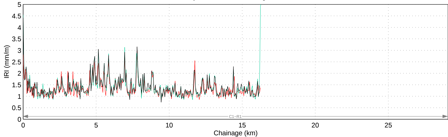
Hwy 504:02 Mean IRI – Right Lane
