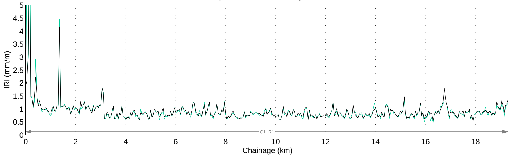
Hwy 533:04 Mean IRI – Right Lane
