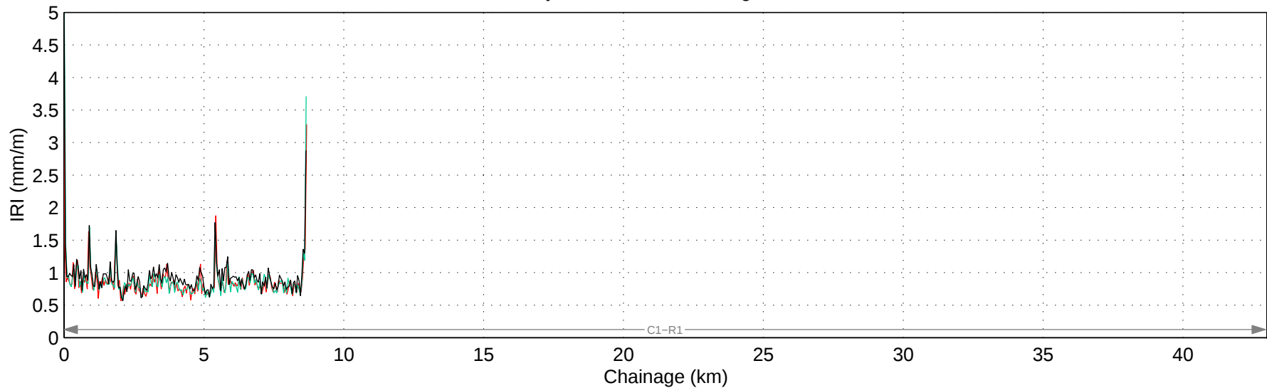
Hwy 500:04 Mean IRI – Right Lane
