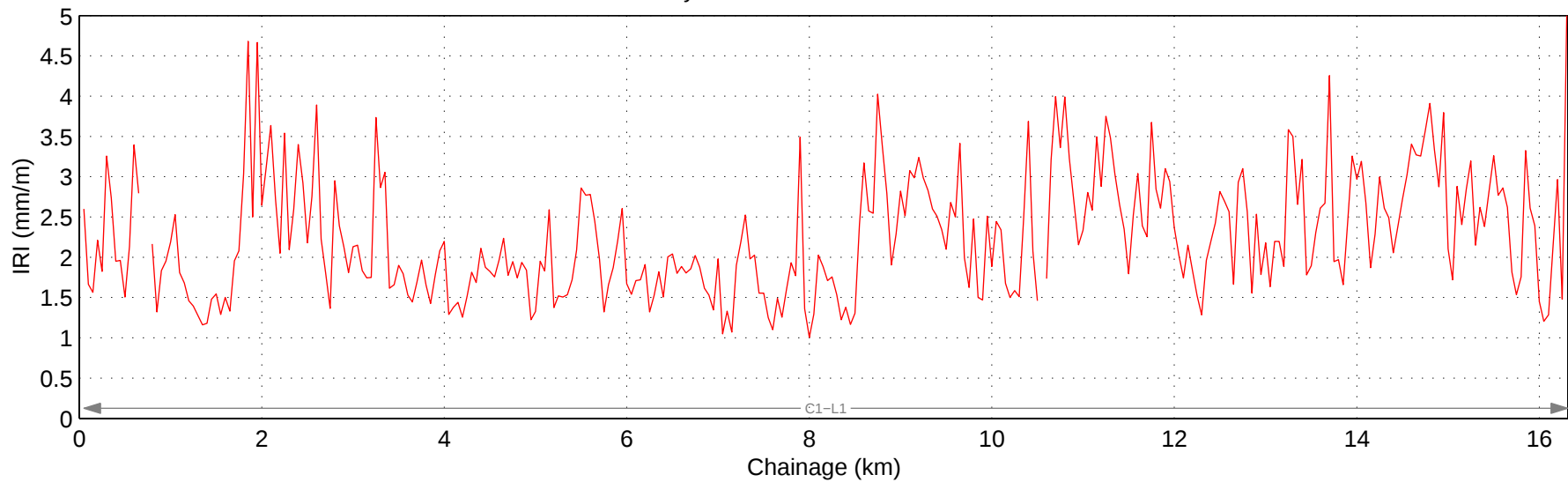
Hwy 560:02 Mean IRI – Right Lane
