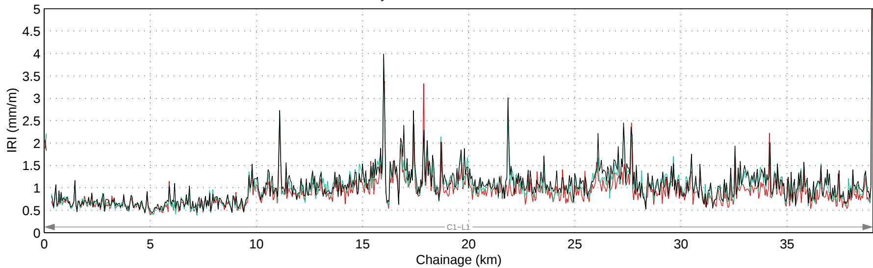
Hwy 526:02 Mean IRI – Right Lane
