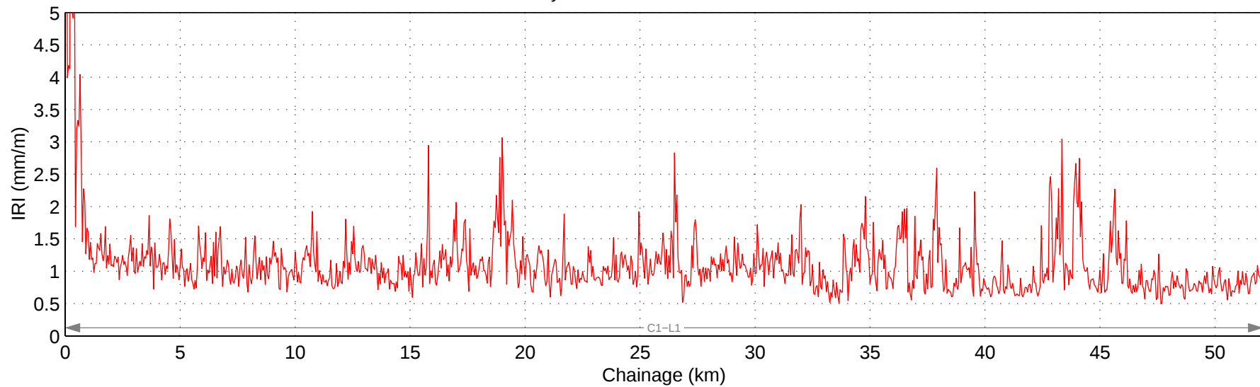
Hwy 501:06 Mean IRI – Right Lane
