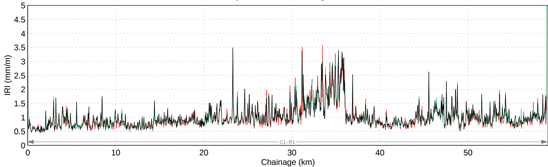
Hwy 501:04 Mean IRI – Right Lane
