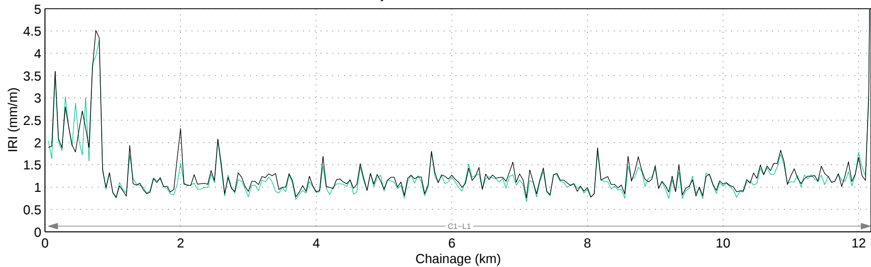
Hwy 519:06 Mean IRI – Right Lane
