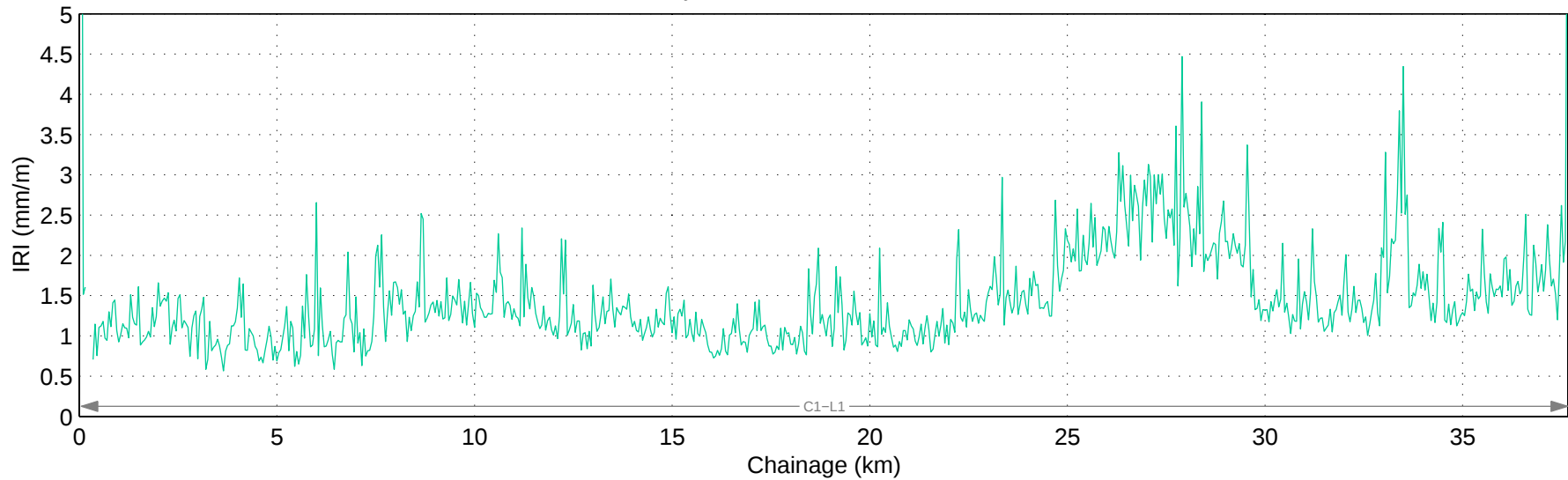
Hwy 529:02 Mean IRI – Right Lane
