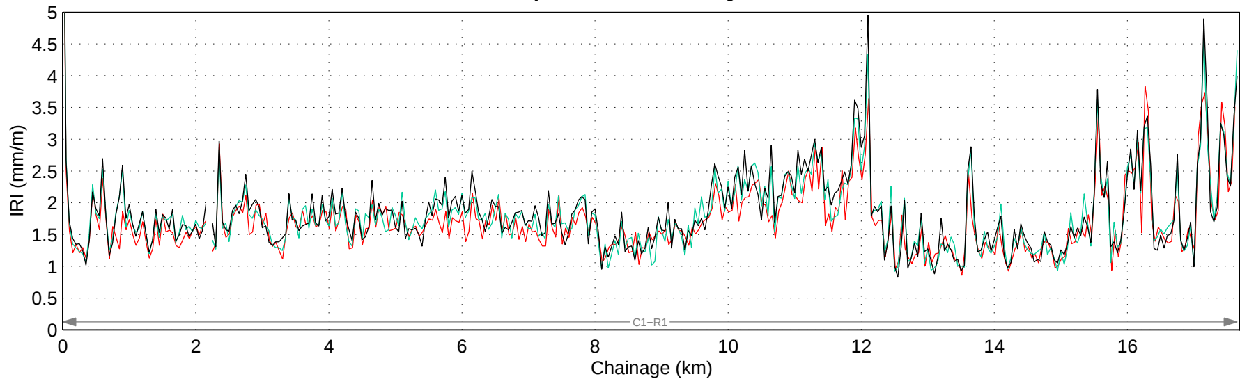
Hwy 519:04 Mean IRI – Right Lane
