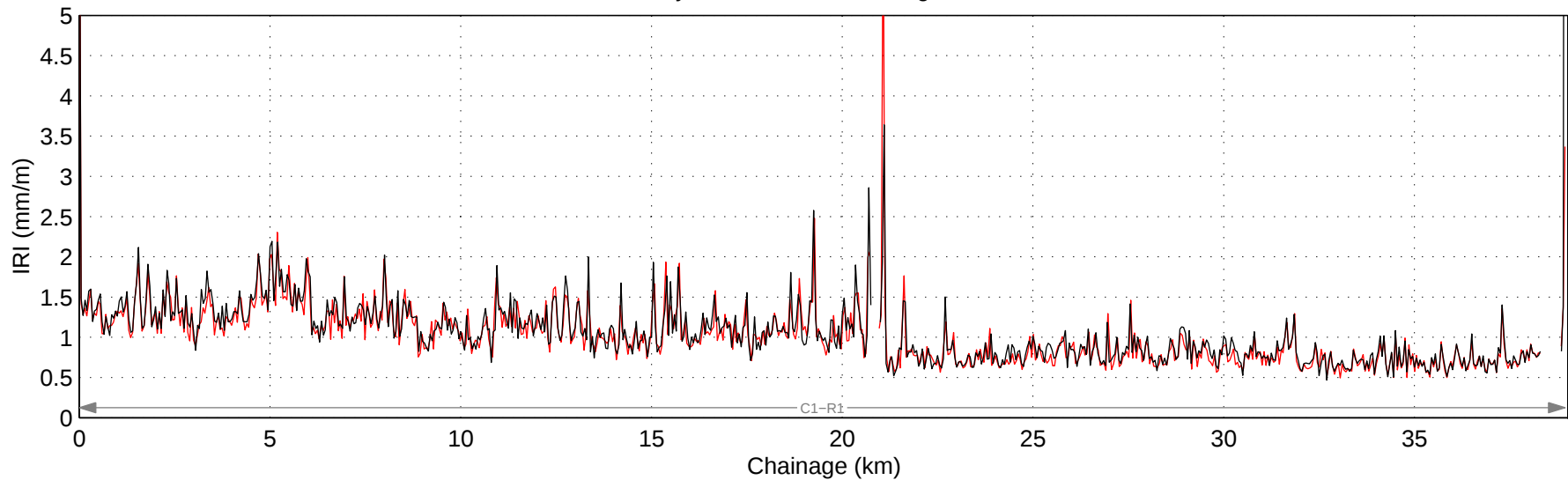
Hwy 570:08 Mean IRI – Right Lane
