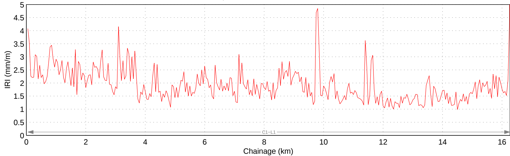
Hwy 564:04 Mean IRI – Right Lane
