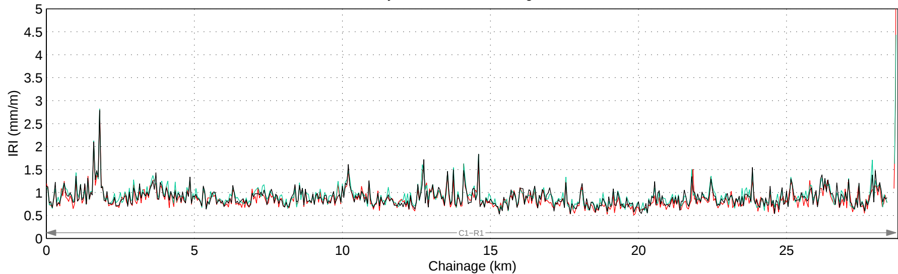
Hwy 570:04 Mean IRI – Right Lane
