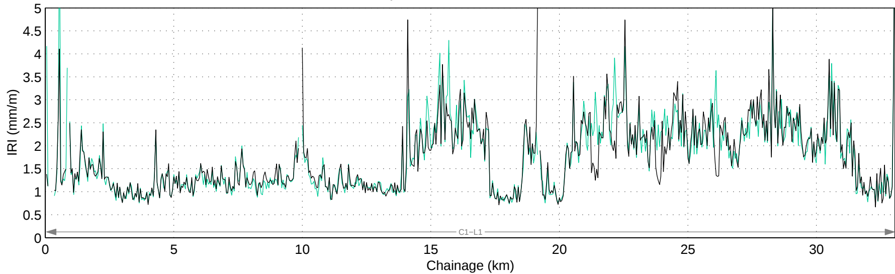
Hwy 507:02 Mean IRI – Right Lane
