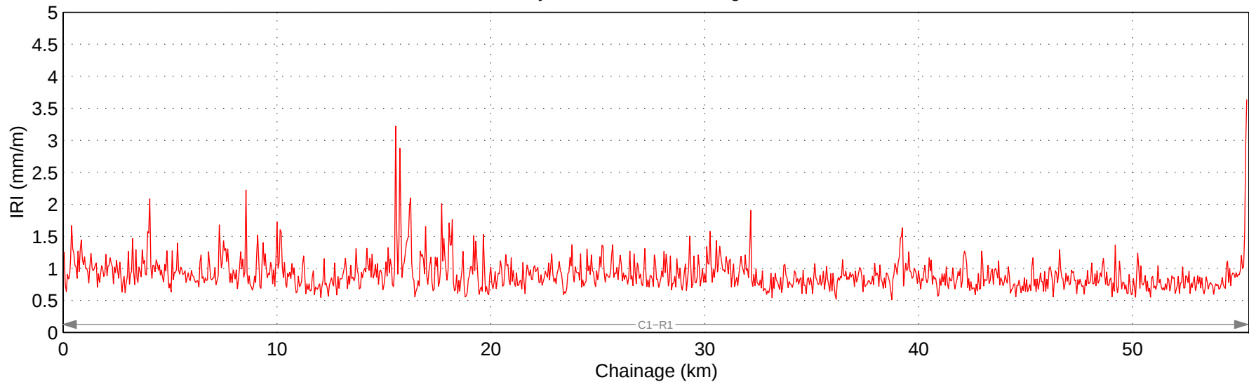
Hwy 524:06 Mean IRI – Right Lane
