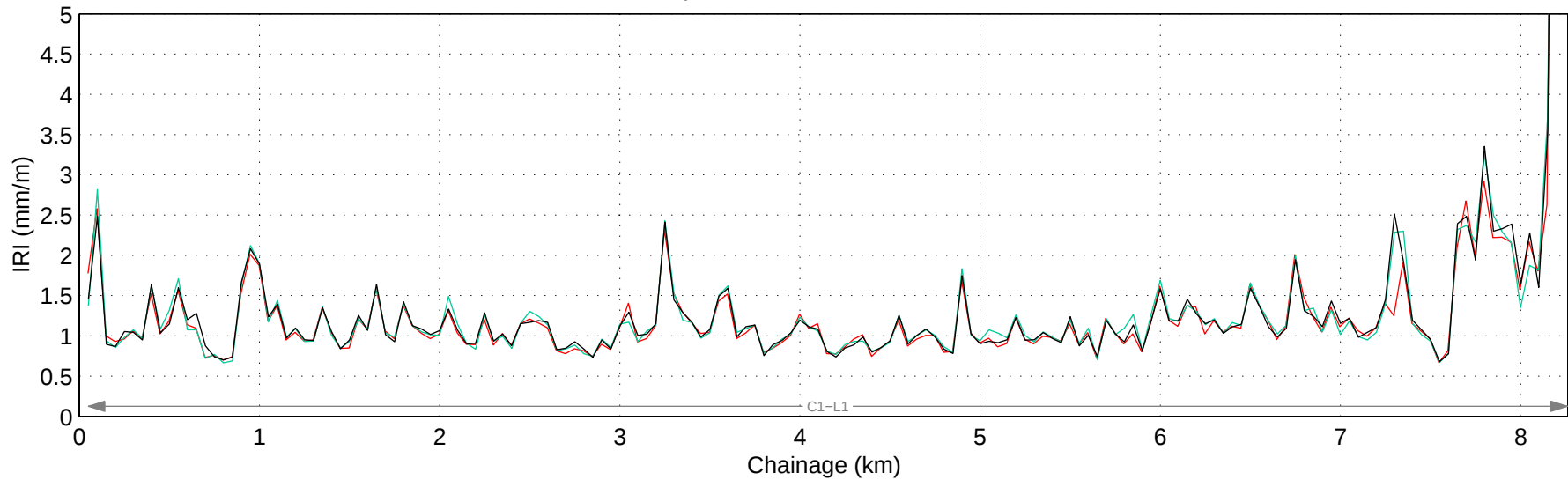
Hwy 508:02 Mean IRI – Right Lane
