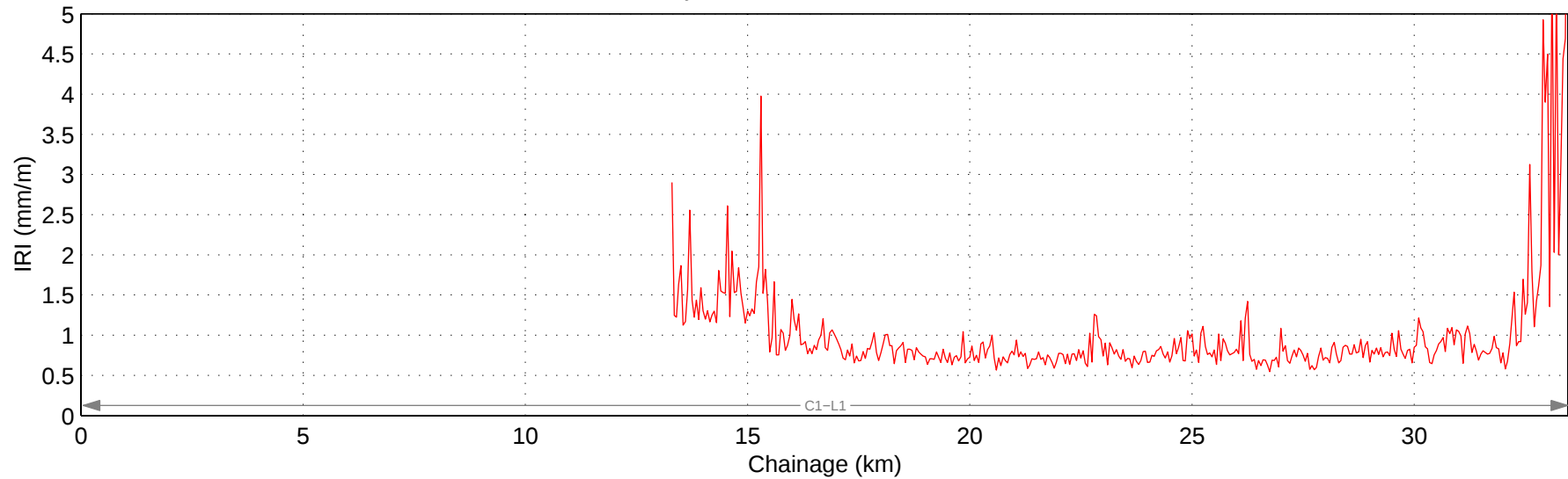
Hwy 574:02 Mean IRI – Right Lane
