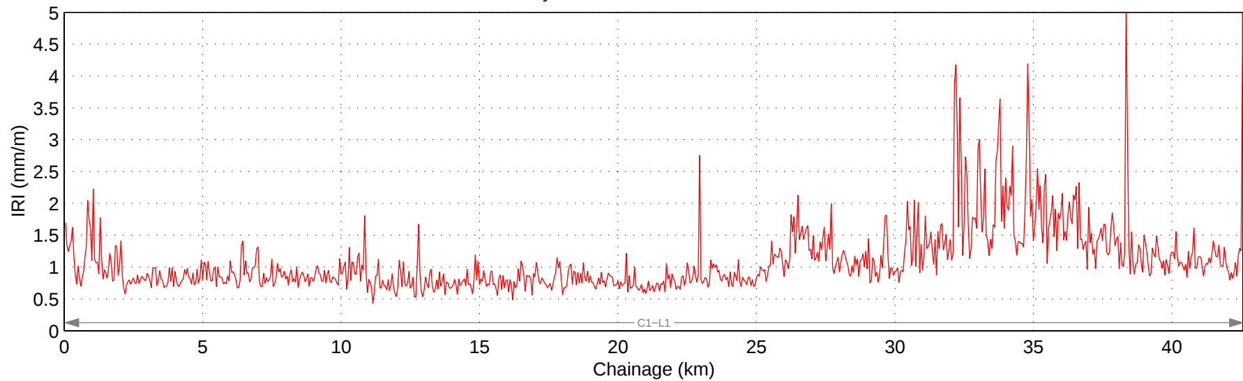
Hwy 555:04 Mean IRI – Right Lane
