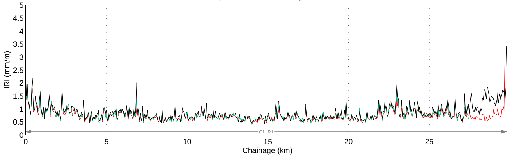
Hwy 539:02 Mean IRI – Right Lane
