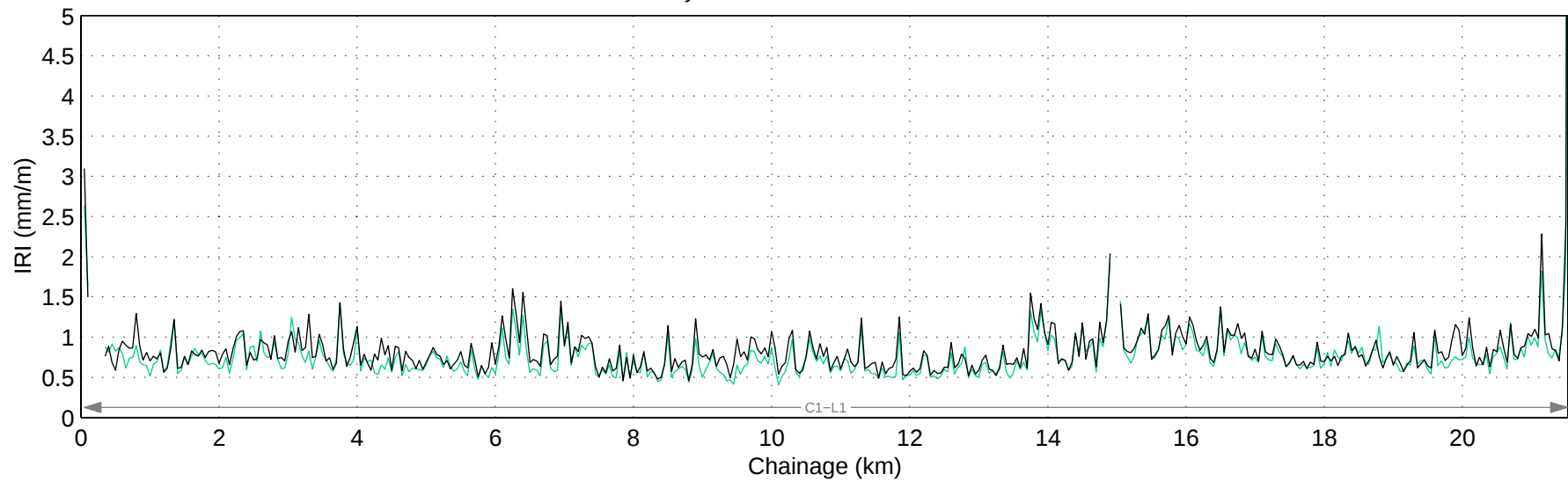
Hwy 505:04 Mean IRI – Right Lane
