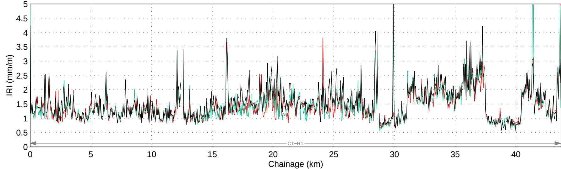
Hwy 587:02 Mean IRI – Right Lane
