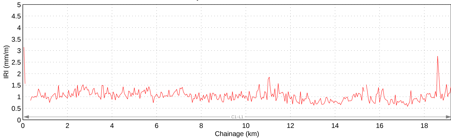
Hwy 570:02 Mean IRI – Right Lane
