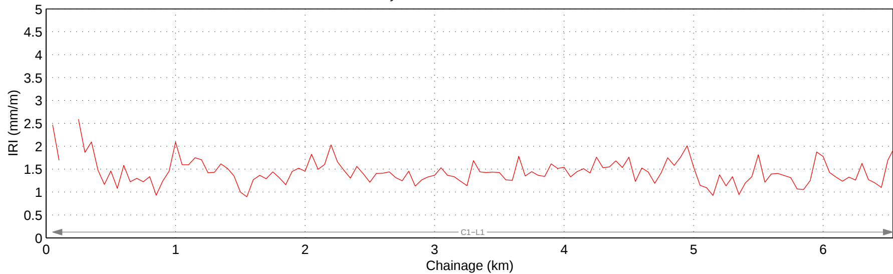
Hwy 545:02 Mean IRI – Right Lane
