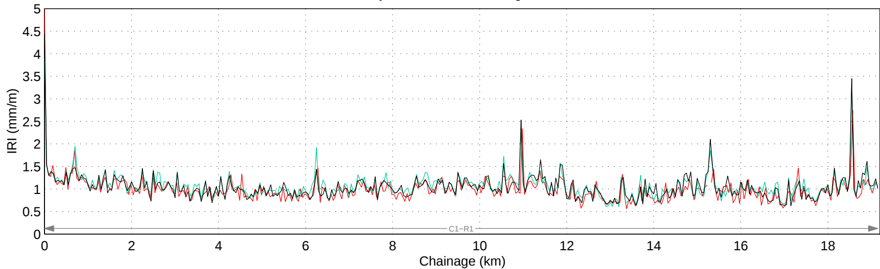
Hwy 570:02 Mean IRI – Right Lane
