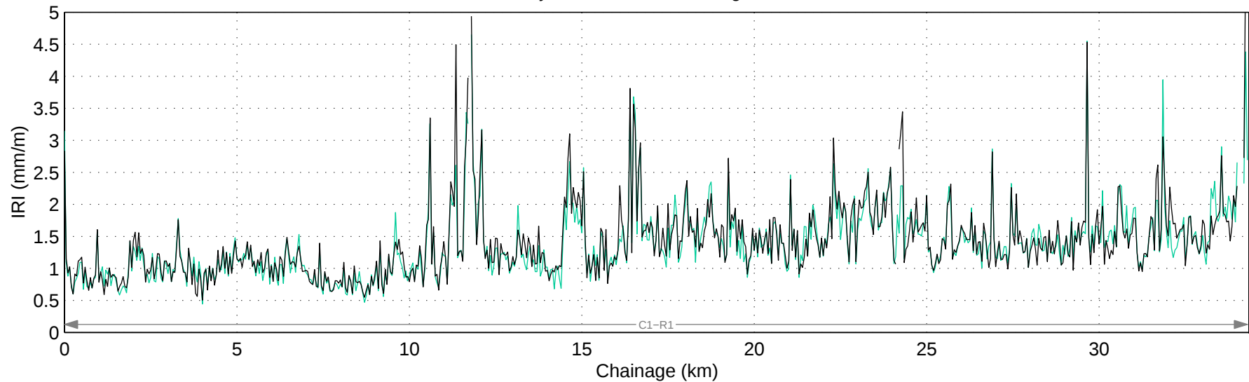
Hwy 566:02 Mean IRI – Right Lane
