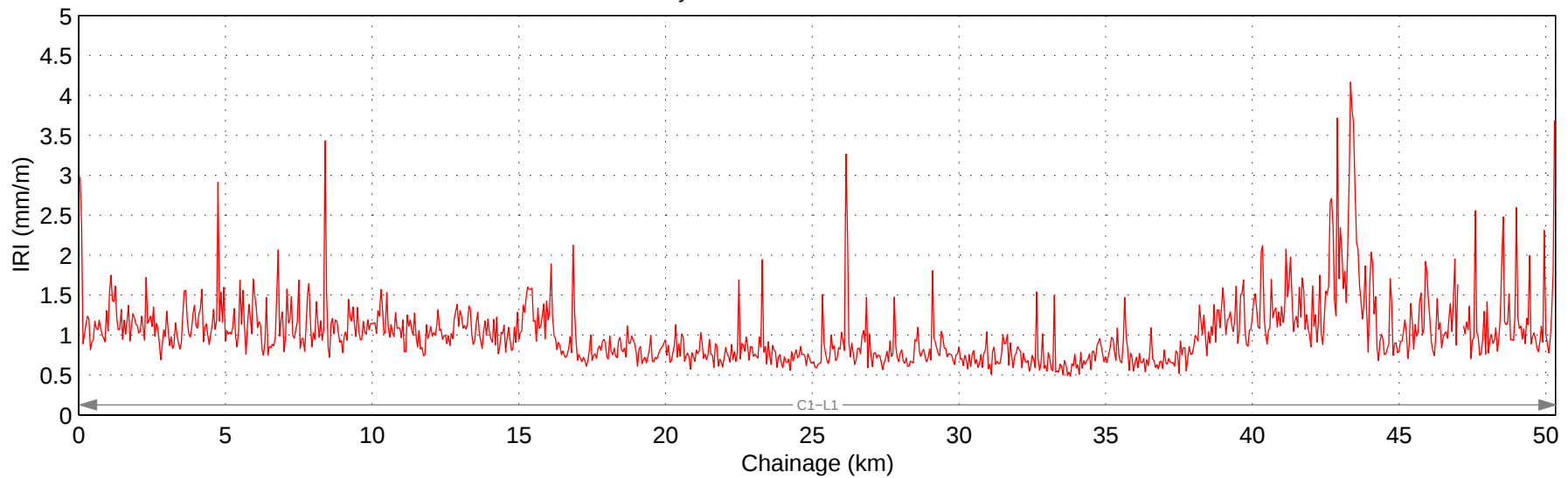
Hwy 509:02 Mean IRI – Right Lane
