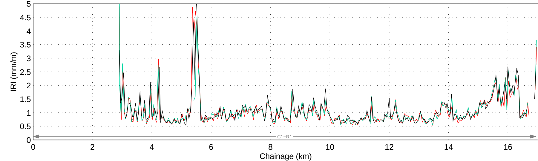
Hwy 549:02 Mean IRI – Right Lane
