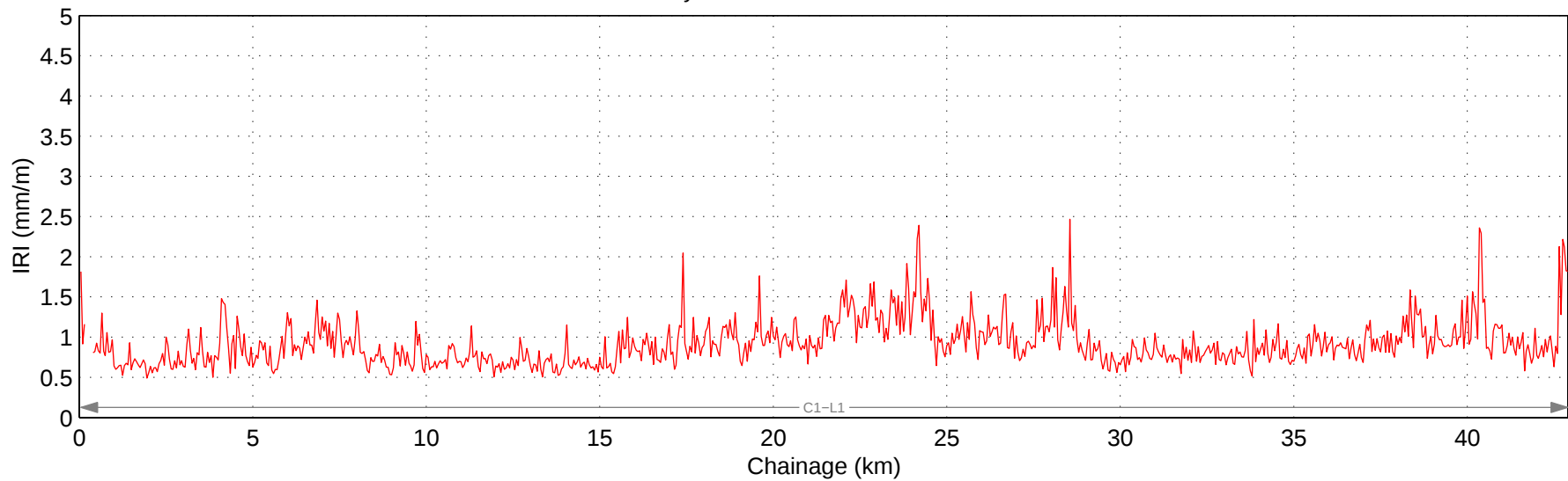
Hwy 555:02 Mean IRI – Right Lane
