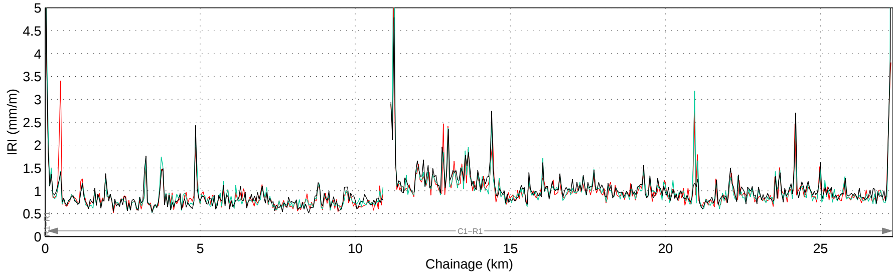
Hwy 512:02 Mean IRI – Right Lane
