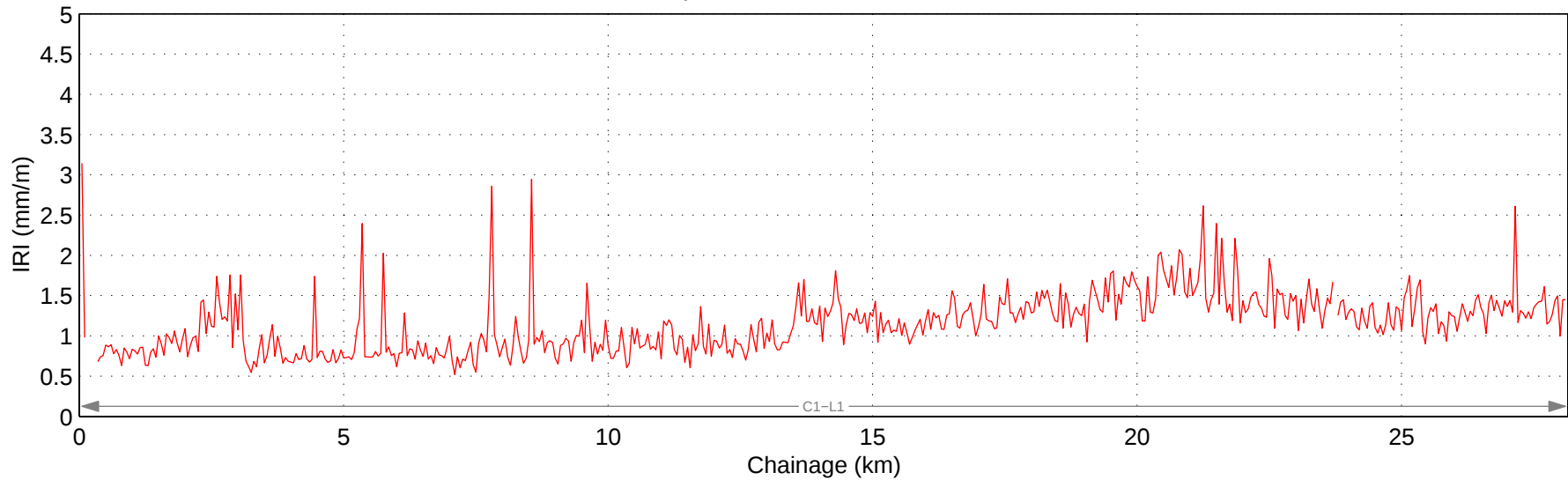
Hwy 599:04 Mean IRI – Right Lane
