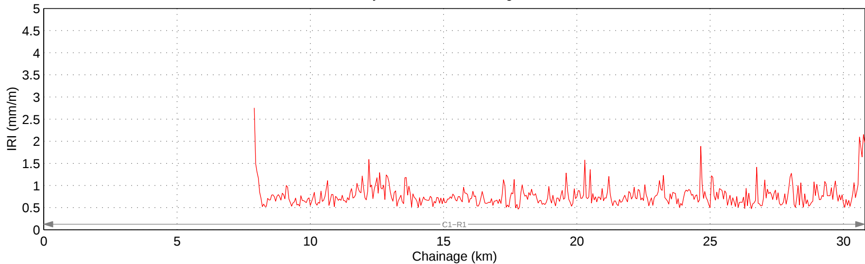
Hwy 591:02 Mean IRI – Right Lane
