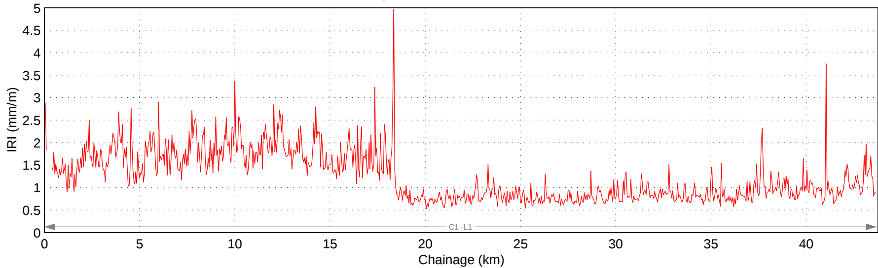
Hwy 534:02 Mean IRI – Right Lane
