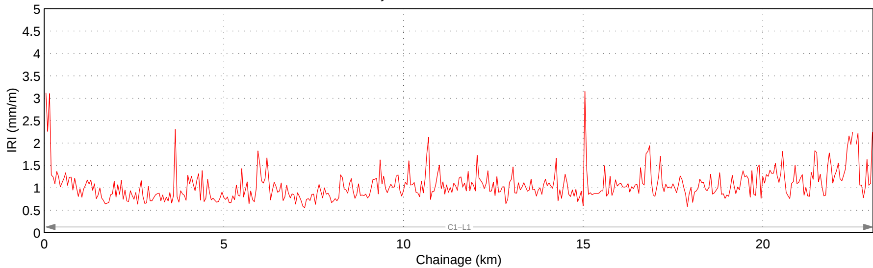
Hwy 598:02 Mean IRI – Right Lane
