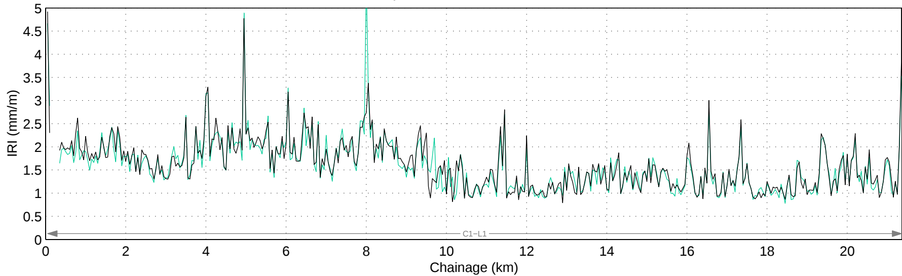
Hwy 567:02 Mean IRI – Right Lane
