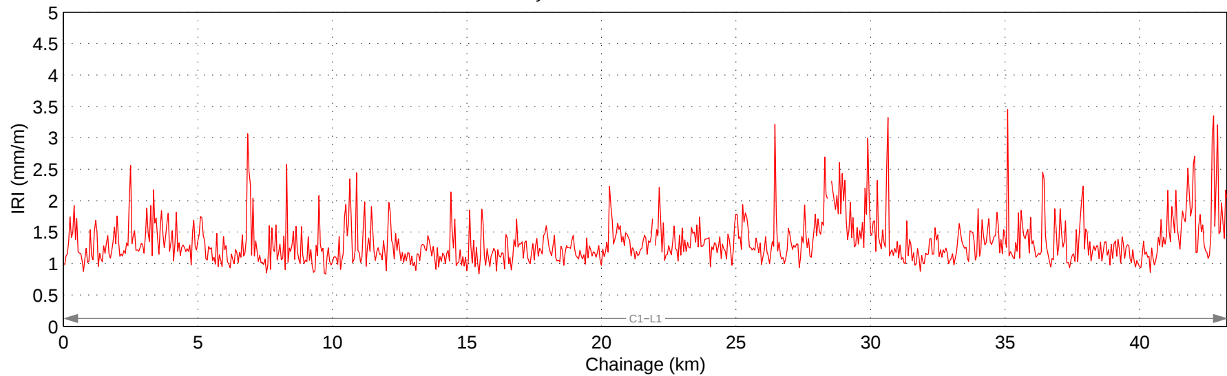
Hwy 541:02 Mean IRI – Right Lane
