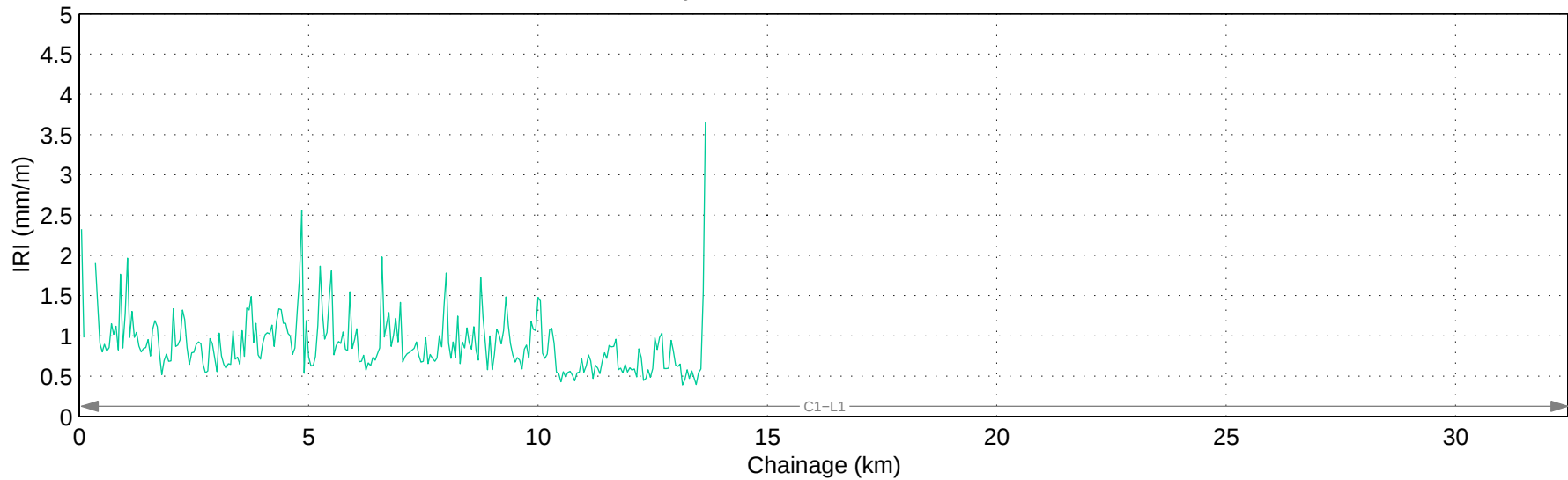
Hwy 540:02 Mean IRI – Right Lane
