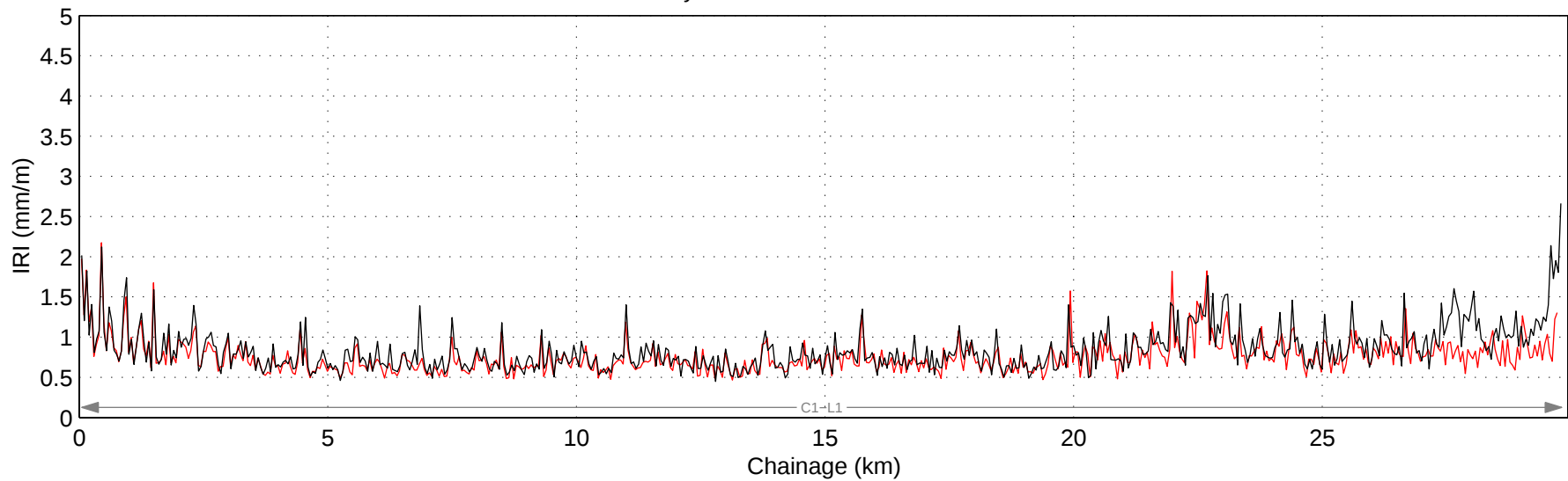
Hwy 539:02 Mean IRI – Right Lane
