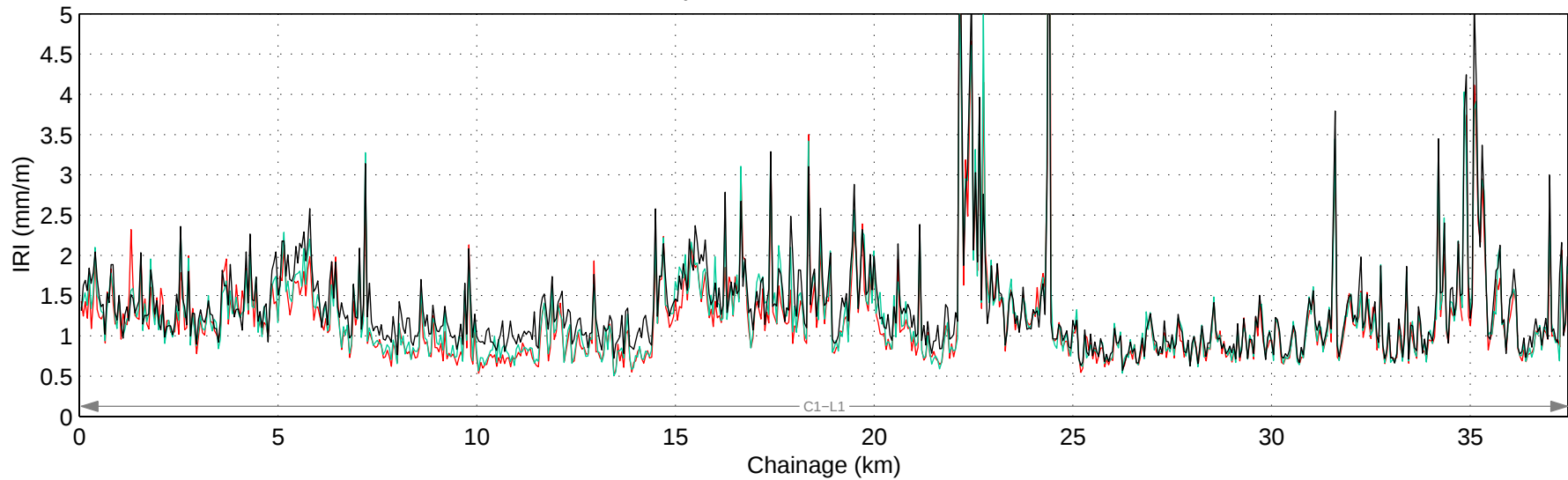
Hwy 583:02 Mean IRI – Right Lane
