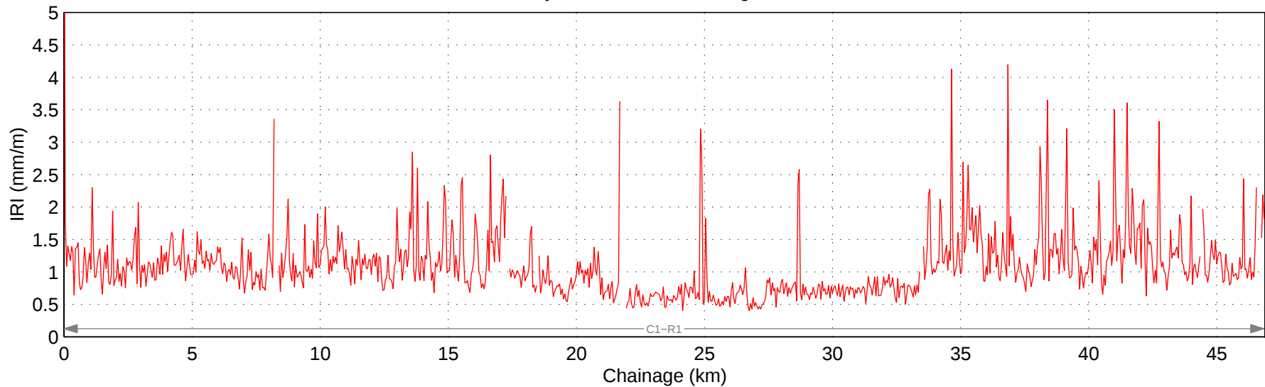
Hwy 505:02 Mean IRI – Right Lane
