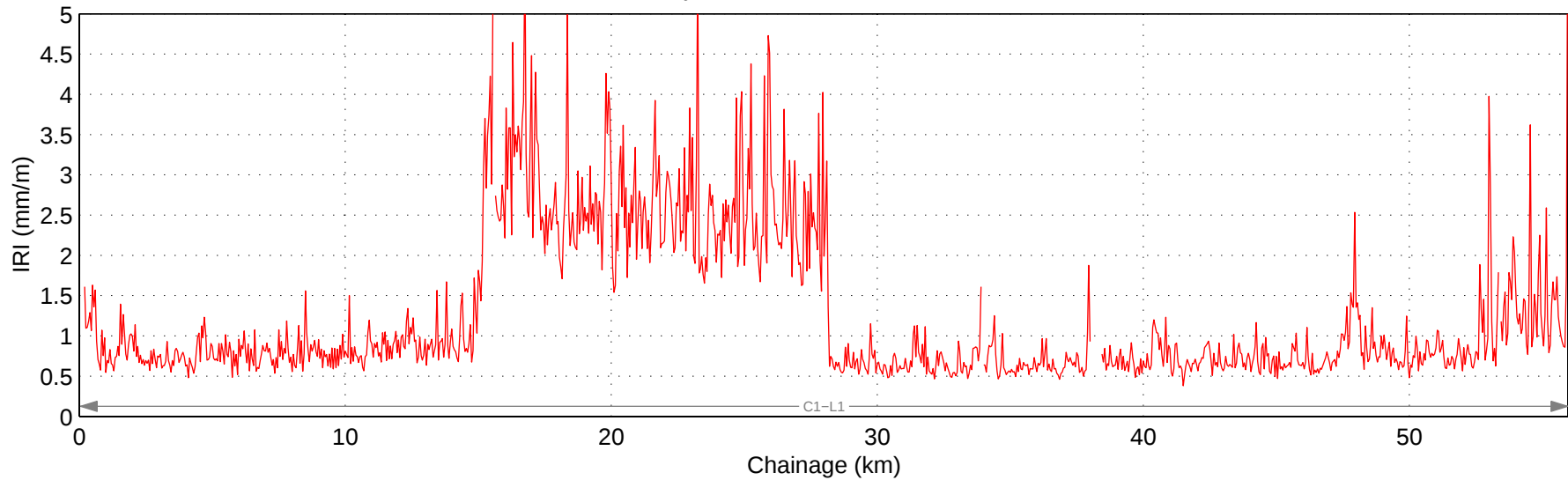
Hwy 582:04 Mean IRI – Right Lane
