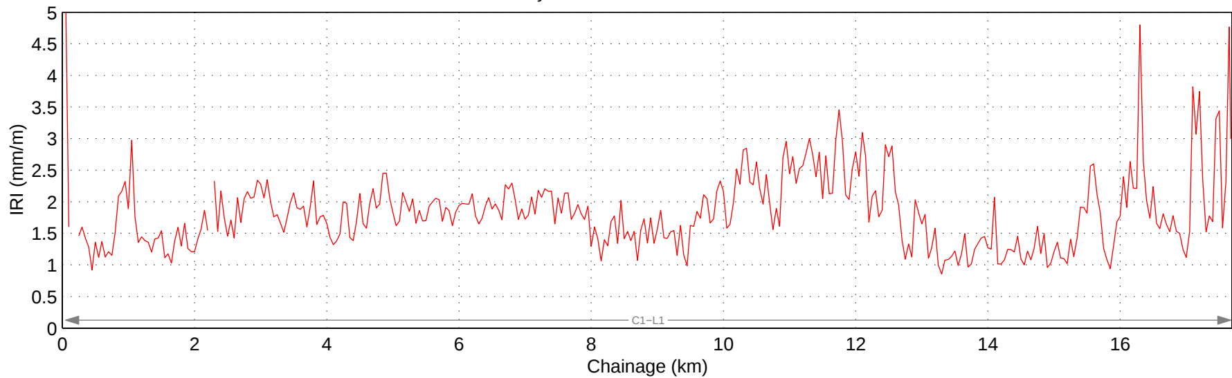
Hwy 519:04 Mean IRI – Right Lane
