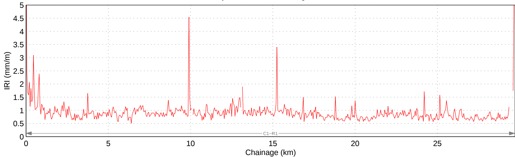
Hwy 580:02 Mean IRI – Right Lane
