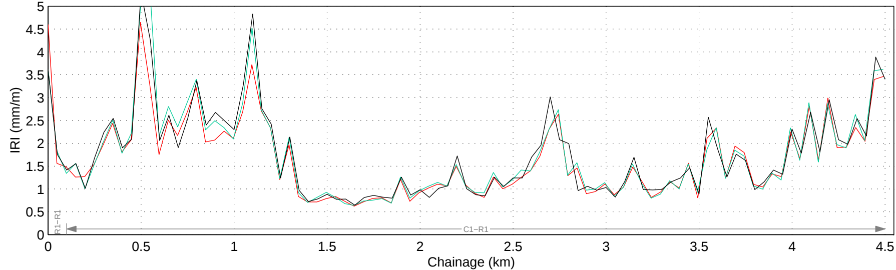
Hwy 501:01 Mean IRI – Right Lane
