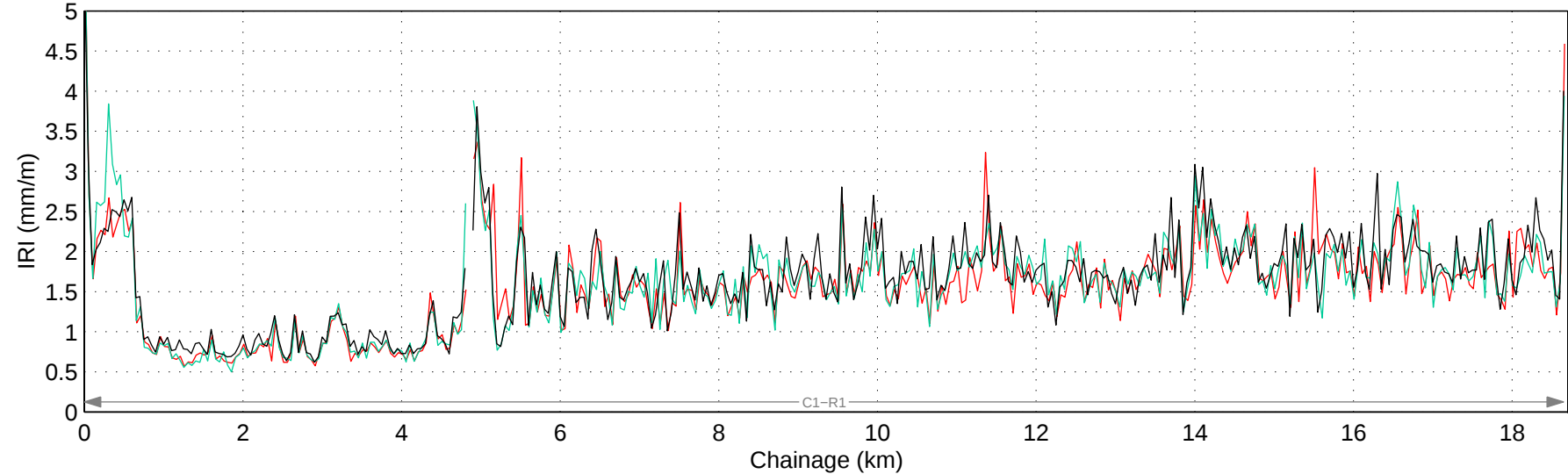
Hwy 581:02 Mean IRI – Right Lane
