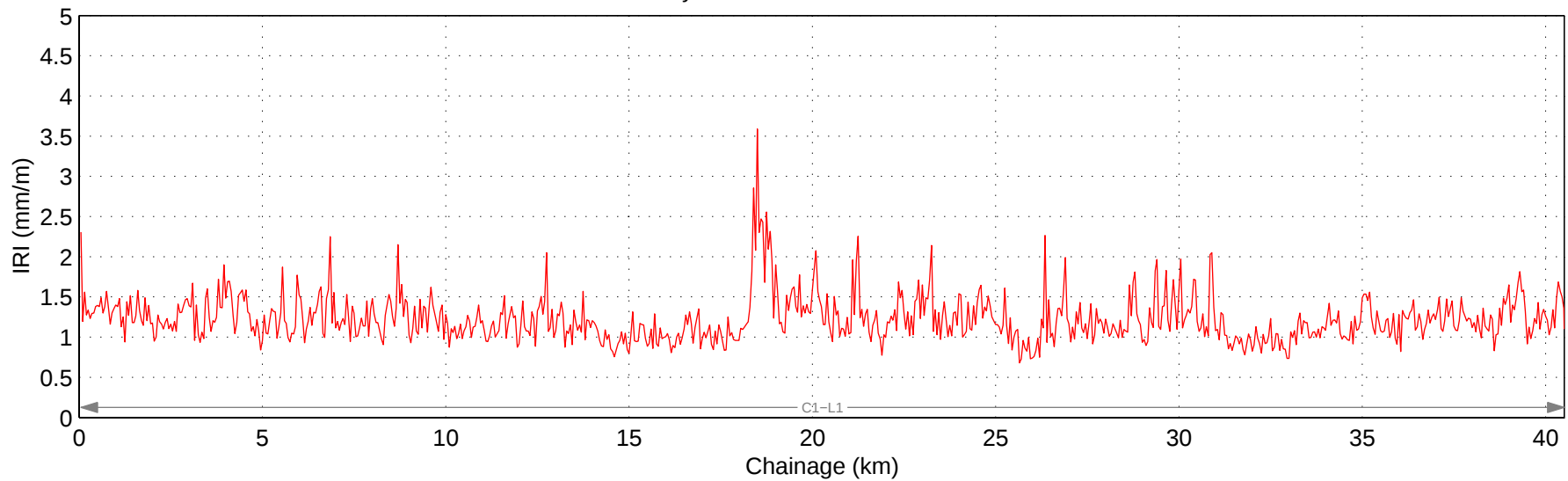
Hwy 589:02 Mean IRI – Right Lane
