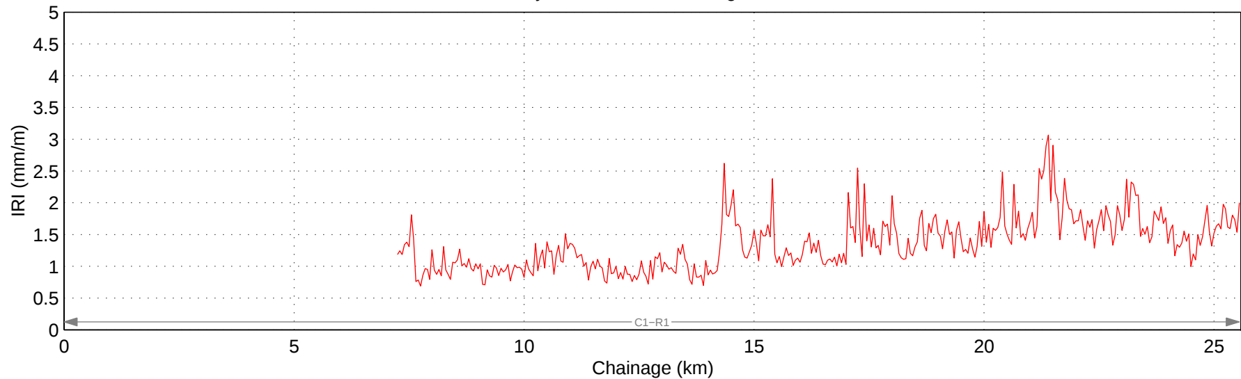
Hwy 523:02 Mean IRI – Right Lane
