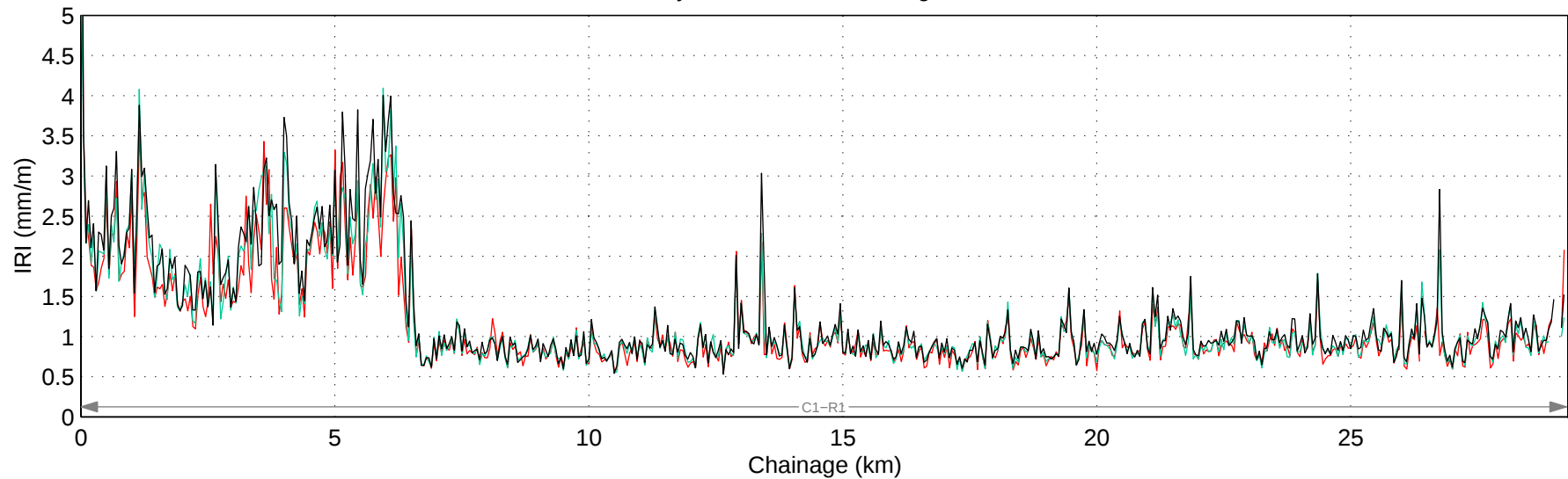
Hwy 564:06 Mean IRI – Right Lane
