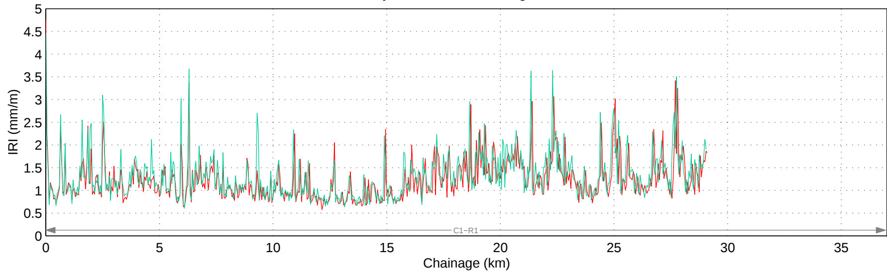
Hwy 576:02 Mean IRI – Right Lane
