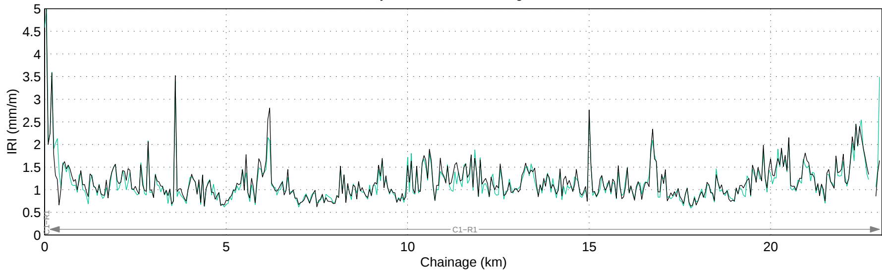
Hwy 598:02 Mean IRI – Right Lane
