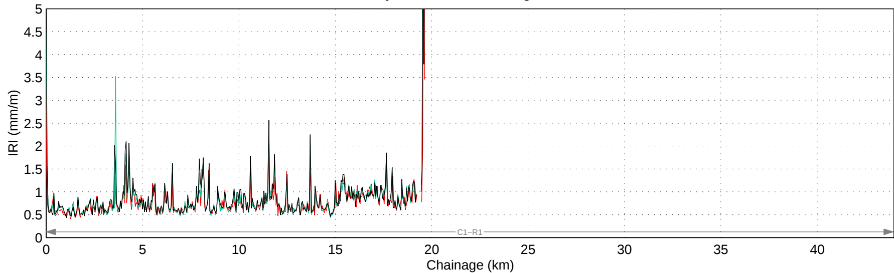
Hwy 564:08 Mean IRI – Right Lane
