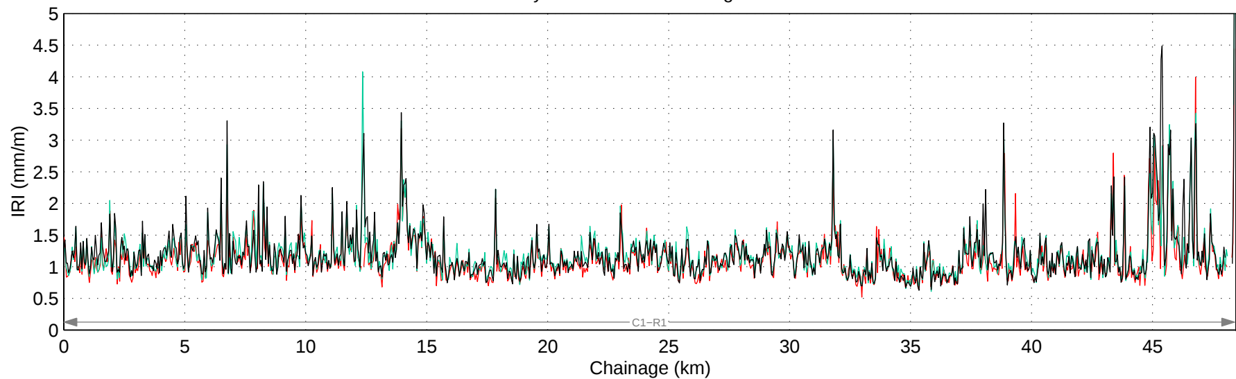
Hwy 570:01 Mean IRI – Right Lane
