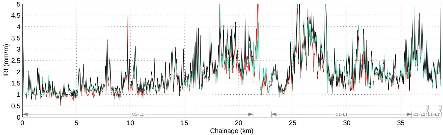
Hwy 575:04 Mean IRI – Right Lane
