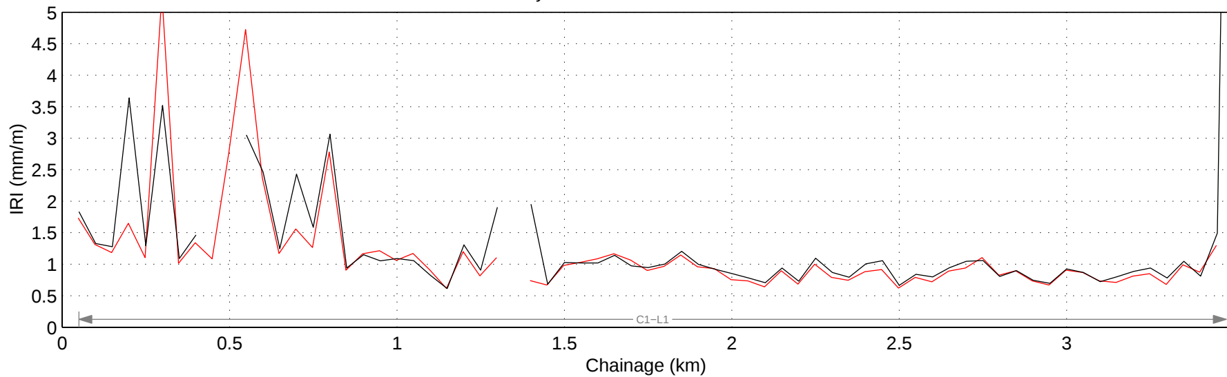
Hwy 599:02 Mean IRI – Right Lane
