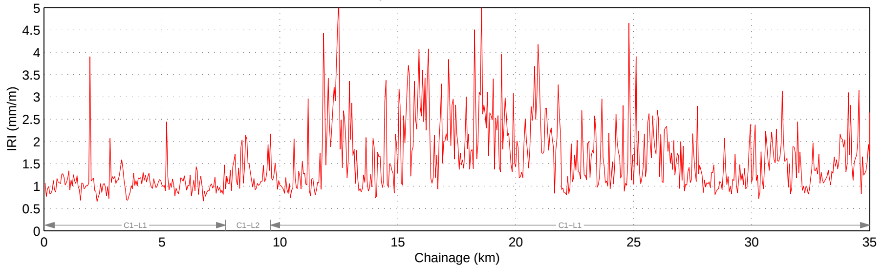
Hwy 595:02 Mean IRI – Right Lane
