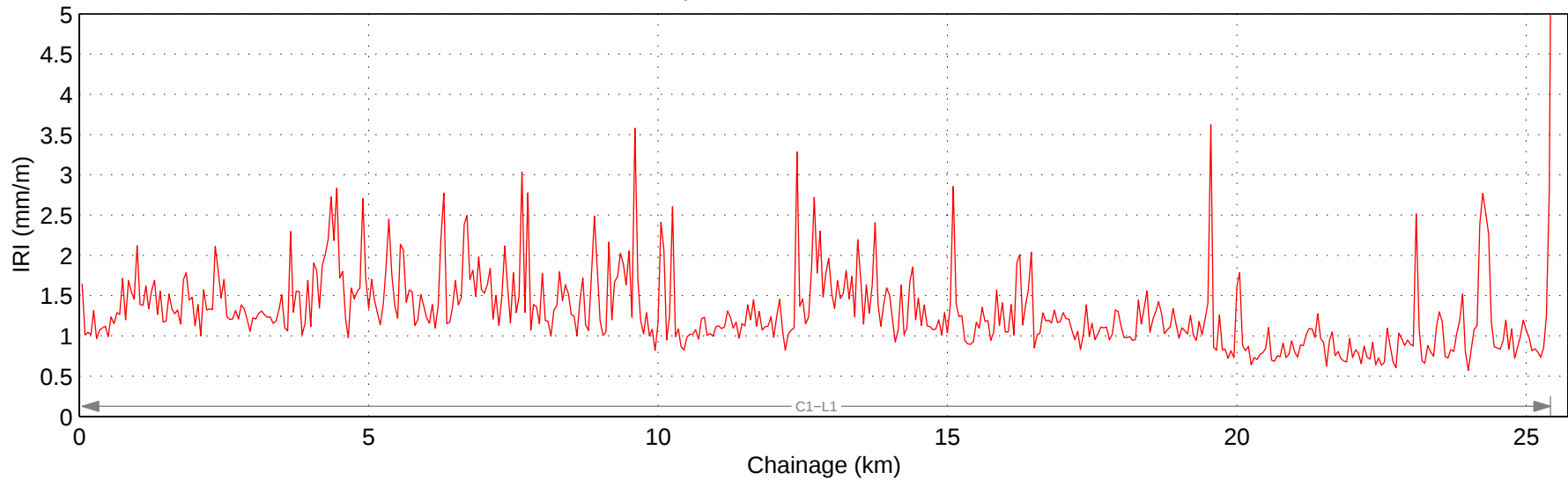
Hwy 549:04 Mean IRI – Right Lane
