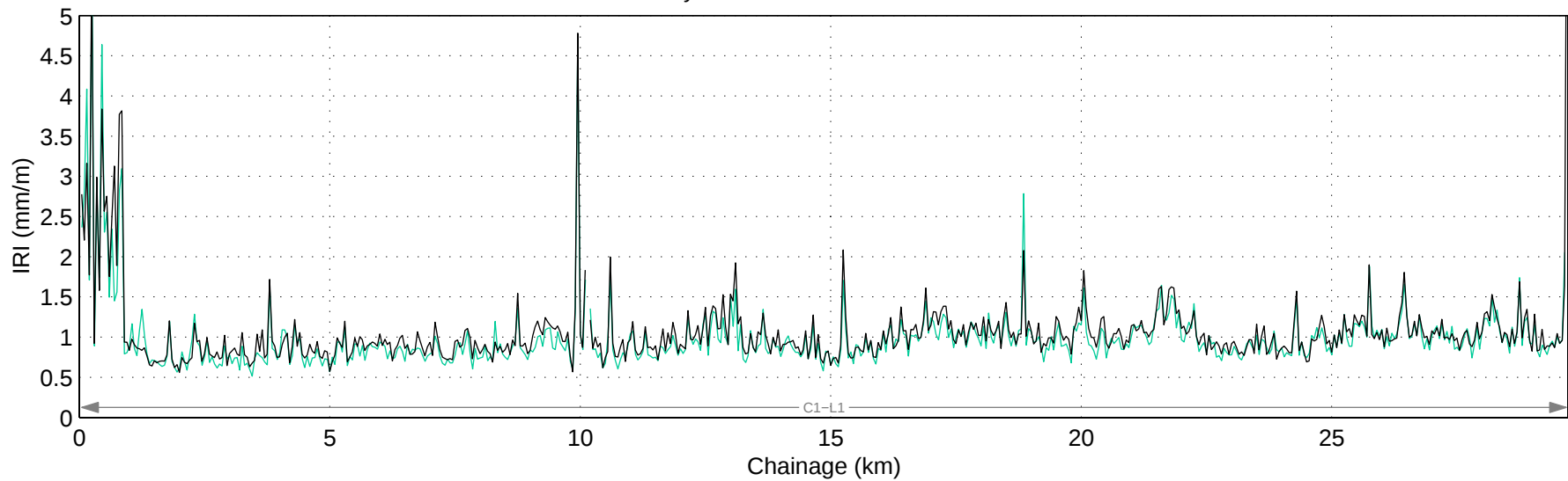
Hwy 580:02 Mean IRI – Right Lane
