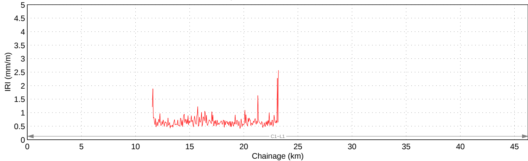
Hwy 506:02 Mean IRI – Right Lane
