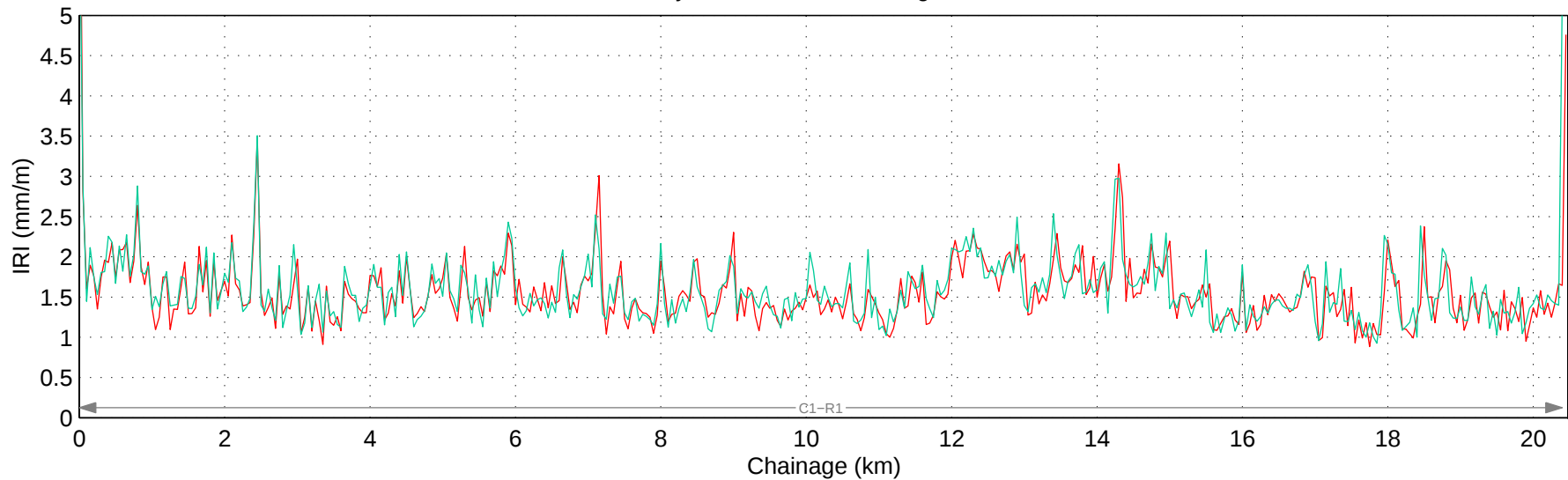
Hwy 530:02 Mean IRI – Right Lane
