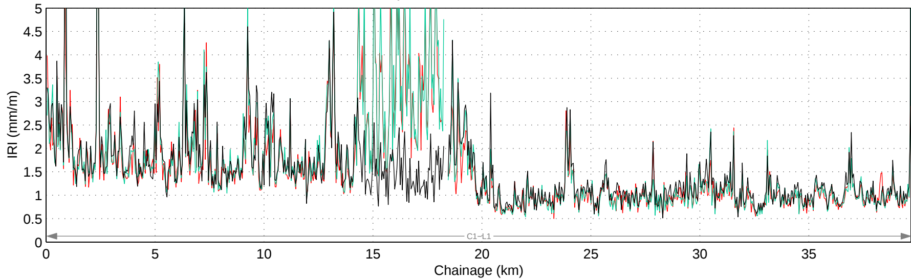
Hwy 585:02 Mean IRI – Right Lane
