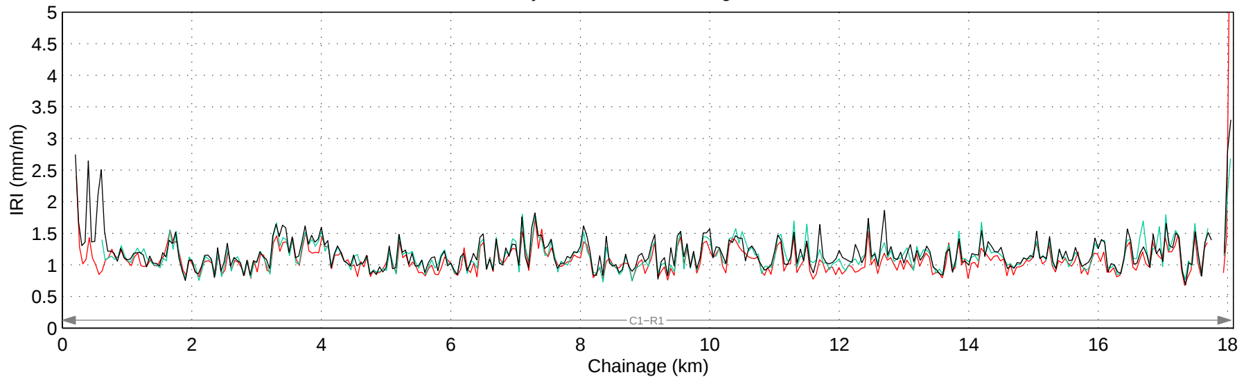
Hwy 539:04 Mean IRI – Right Lane
