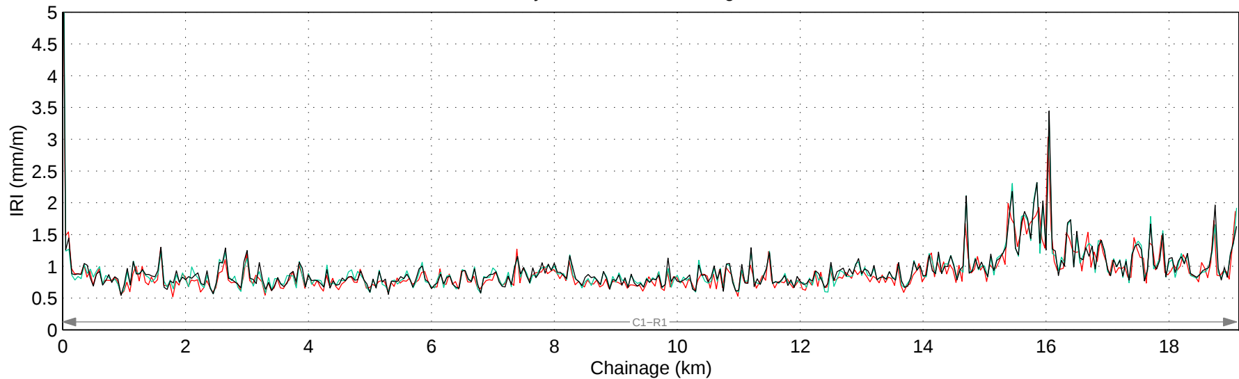
Hwy 570:10 Mean IRI – Right Lane
