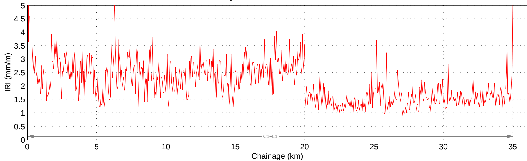
Hwy 547:02 Mean IRI – Right Lane
