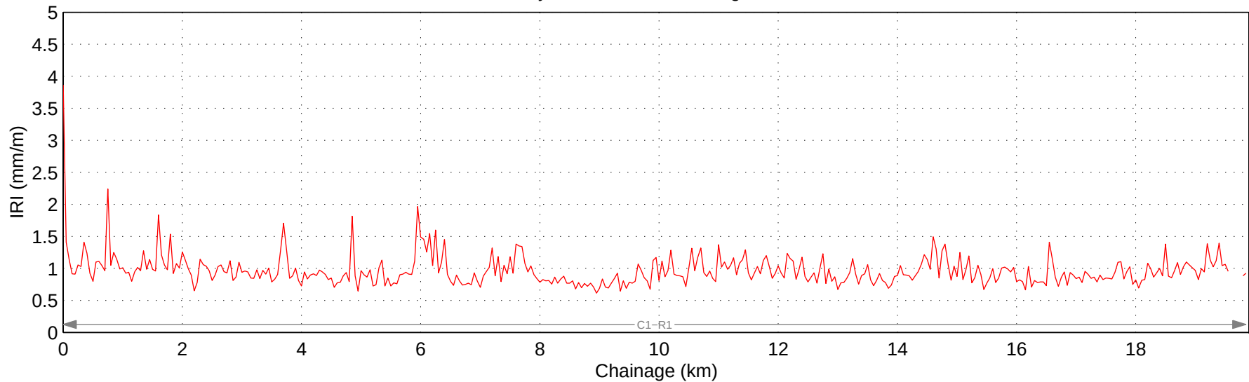
Hwy 792:04 Mean IRI – Right Lane
