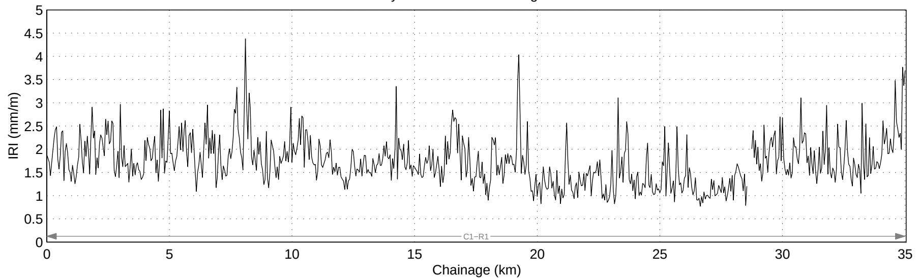
Hwy 754:06 Mean IRI – Right Lane
