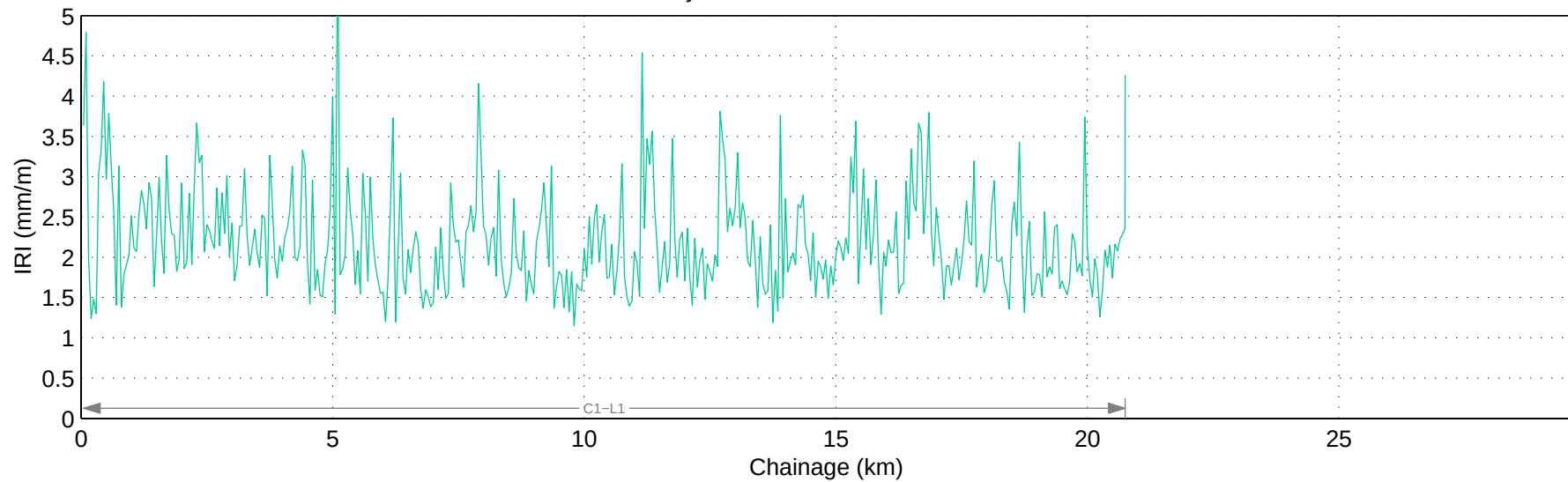
Hwy 736:02 Mean IRI – Right Lane
