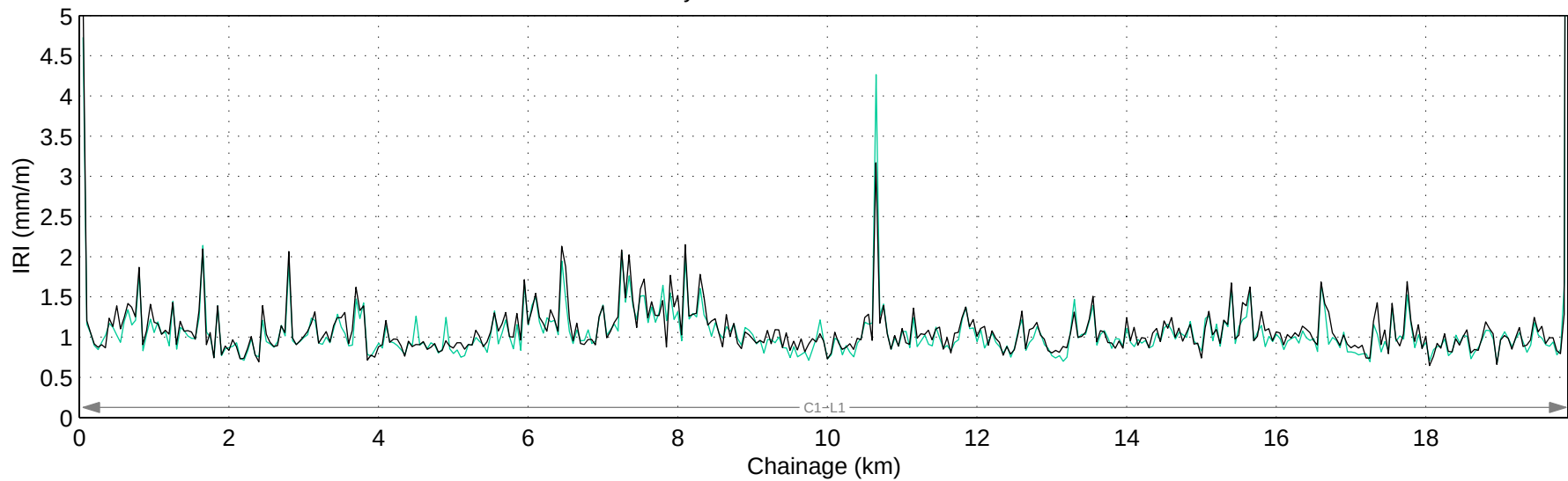
Hwy 792:04 Mean IRI – Right Lane
