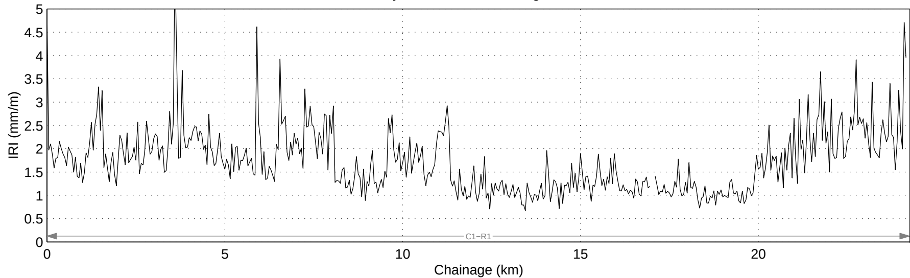
Hwy 770:04 Mean IRI – Right Lane
