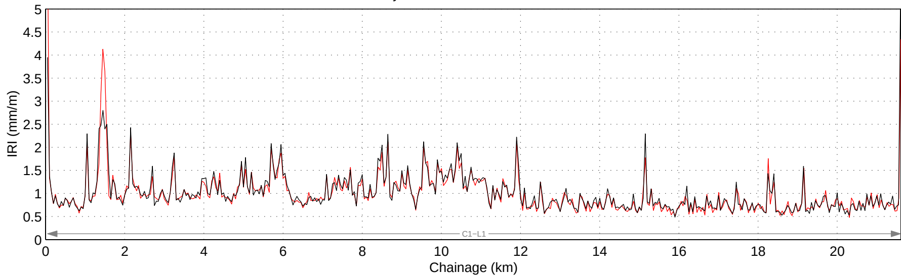
Hwy 771:02 Mean IRI – Right Lane
