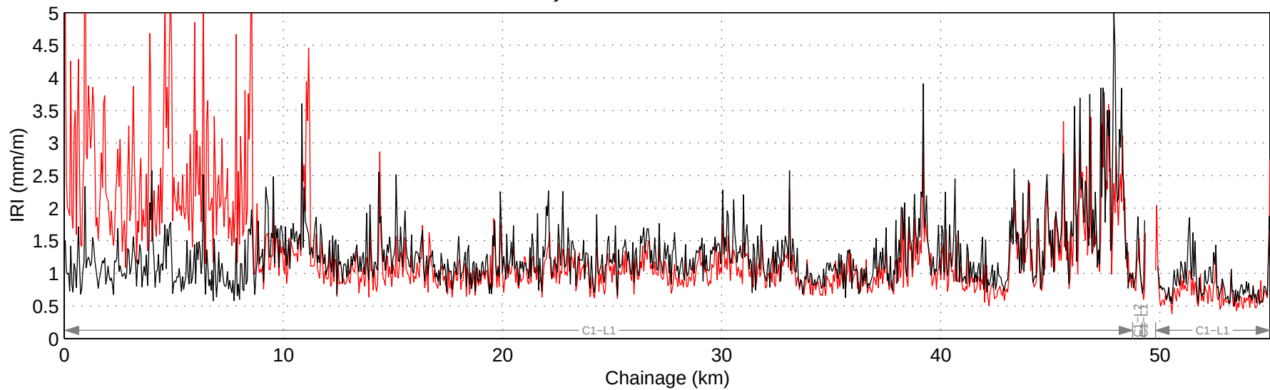
Hwy 740:02 Mean IRI – Right Lane
