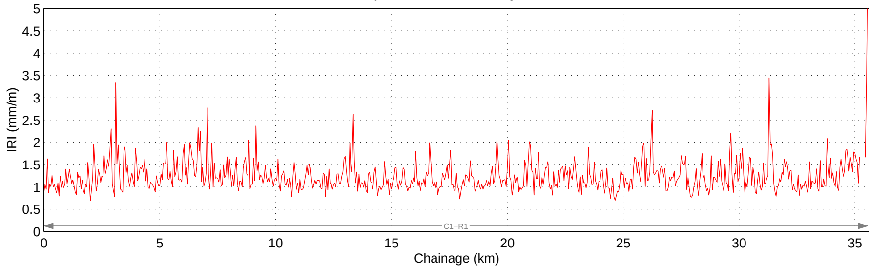
Hwy 750:06 Mean IRI – Right Lane
