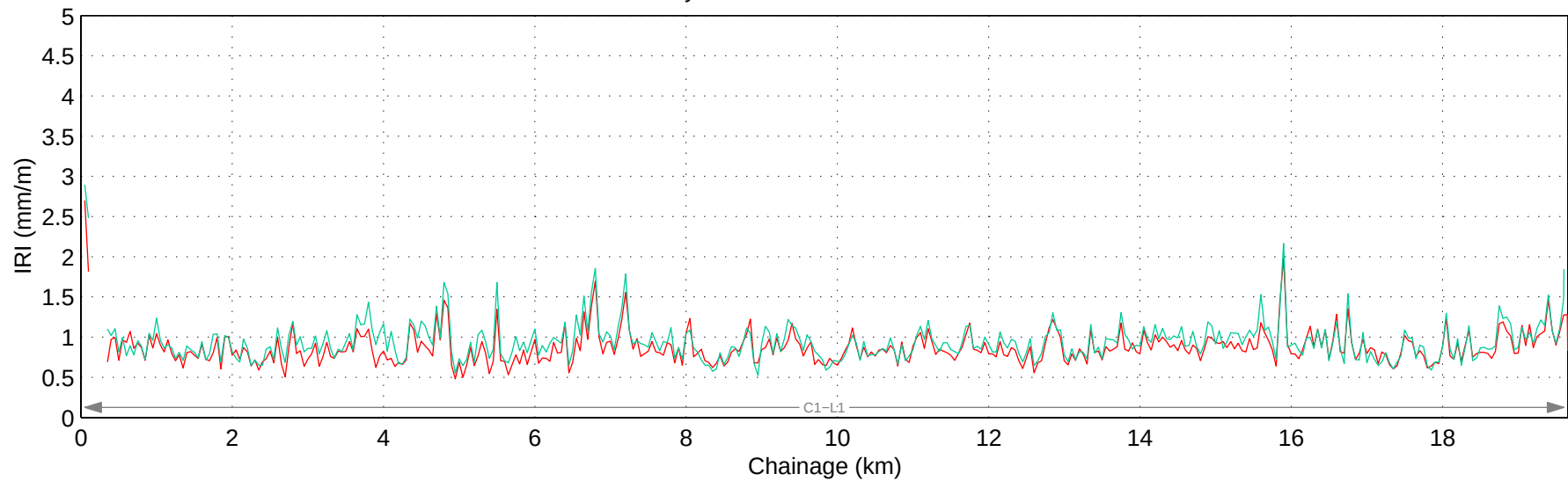
Hwy 754:02 Mean IRI – Right Lane
