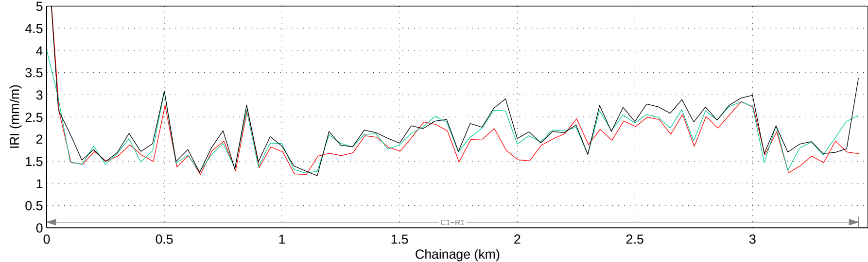
Hwy 727:02 Mean IRI – Right Lane
