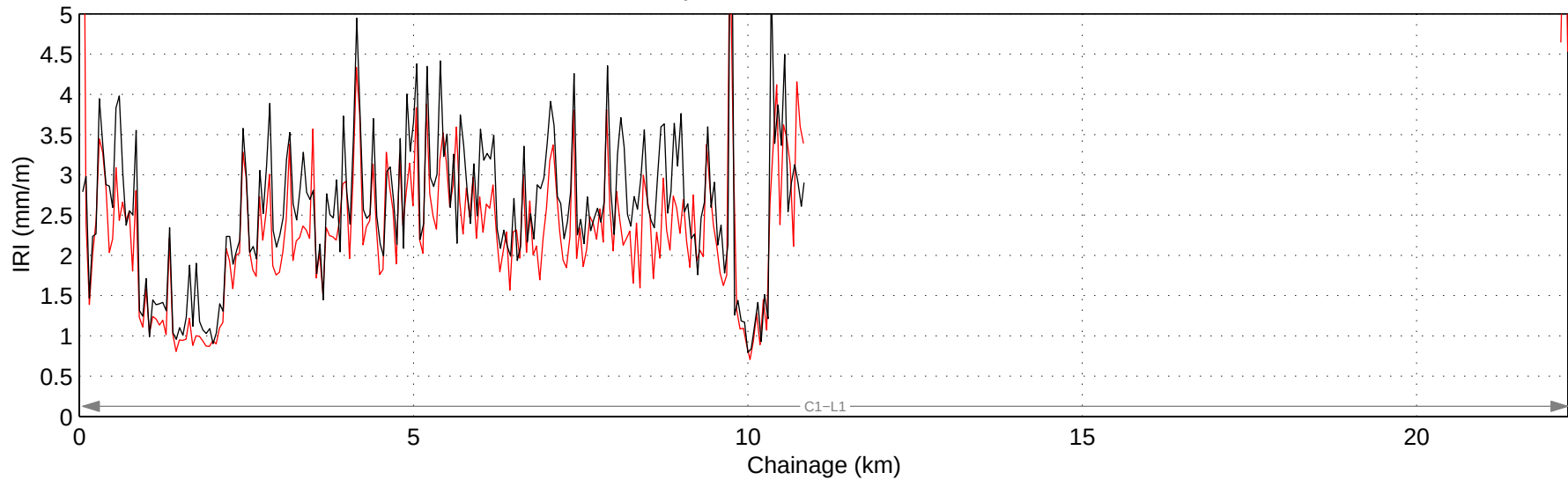
Hwy 771:03 Mean IRI – Right Lane
