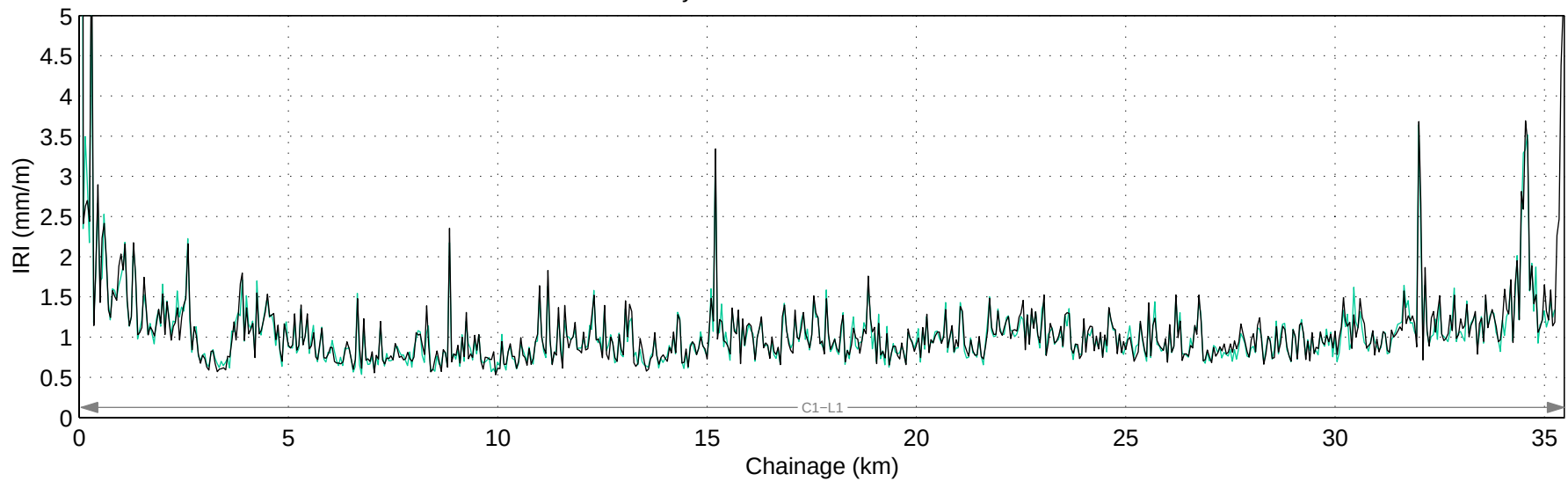
Hwy 757:02 Mean IRI – Right Lane
