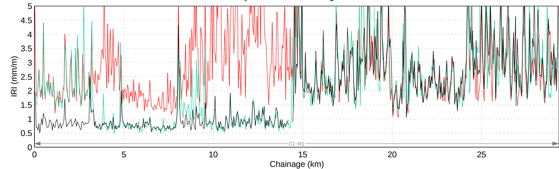
Hwy 766:04 Mean IRI – Right Lane
