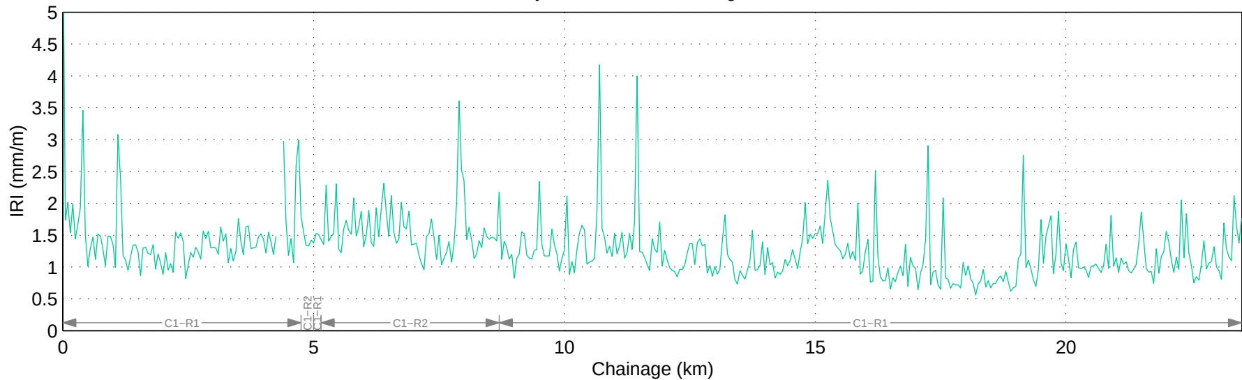
Hwy 753:02 Mean IRI – Right Lane
