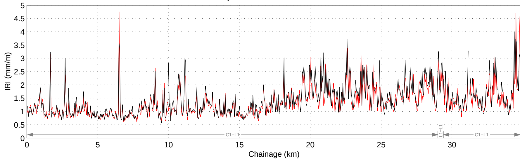
Hwy 752:04 Mean IRI – Right Lane
