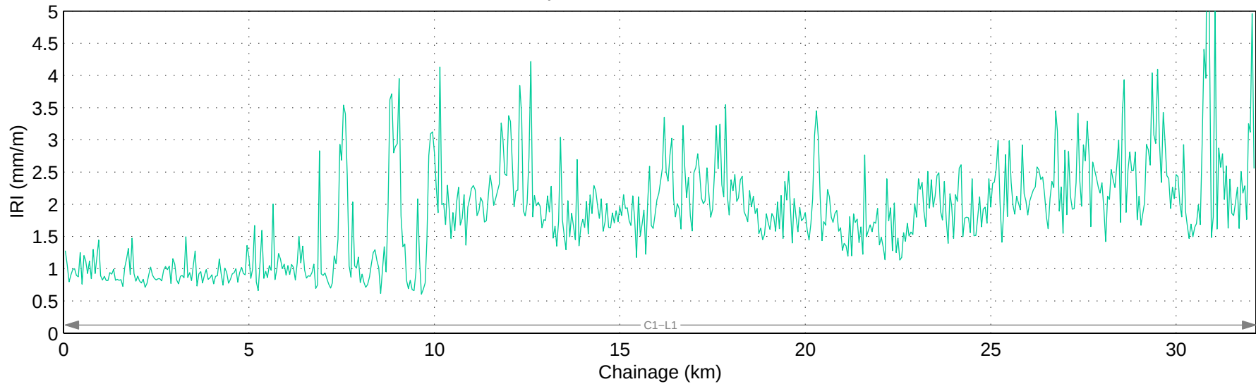
Hwy 733:04 Mean IRI – Right Lane
