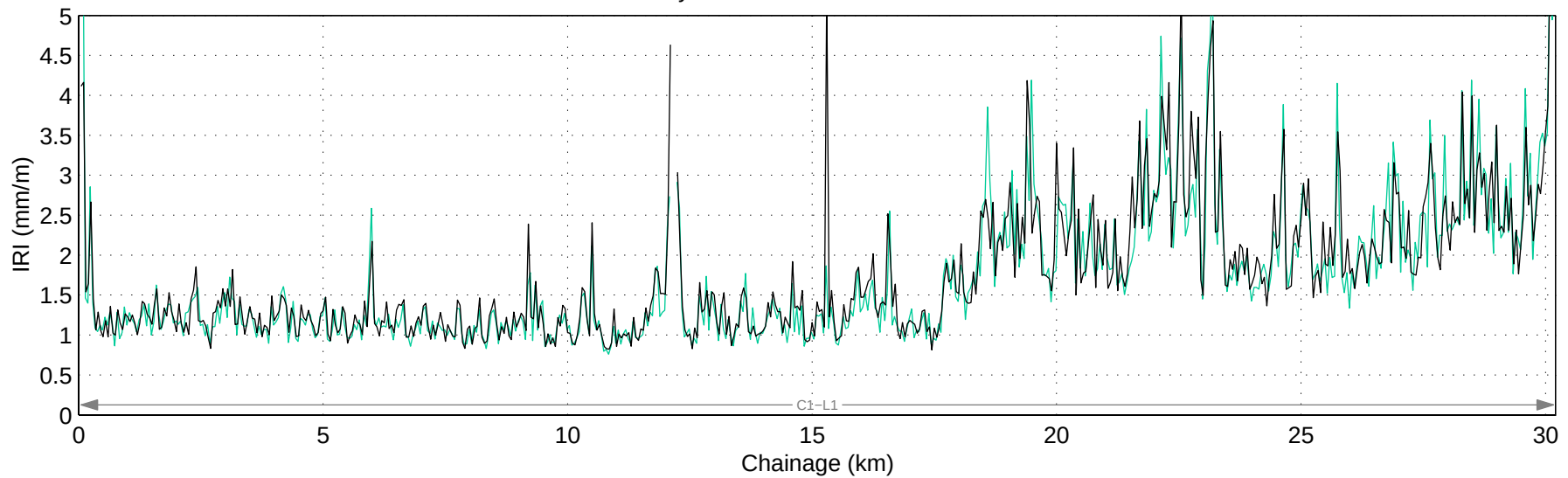
Hwy 764:02 Mean IRI – Right Lane
