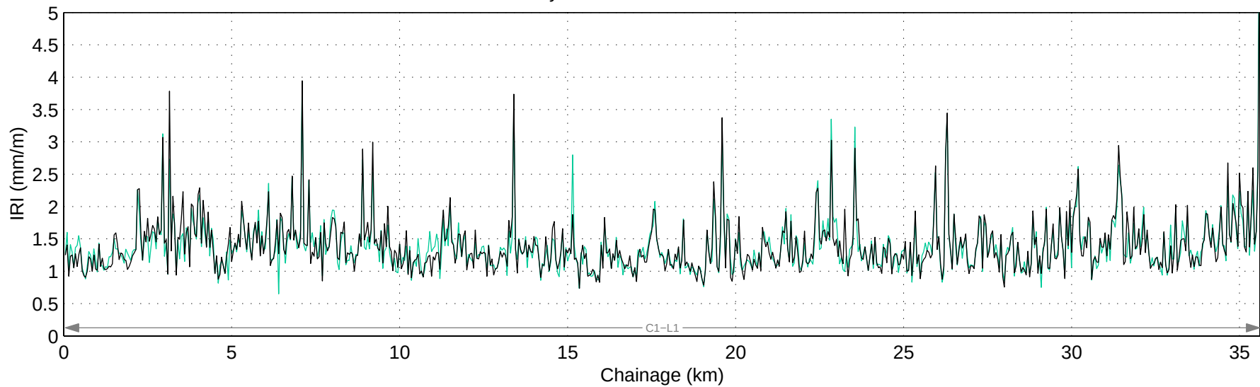
Hwy 750:06 Mean IRI – Right Lane
