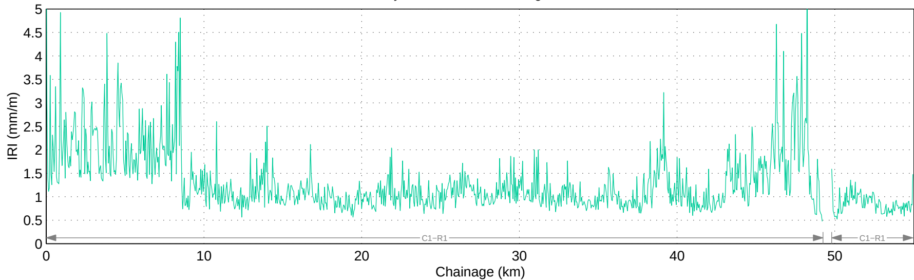
Hwy 740:02 Mean IRI – Right Lane
