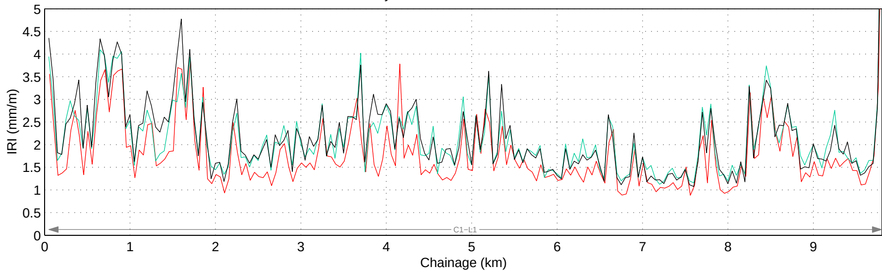
Hwy 791:05 Mean IRI – Right Lane
