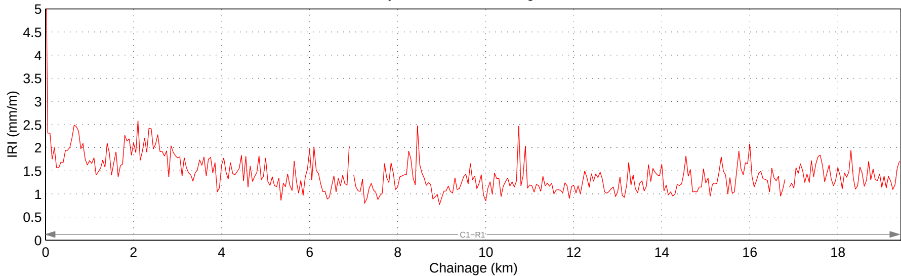
Hwy 776:02 Mean IRI – Right Lane
