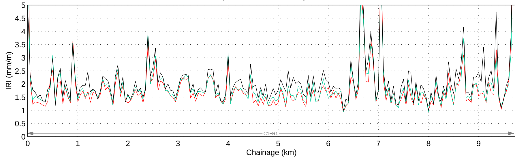
Hwy 739:02 Mean IRI – Right Lane
