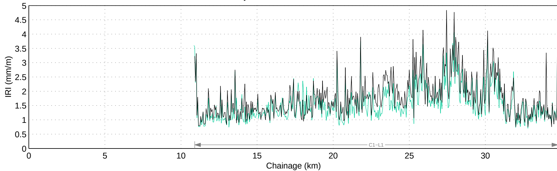
Hwy 737:02 Mean IRI – Right Lane
