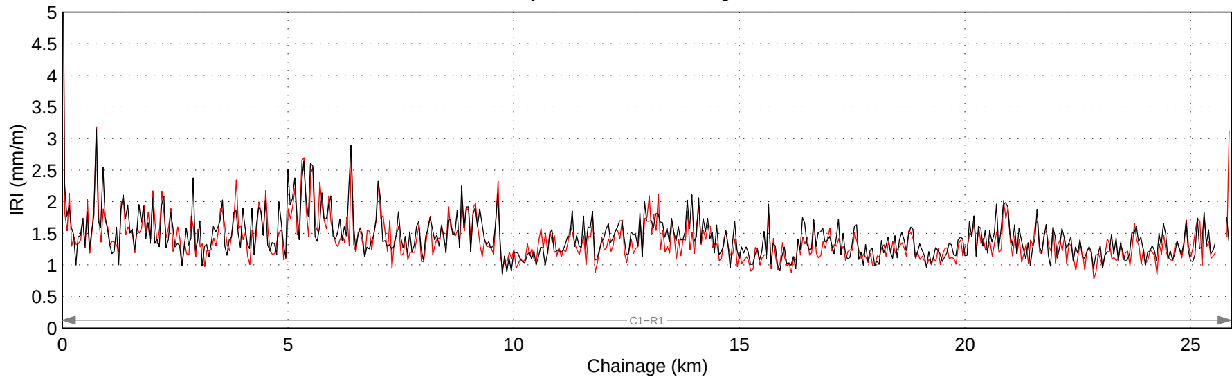
Hwy 761:02 Mean IRI – Right Lane
