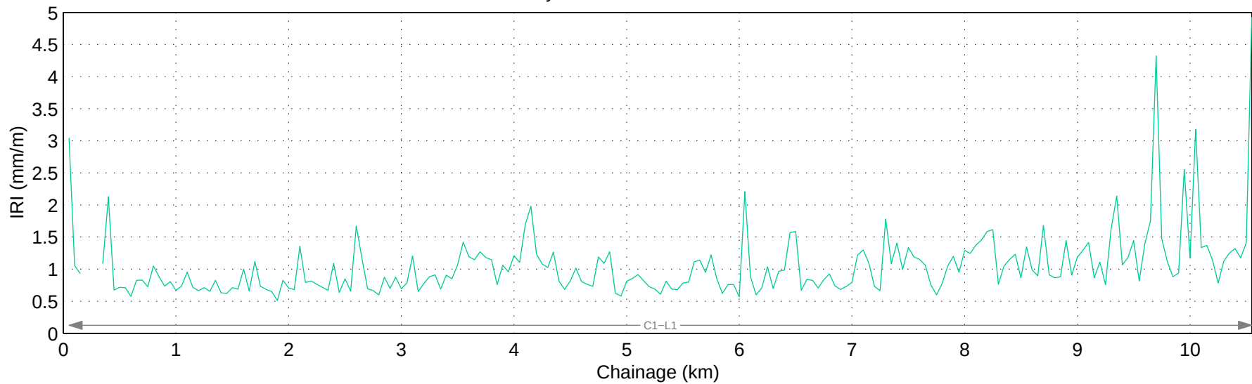
Hwy 777:04 Mean IRI – Right Lane
