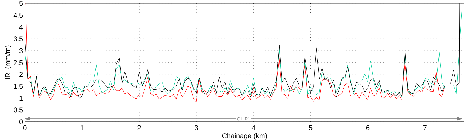
Hwy 721:02 Mean IRI – Right Lane
