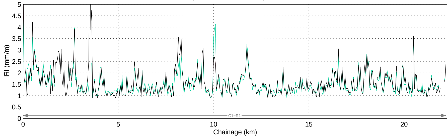
Hwy 762:02 Mean IRI – Right Lane
