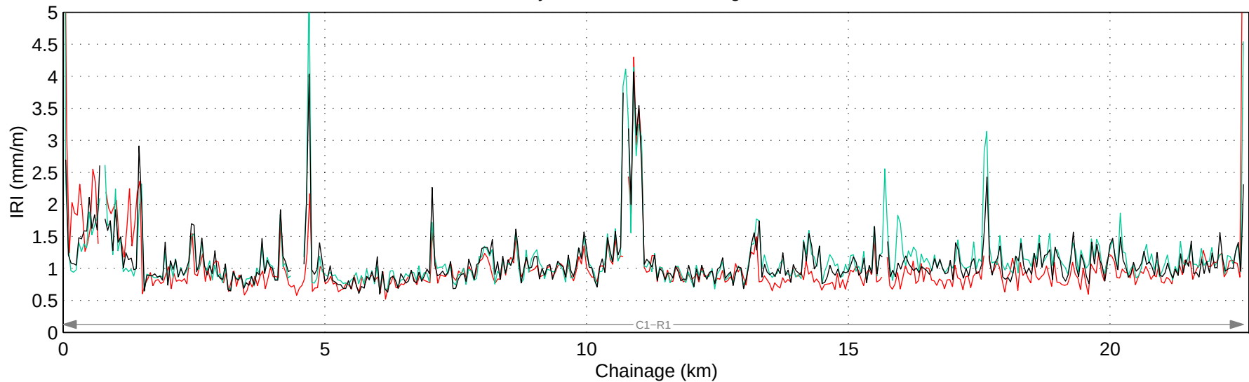
Hwy 748:02 Mean IRI – Right Lane
