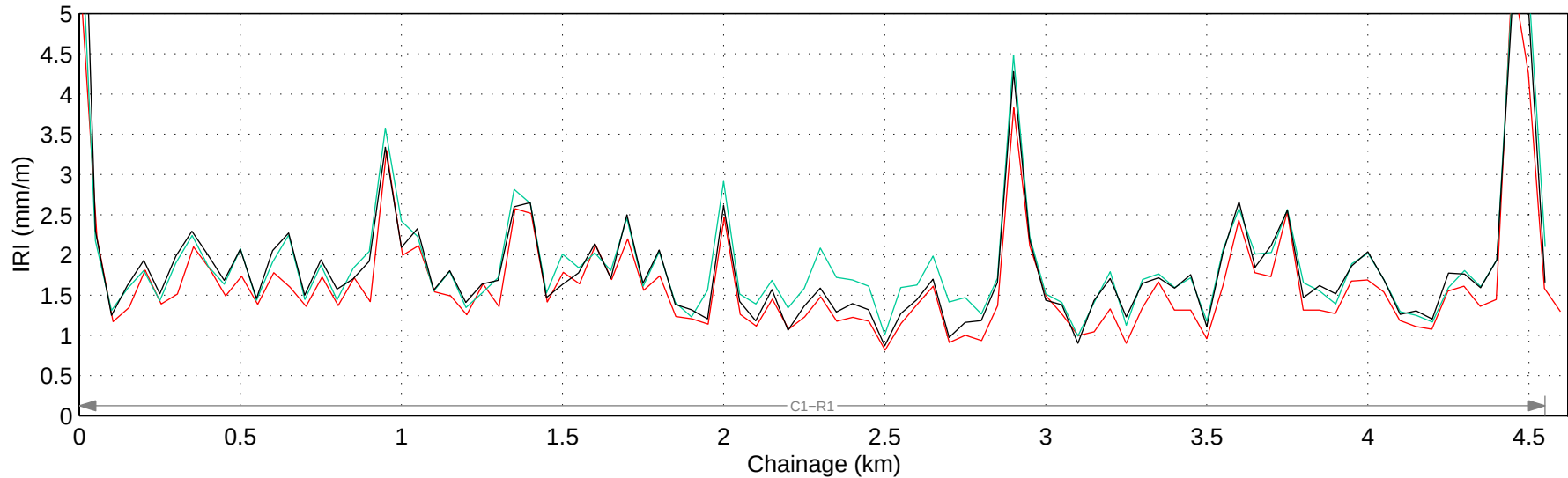
Hwy 756:02 Mean IRI – Right Lane
