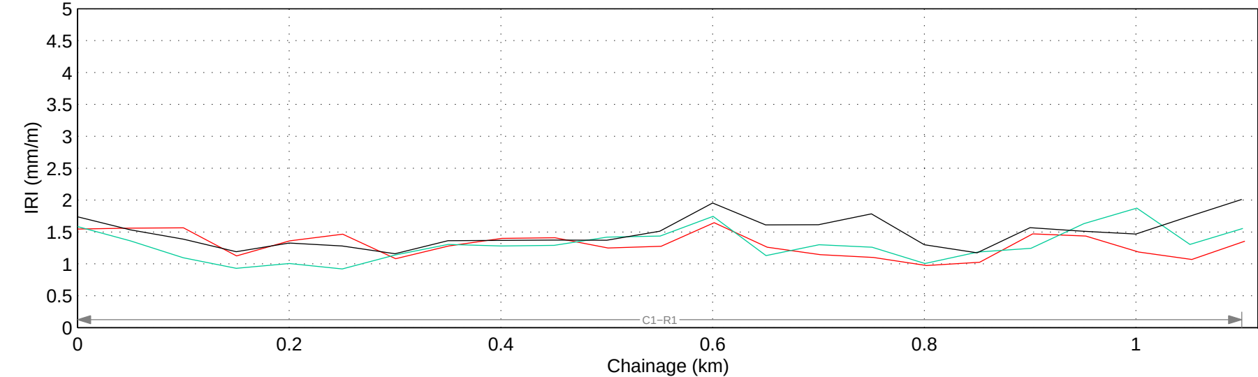
Hwy 741:02 Mean IRI – Right Lane
