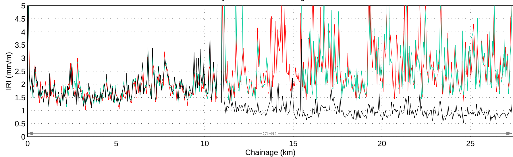
Hwy 766:02 Mean IRI – Right Lane
