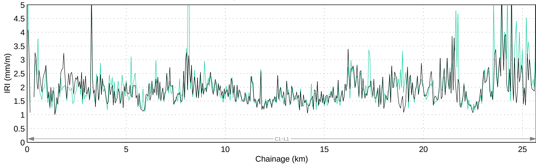
Hwy 763:02 Mean IRI – Right Lane
