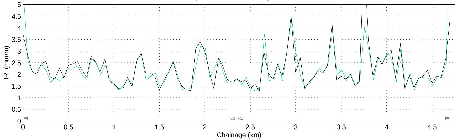
Hwy 758:02 Mean IRI – Right Lane
