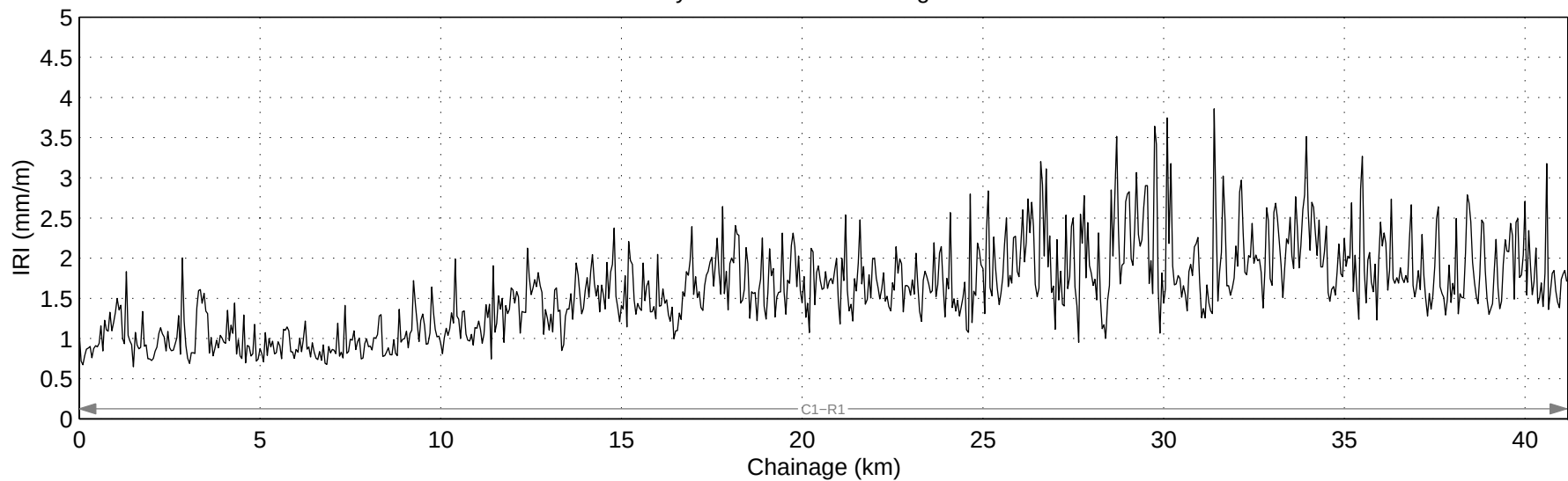
Hwy 754:04 Mean IRI – Right Lane
