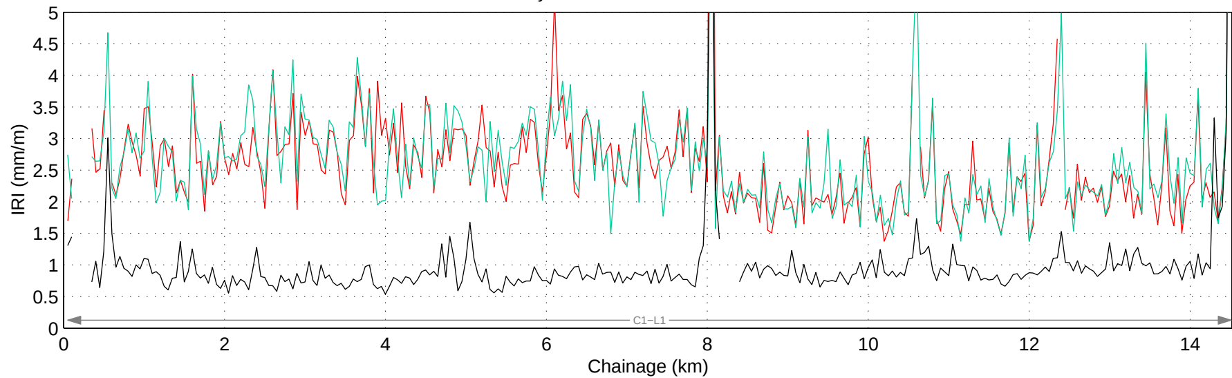
Hwy 791:02 Mean IRI – Right Lane
