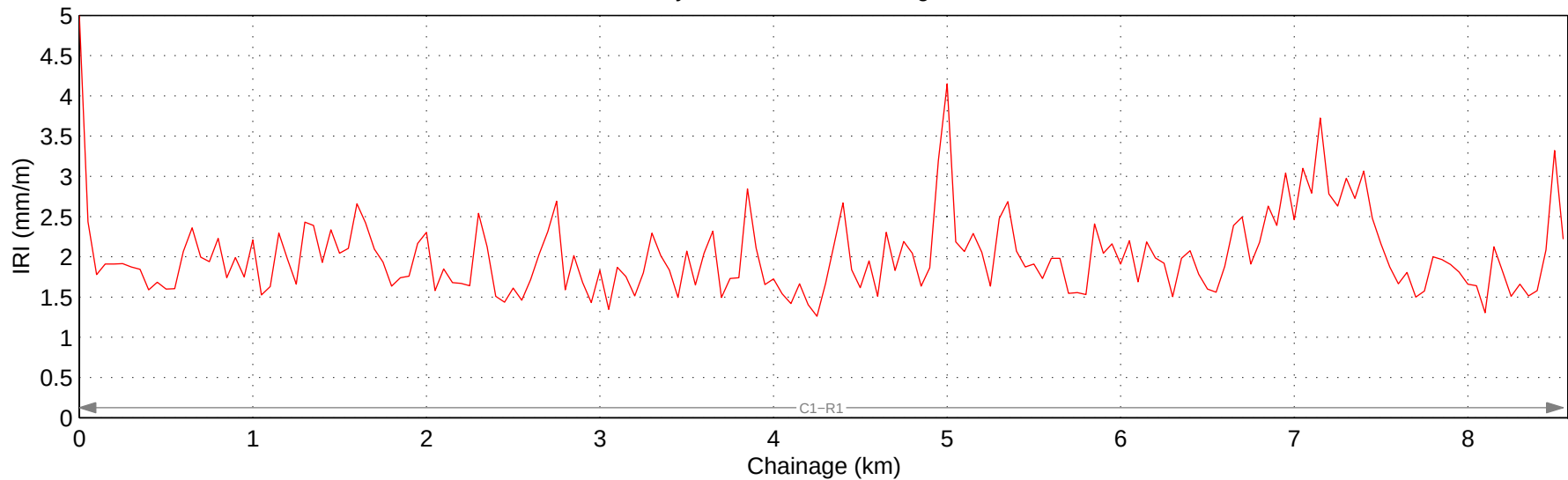
Hwy 780:02 Mean IRI – Right Lane
