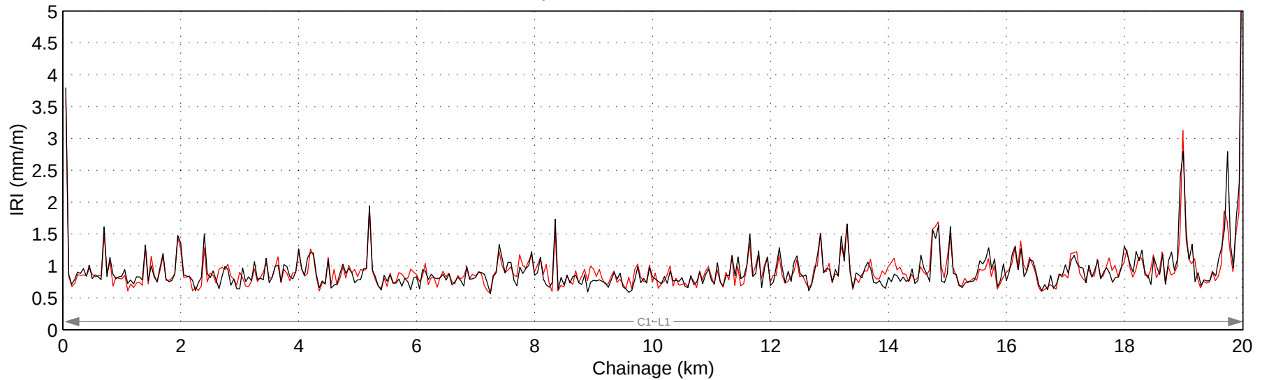
Hwy 751:04 Mean IRI – Right Lane
