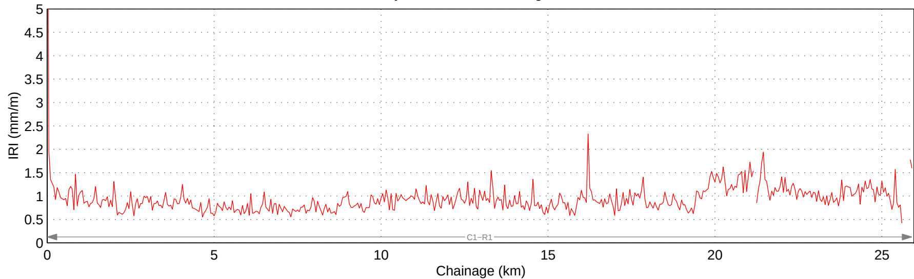
Hwy 724:04 Mean IRI – Right Lane
