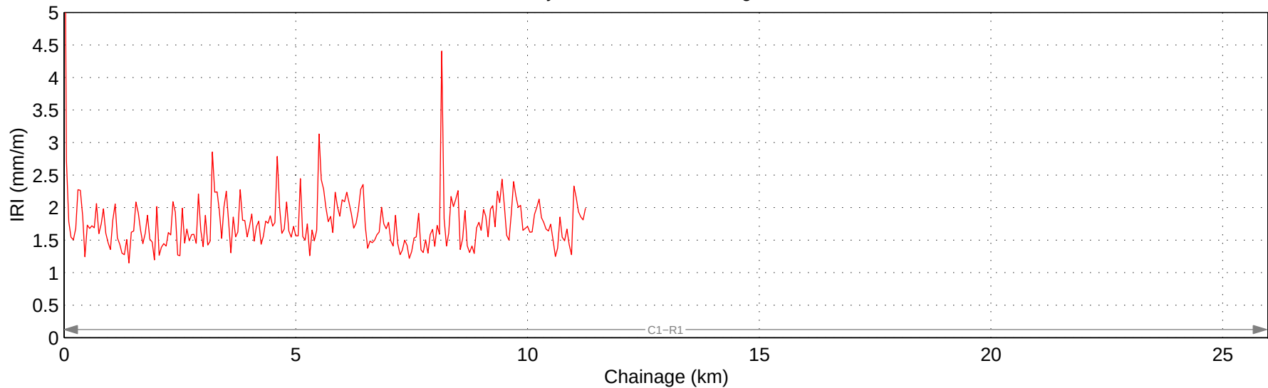
Hwy 791:08 Mean IRI – Right Lane
