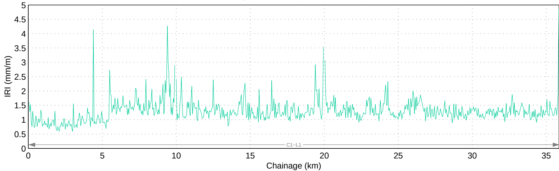
Hwy 748:04 Mean IRI – Right Lane
