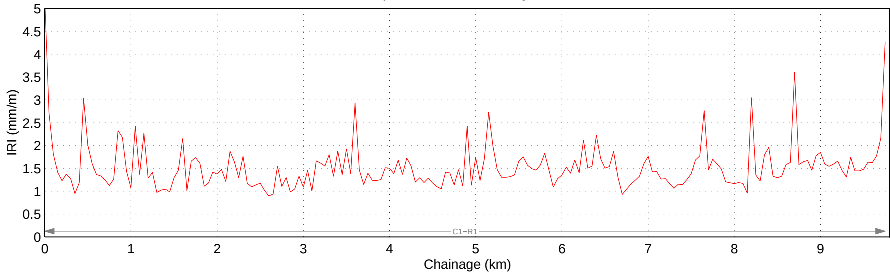
Hwy 791:05 Mean IRI – Right Lane
