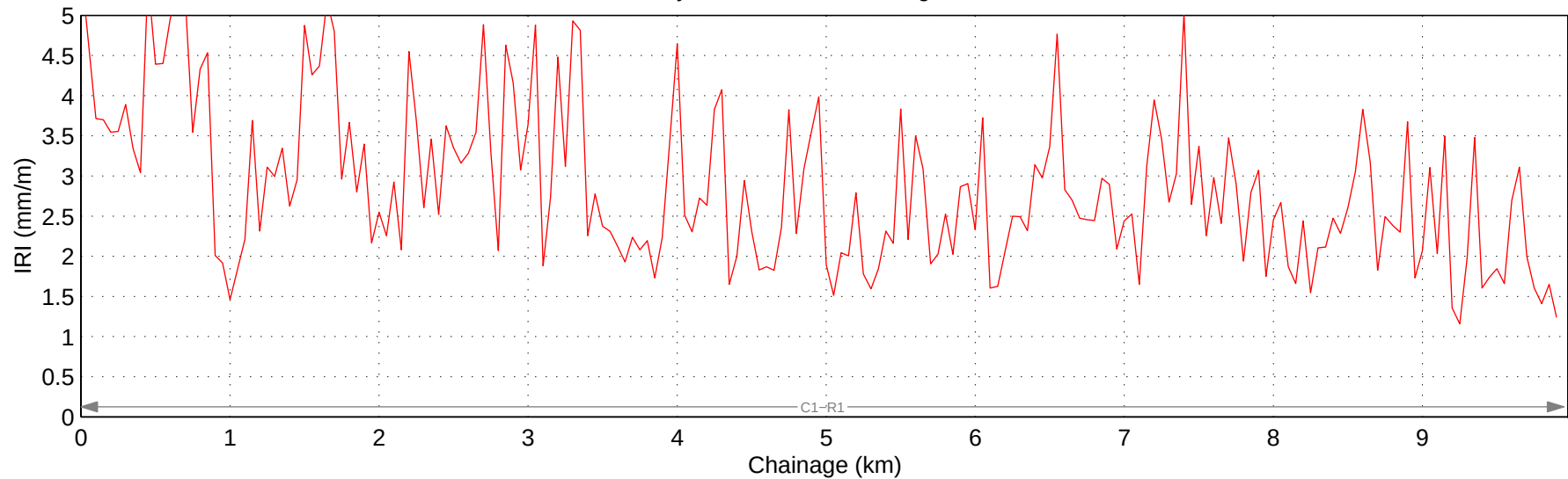
Hwy 760:02 Mean IRI – Right Lane
