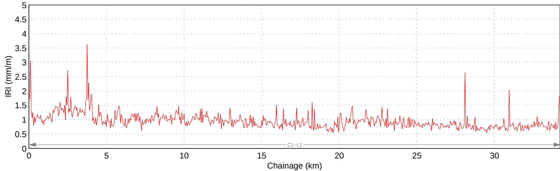
Hwy 751:02 Mean IRI – Right Lane
