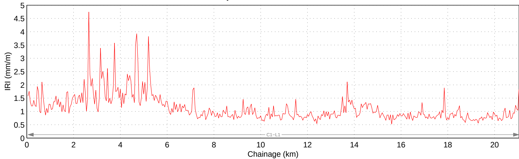
Hwy 759:04 Mean IRI – Right Lane
