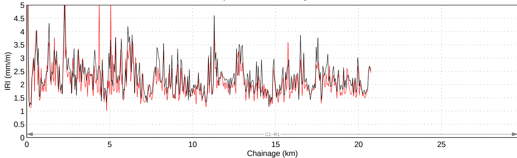
Hwy 736:02 Mean IRI – Right Lane
