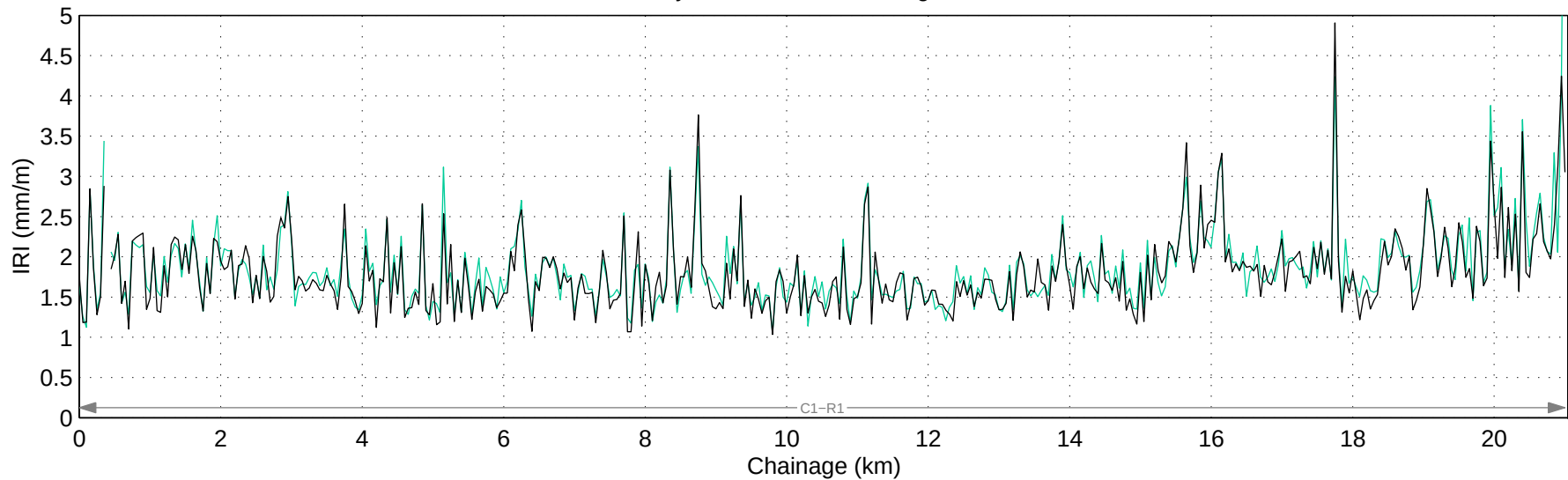
Hwy 731:02 Mean IRI – Right Lane
