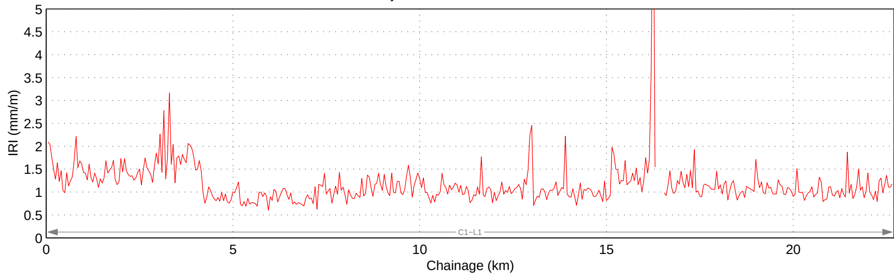
Hwy 799:02 Mean IRI – Right Lane
