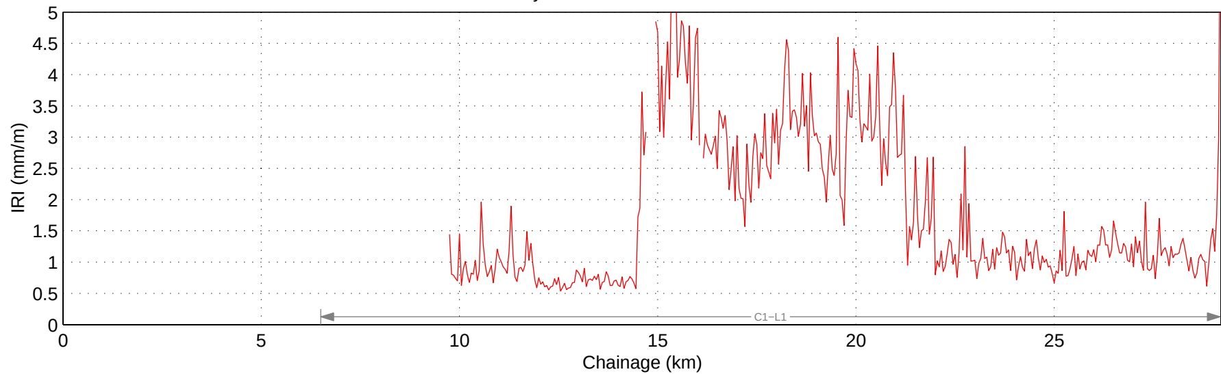
Hwy 797:02 Mean IRI – Right Lane
