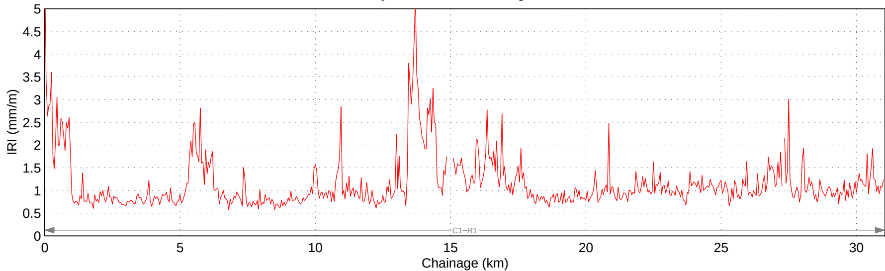
Hwy 750:02 Mean IRI – Right Lane
