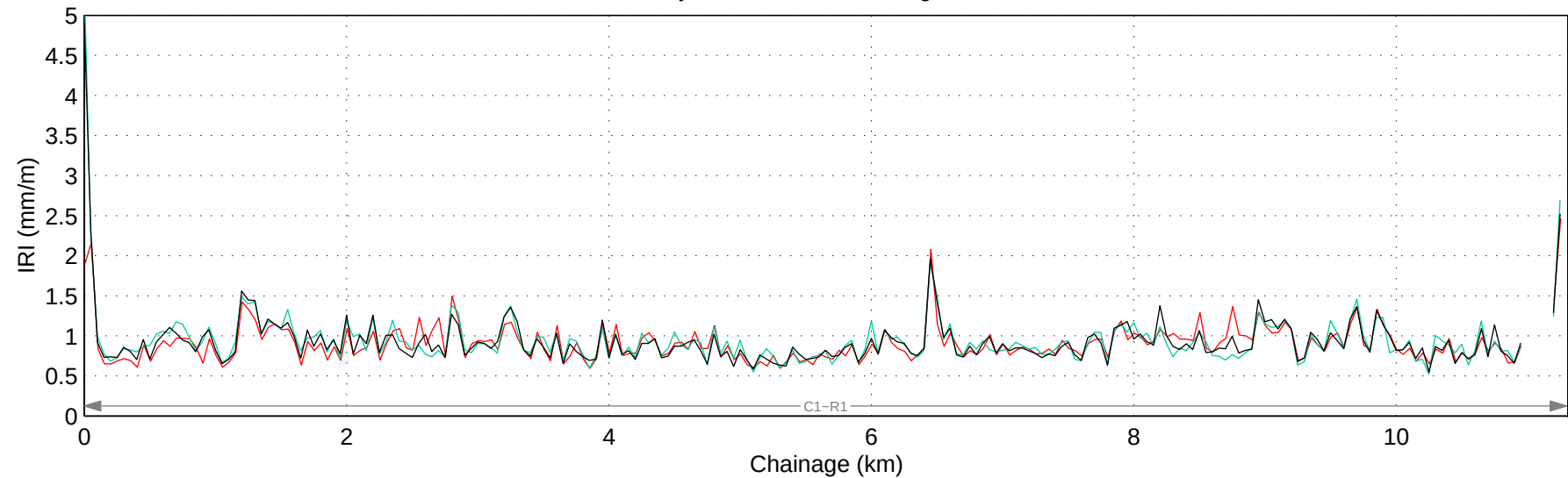
Hwy 783:02 Mean IRI – Right Lane
