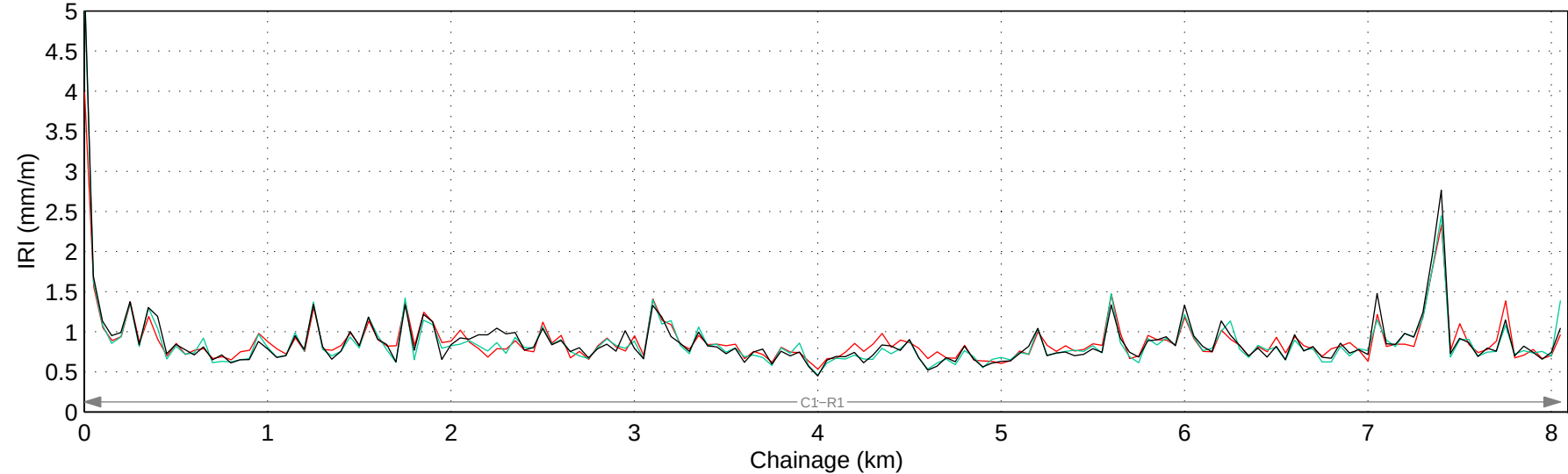
Hwy 761:06 Mean IRI – Right Lane
