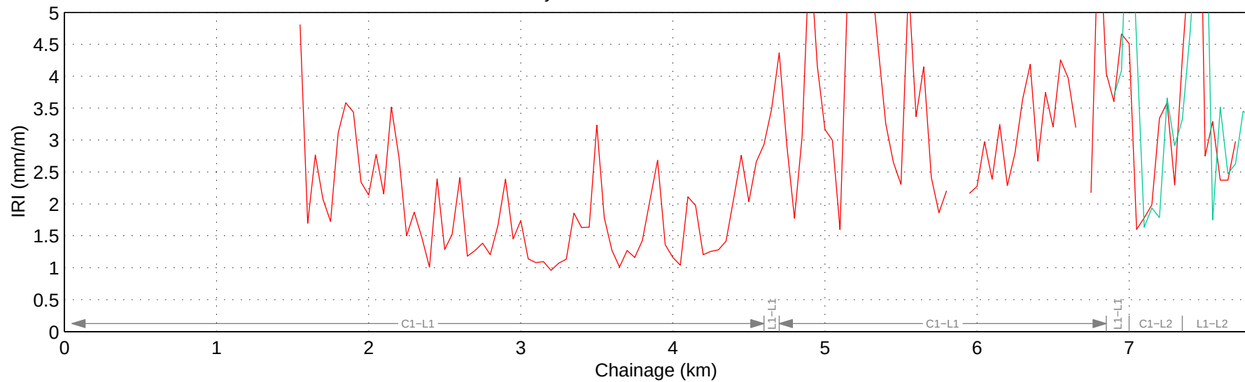
Hwy 742:02 Mean IRI – Right Lane
