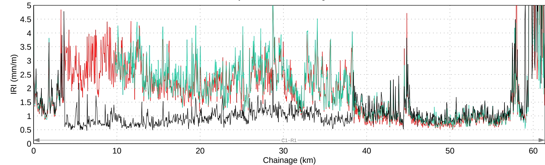
Hwy 744:04 Mean IRI – Right Lane
