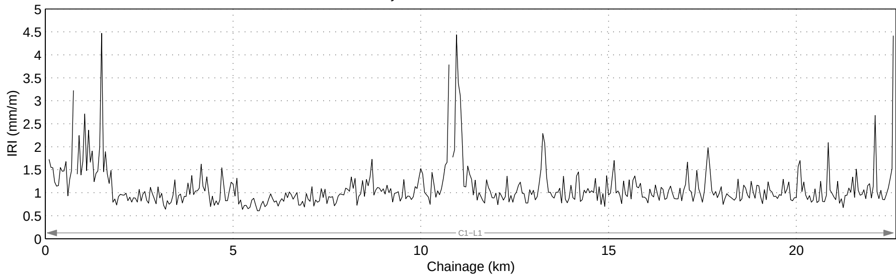
Hwy 748:02 Mean IRI – Right Lane
