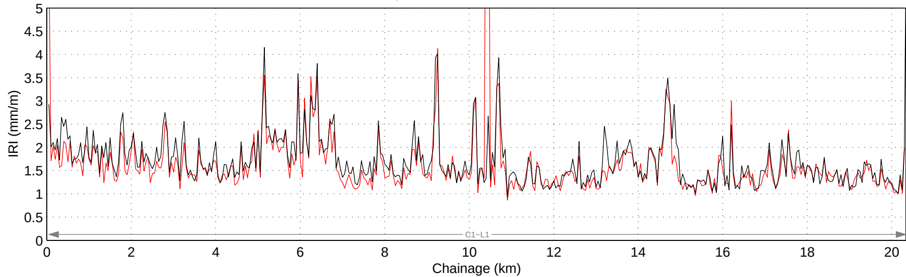
Hwy 771:06 Mean IRI – Right Lane
