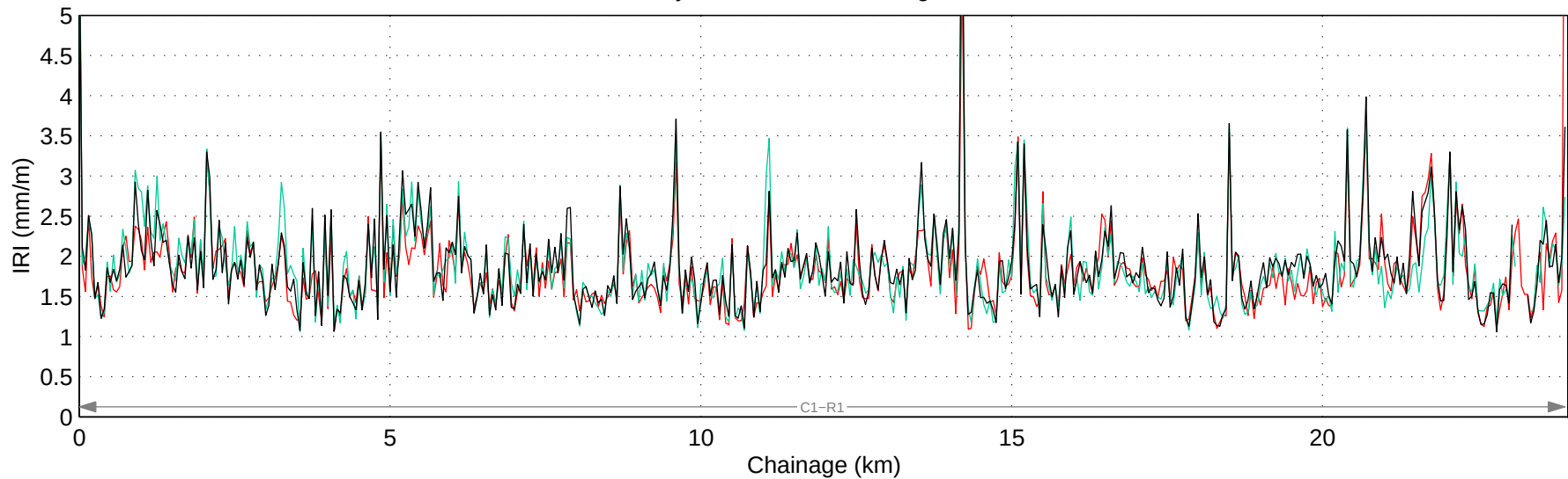
Hwy 723:02 Mean IRI – Right Lane
