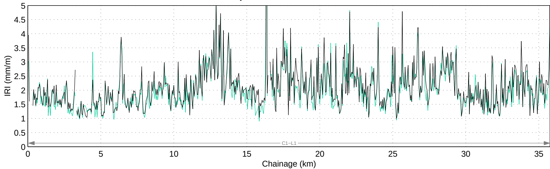
Hwy 766:12 Mean IRI – Right Lane
