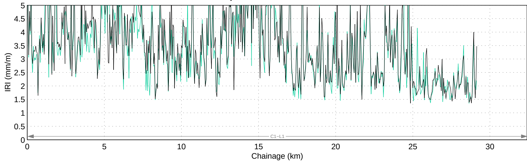
Hwy 766:06 Mean IRI – Right Lane
