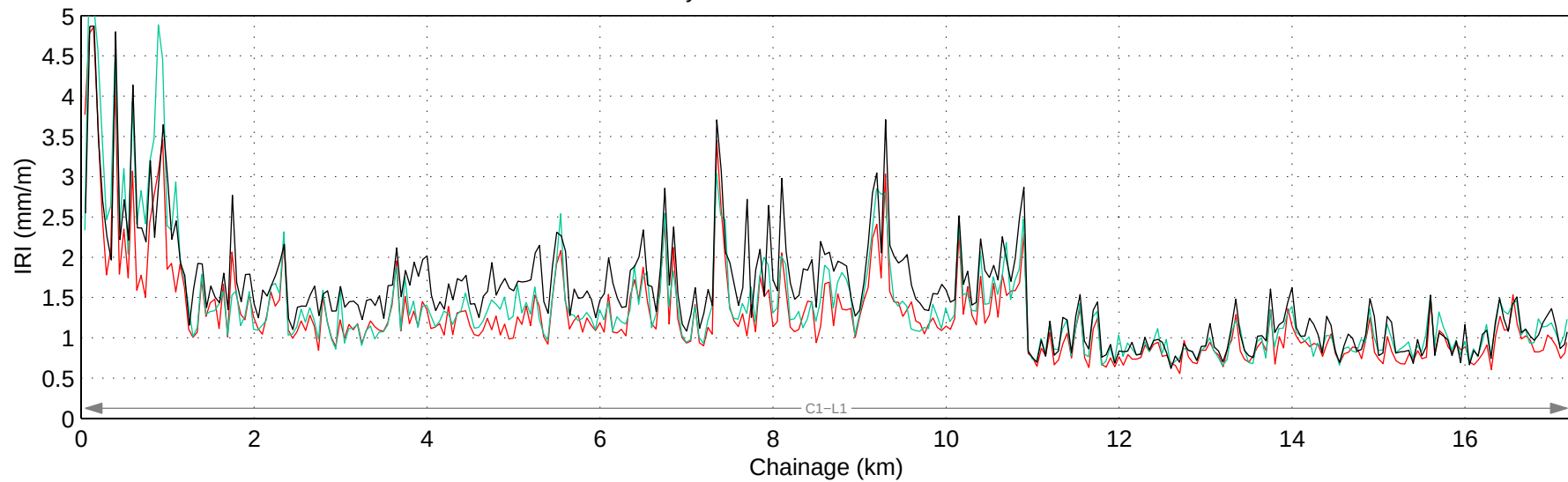
Hwy 732:02 Mean IRI – Right Lane
