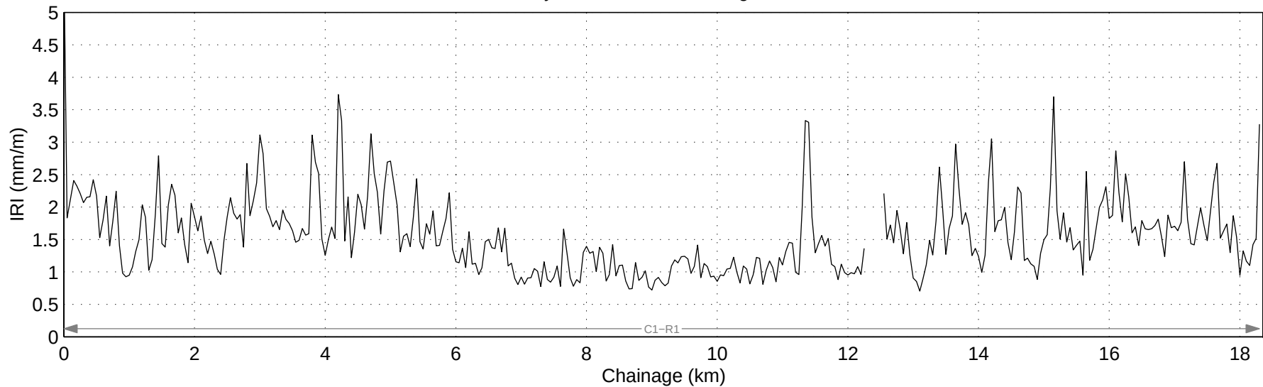
Hwy 759:02 Mean IRI – Right Lane
