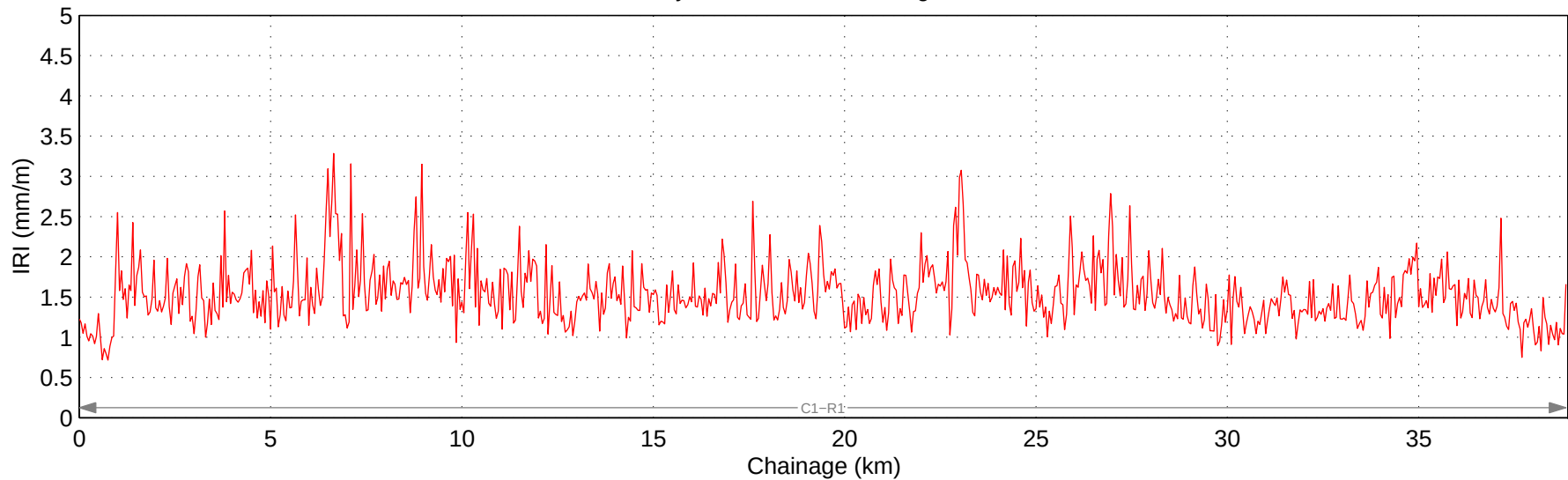
Hwy 750:04 Mean IRI – Right Lane
