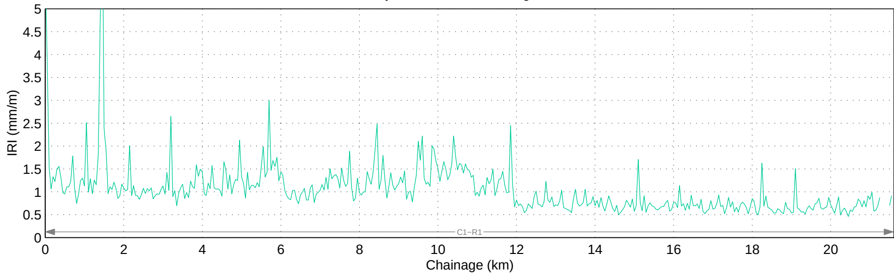
Hwy 771:02 Mean IRI – Right Lane
