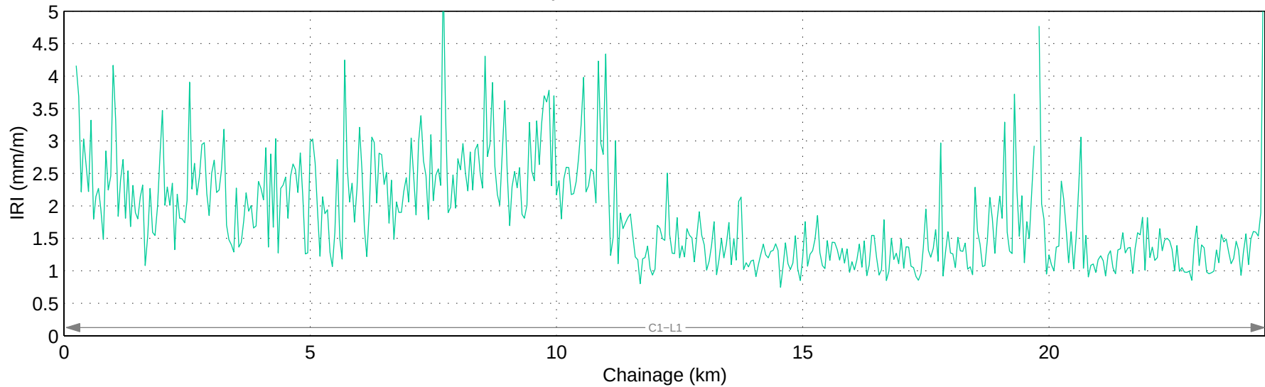
Hwy 770:06 Mean IRI – Right Lane
