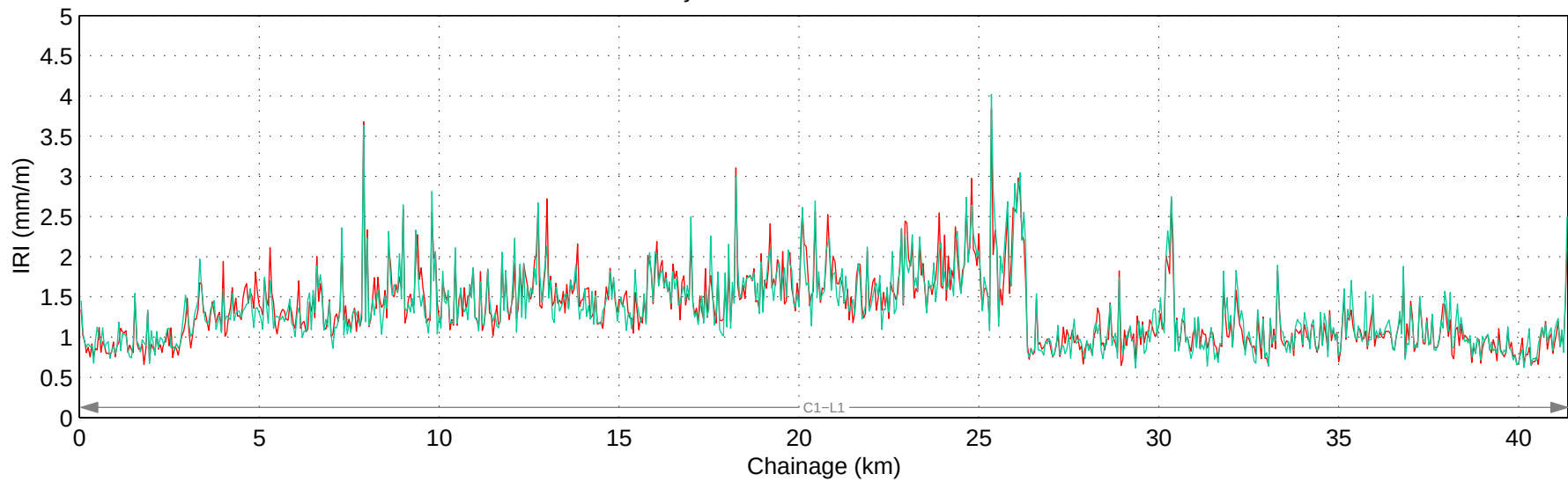
Hwy 747:02 Mean IRI – Right Lane
