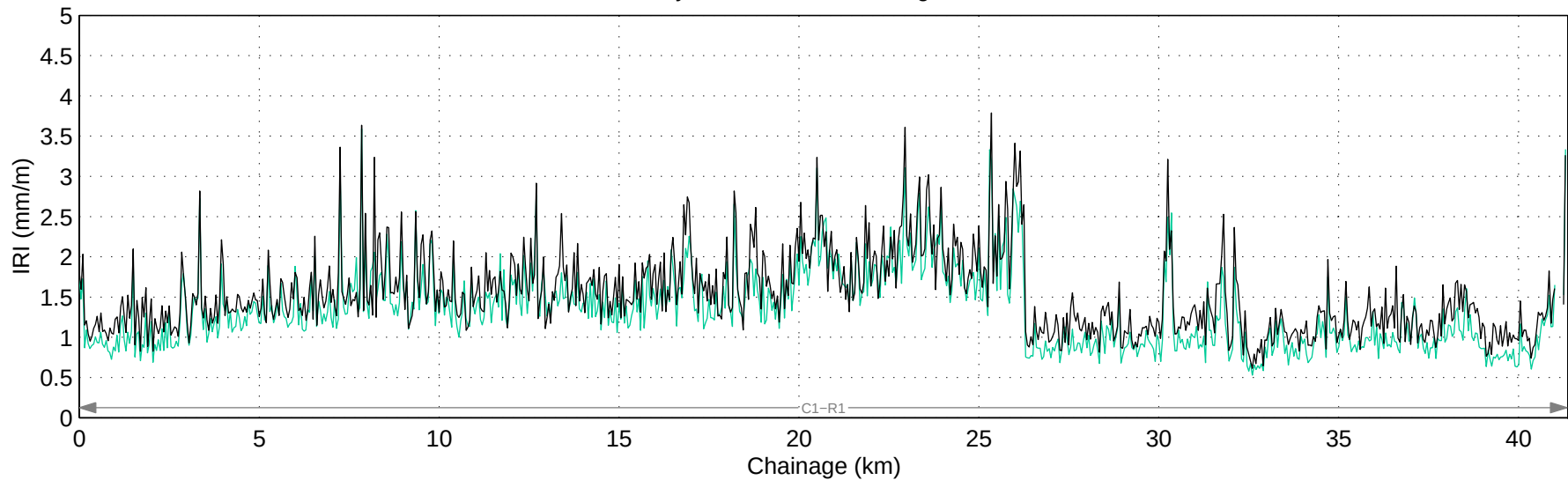
Hwy 747:02 Mean IRI – Right Lane
