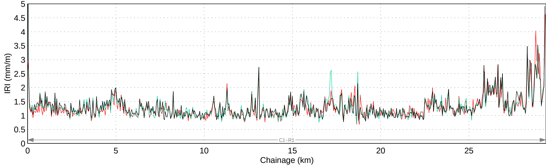
Hwy 769:02 Mean IRI – Right Lane
