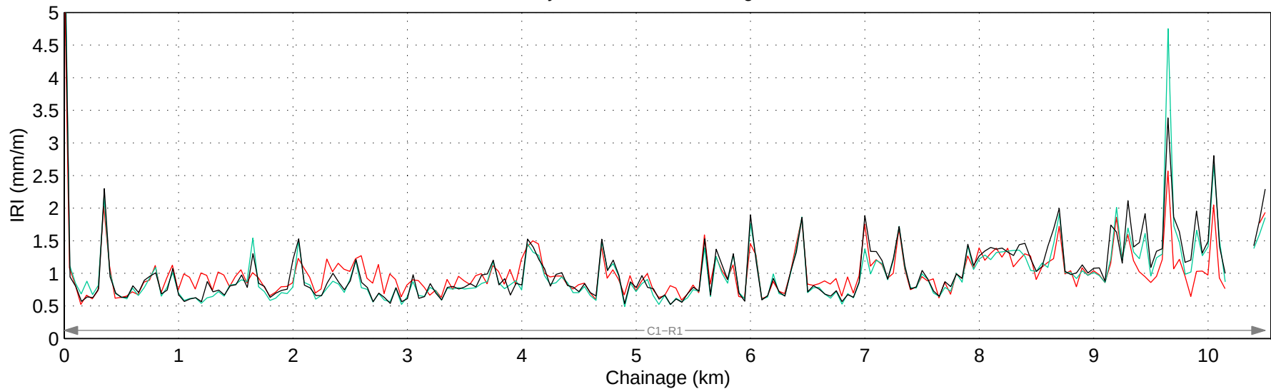
Hwy 777:04 Mean IRI – Right Lane
