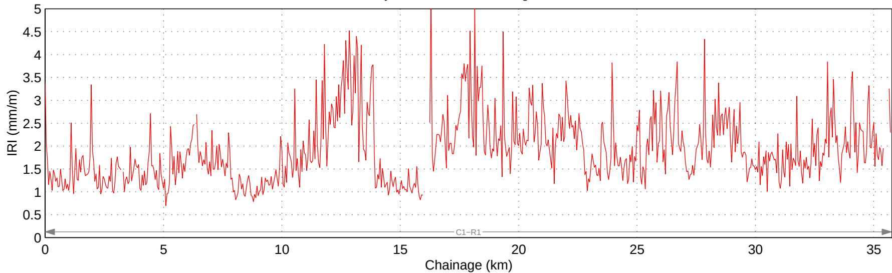
Hwy 766:12 Mean IRI – Right Lane
