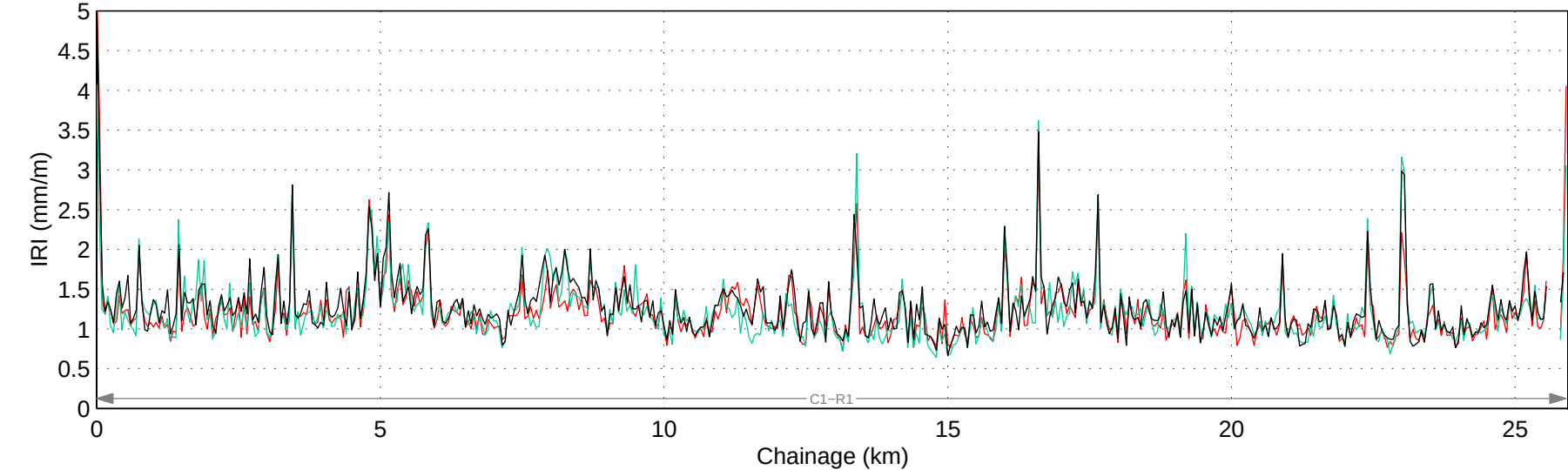
Hwy 766:10 Mean IRI – Right Lane
