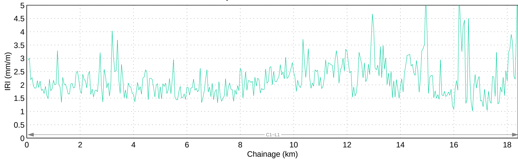
Hwy 778:02 Mean IRI – Right Lane
