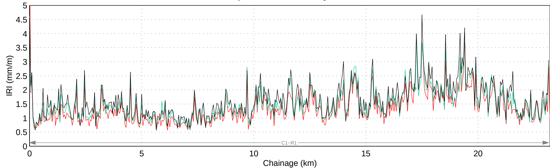
Hwy 725:02 Mean IRI – Right Lane
