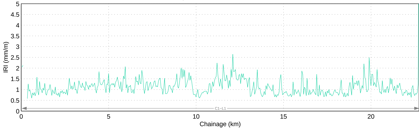
Hwy 792:02 Mean IRI – Right Lane
