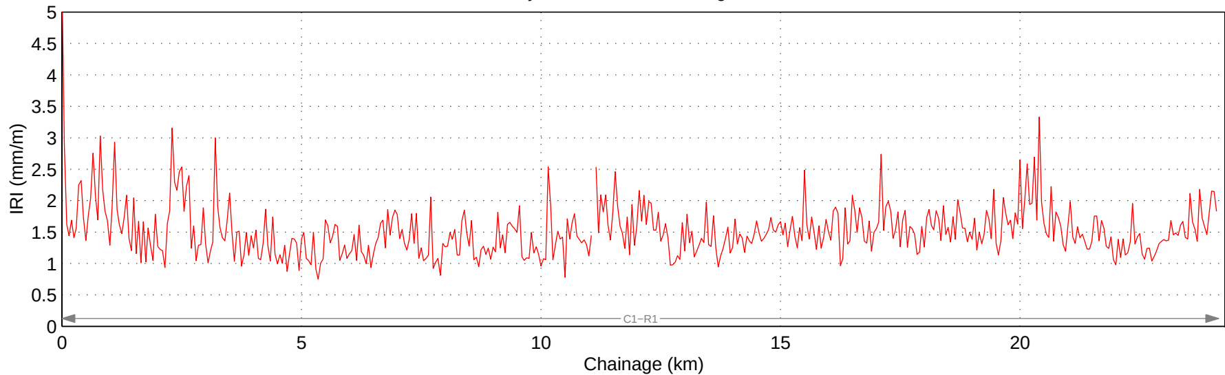
Hwy 765:02 Mean IRI – Right Lane
