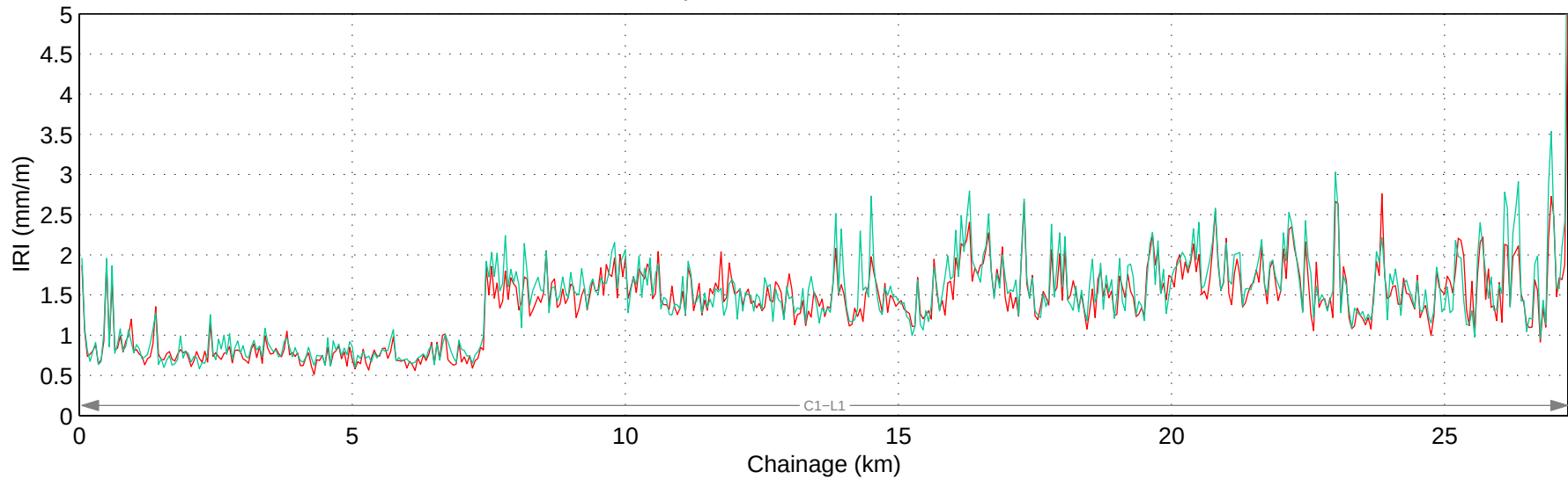
Hwy 749:02 Mean IRI – Right Lane
