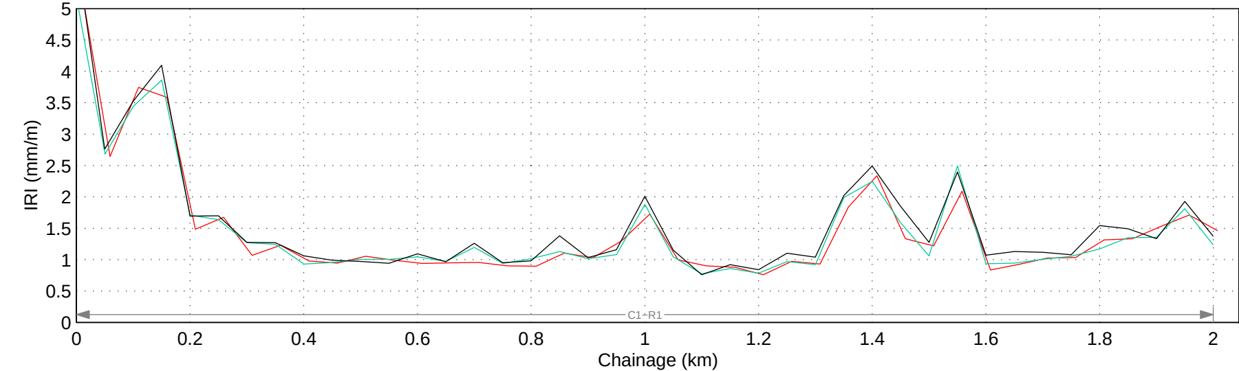
Hwy 795:02 Mean IRI – Right Lane
