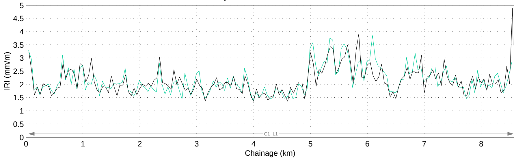
Hwy 780:02 Mean IRI – Right Lane
