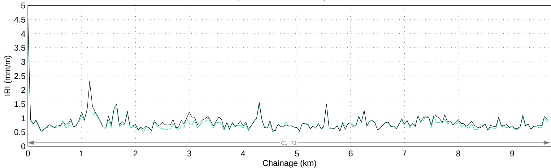
Hwy 777:01 Mean IRI – Right Lane
