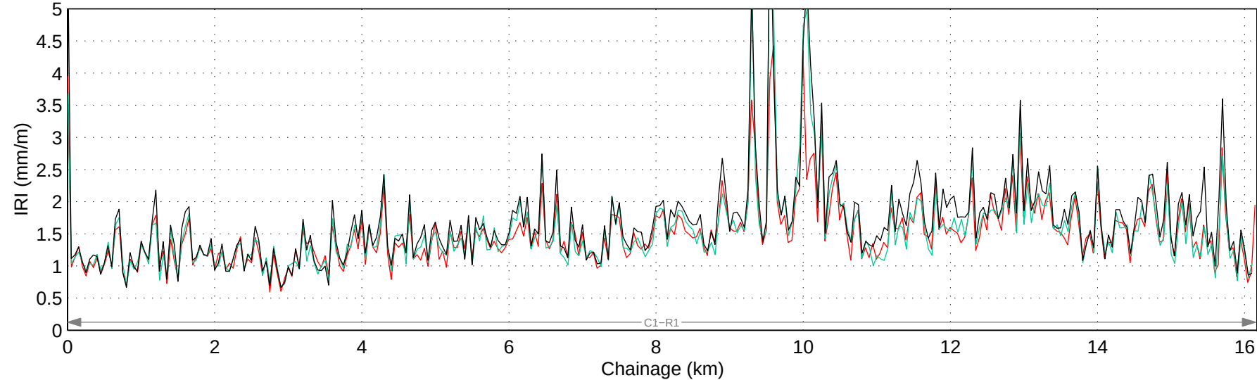
Hwy 726:02 Mean IRI – Right Lane
