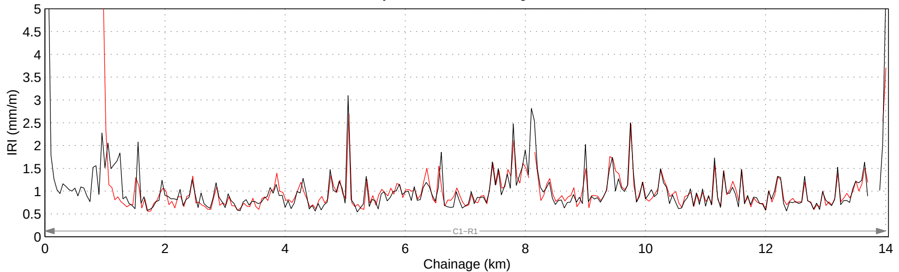
Hwy 757:04 Mean IRI – Right Lane
