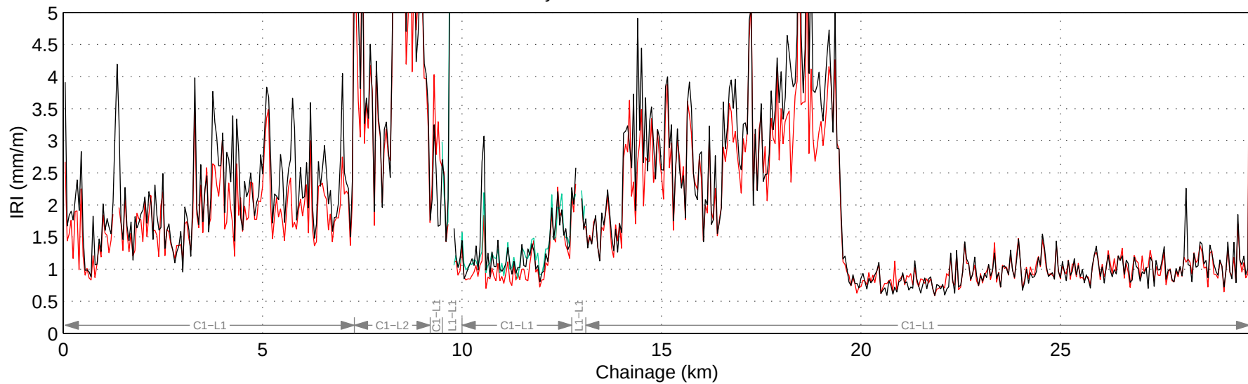
Hwy 779:02 Mean IRI – Right Lane
