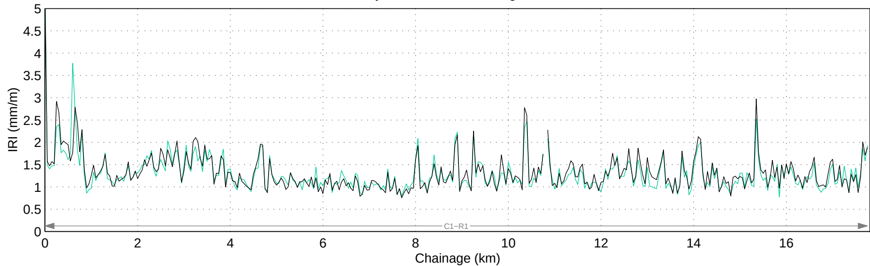
Hwy 749:04 Mean IRI – Right Lane
