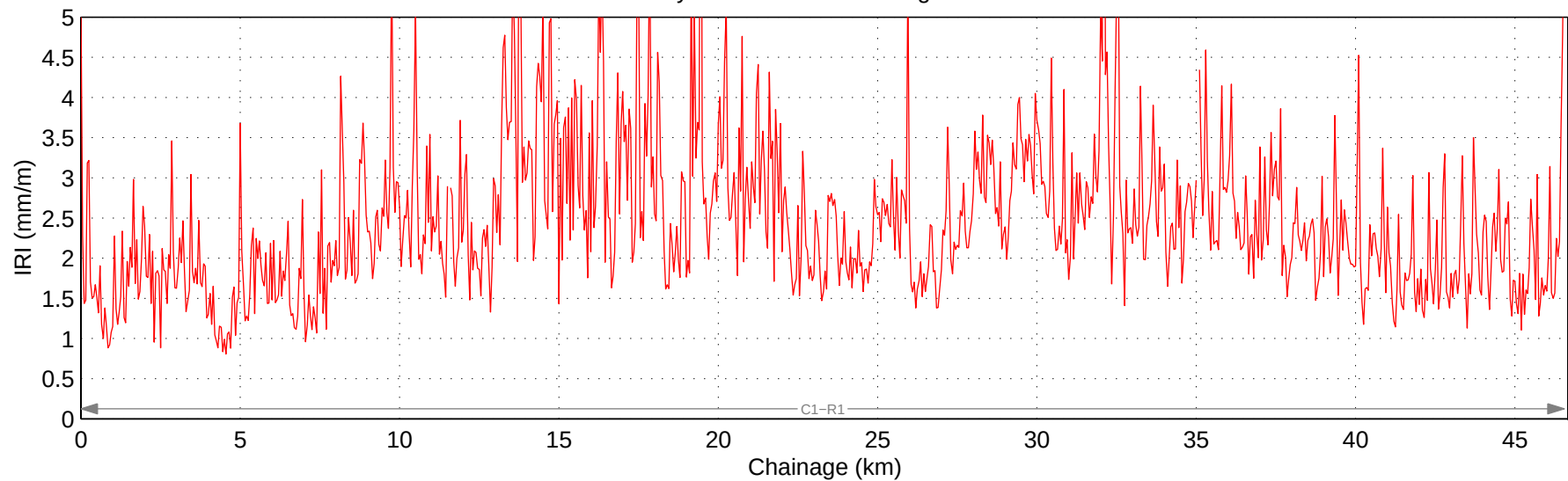
Hwy 791:06 Mean IRI – Right Lane
