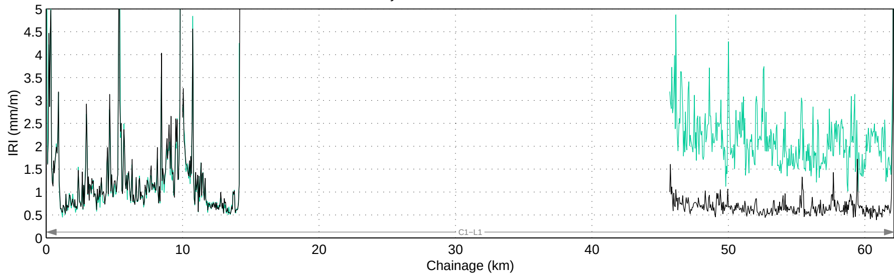
Hwy 785:02 Mean IRI – Right Lane
