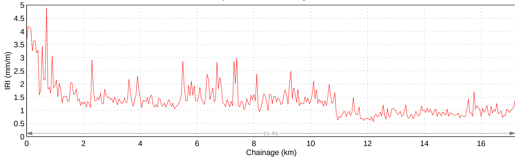
Hwy 732:02 Mean IRI – Right Lane
