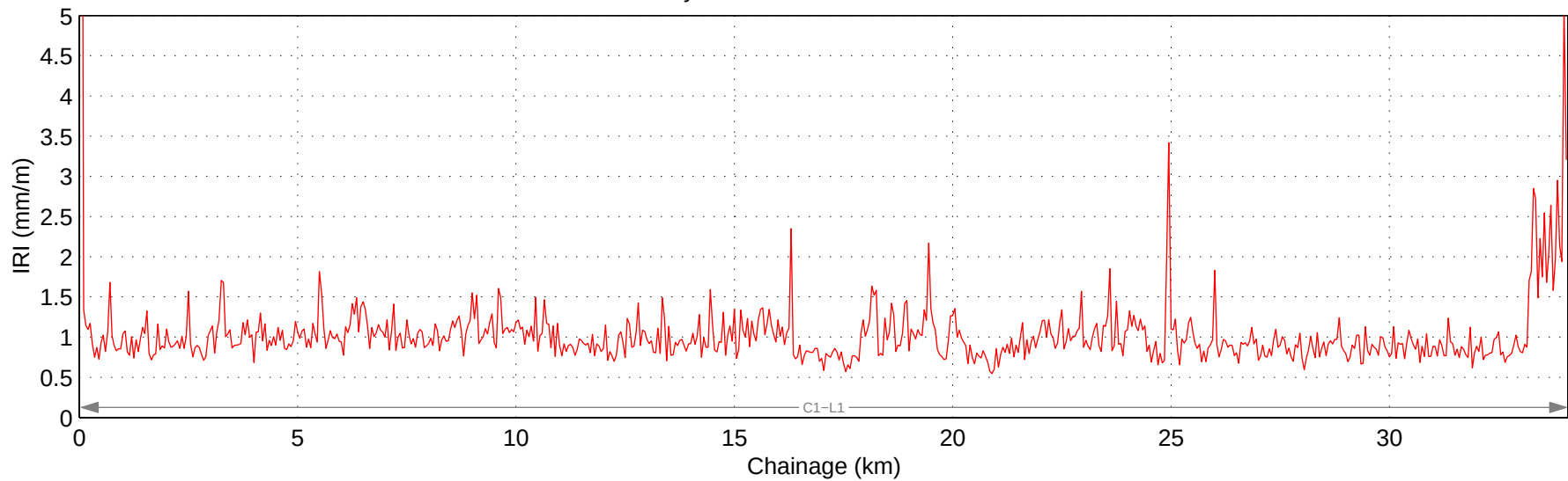
Hwy 795:06 Mean IRI – Right Lane
