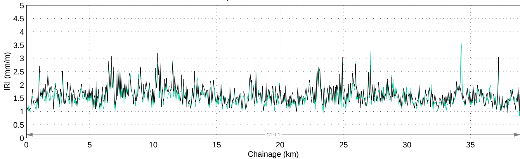
Hwy 750:04 Mean IRI – Right Lane
