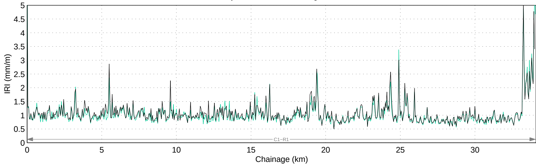
Hwy 795:06 Mean IRI – Right Lane
