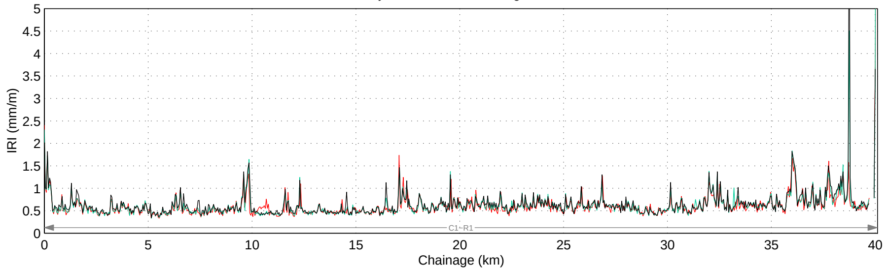
Hwy 901:48 Mean IRI – Right Lane
