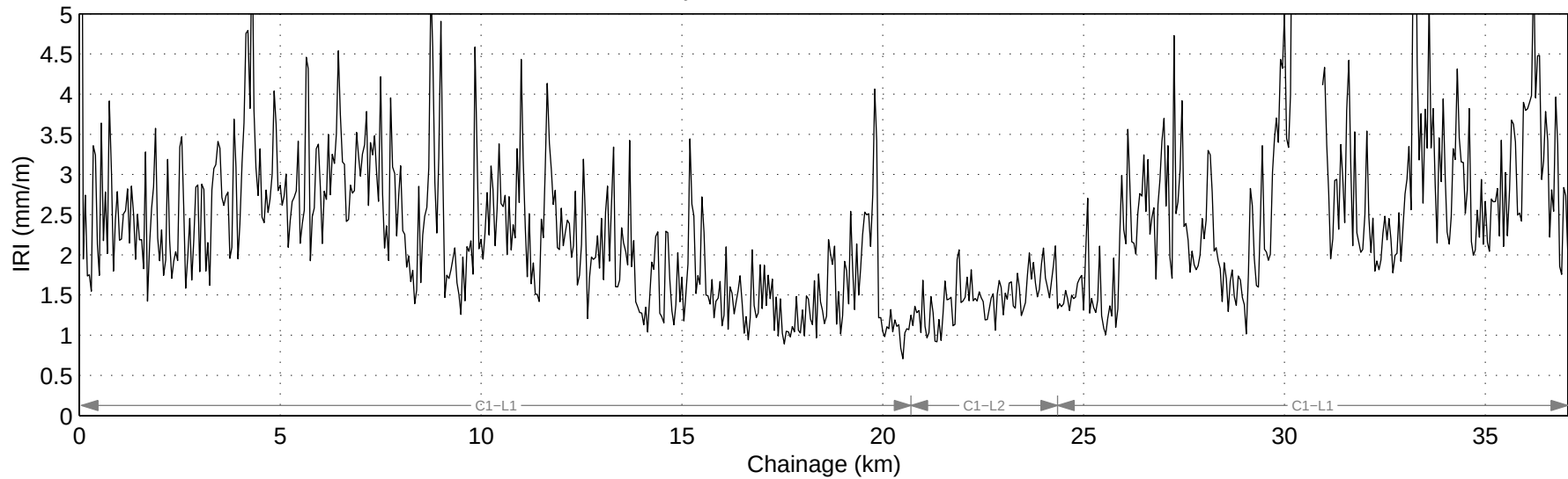
Hwy 986:01 Mean IRI – Right Lane
