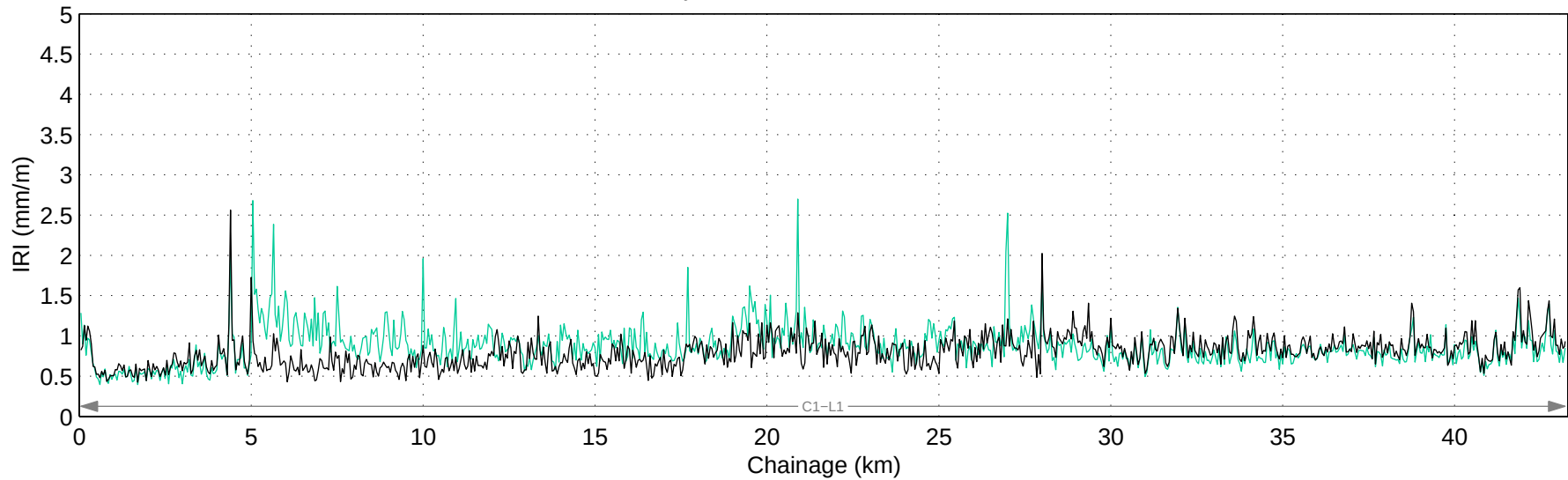
Hwy 986:04 Mean IRI – Right Lane
