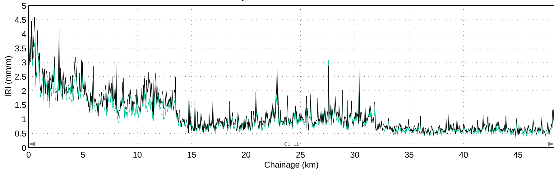
Hwy 986:02 Mean IRI – Right Lane
