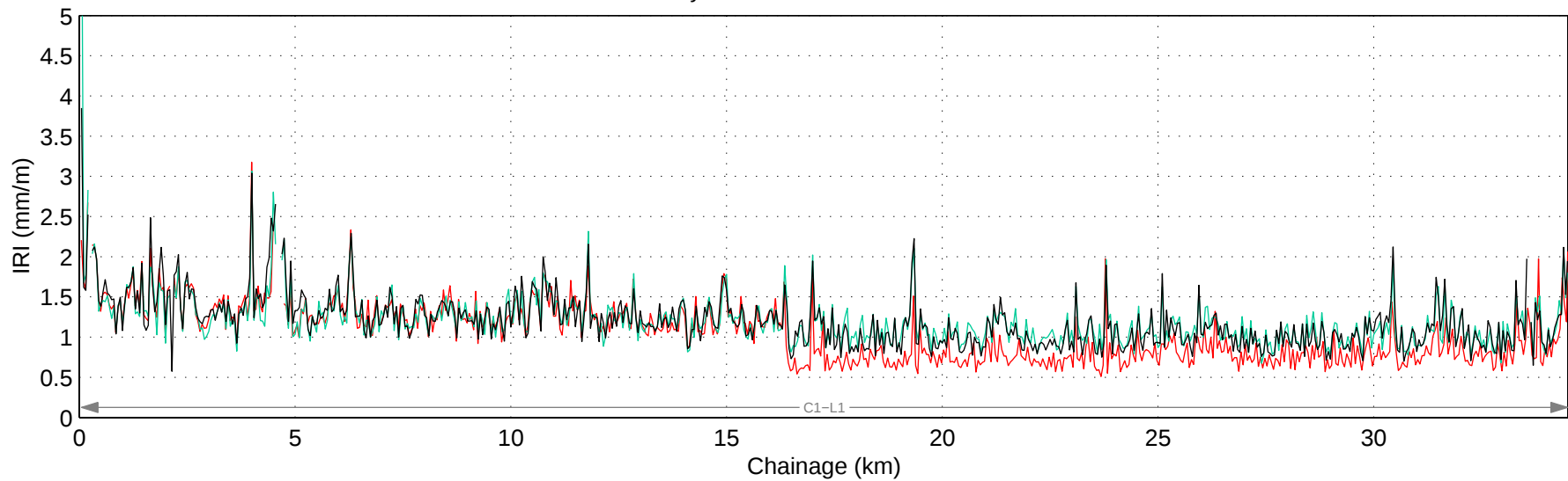
Hwy 88:02 Mean IRI – Right Lane
