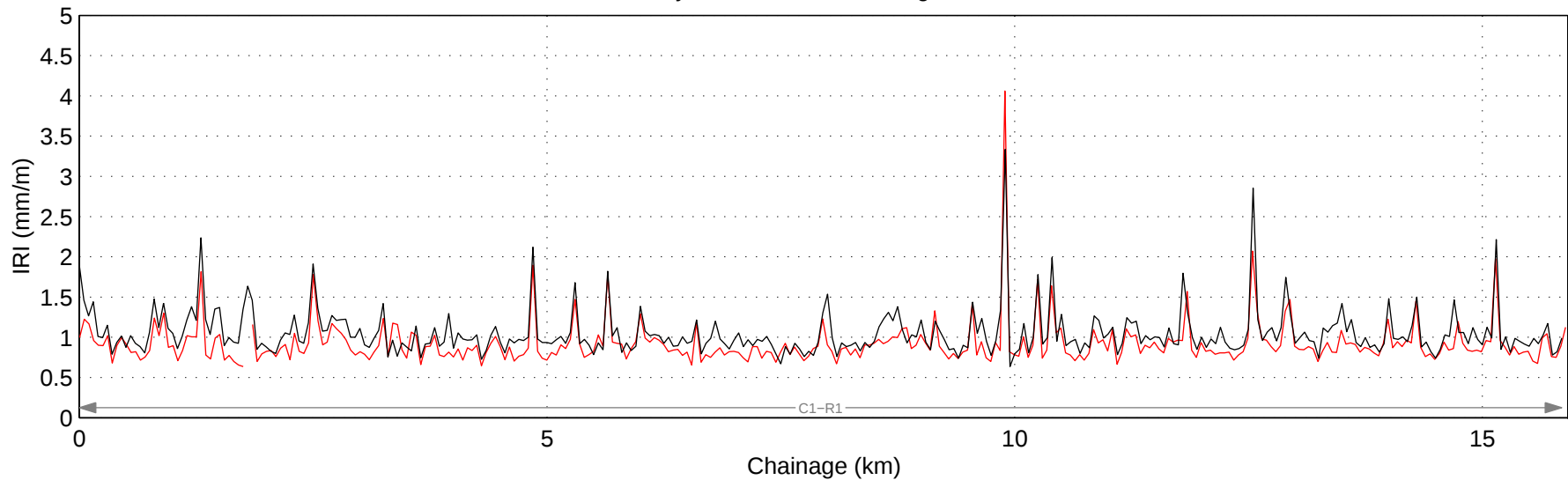
Hwy 747:01 Mean IRI – Right Lane
