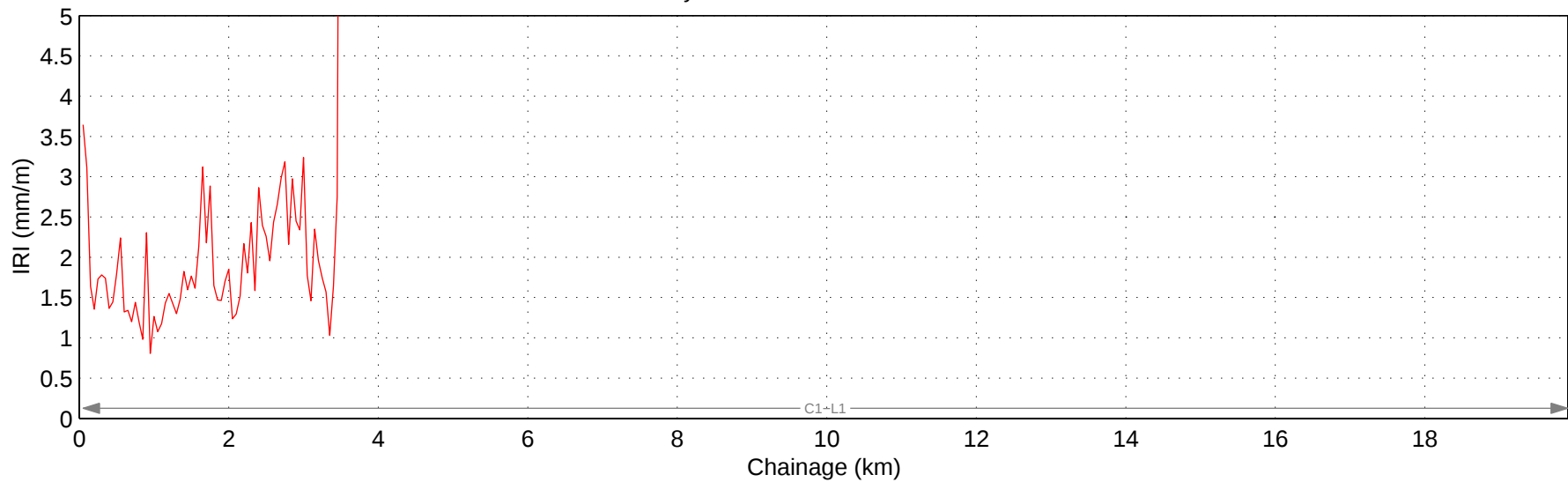
Hwy 727:02 Mean IRI – Right Lane
