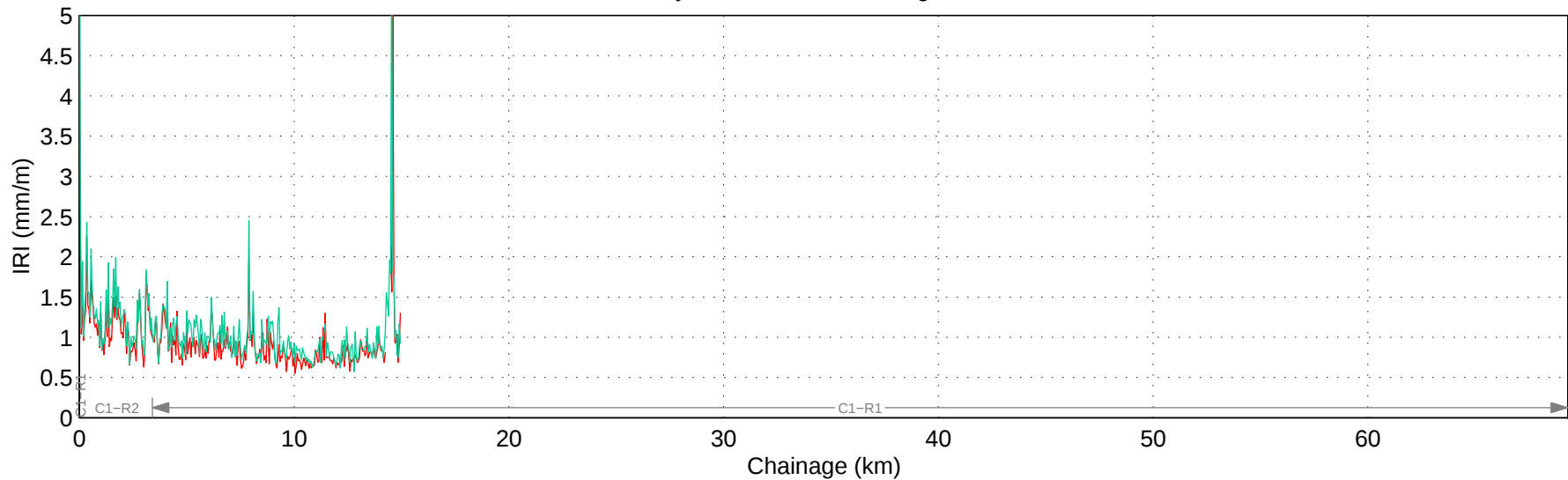
Hwy 743:02 Mean IRI – Right Lane
