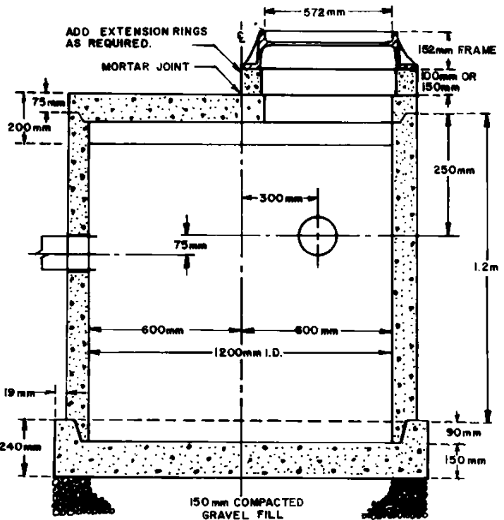
PRECAST REINFORCED CONCRETE MANHOLE
