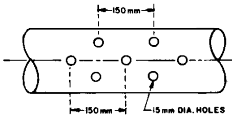
PERFORATED PIPE
