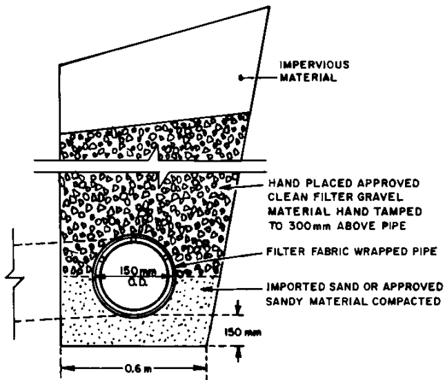
CLASS "B" BEDDING
