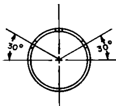
PERFORATED PIPE SECTION
