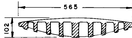
SECTION B-B
