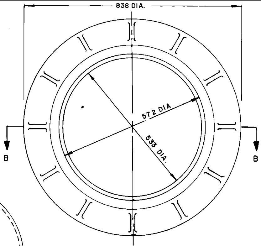
FRAME - PLAN VIEW
