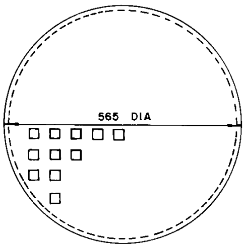
COVER - PLAN VIEW
