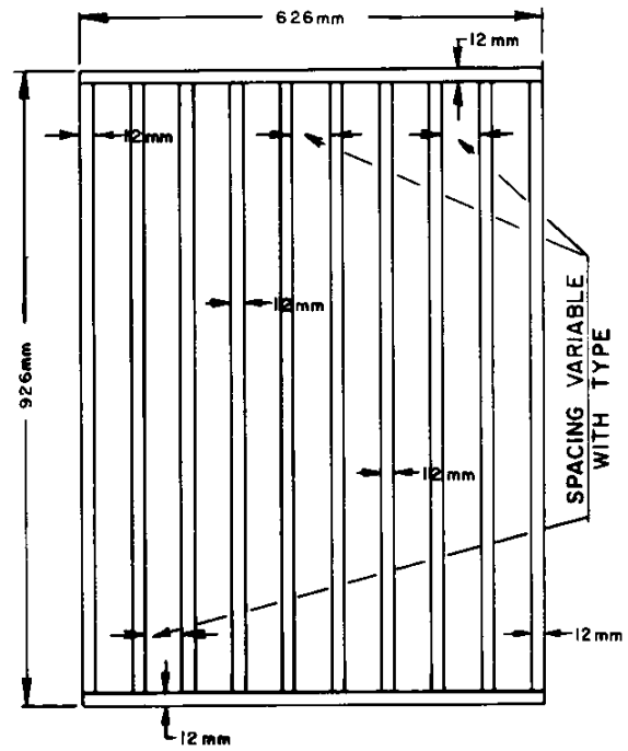
WELDED GRATE
