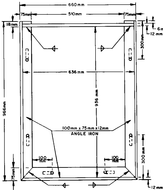
WELDED GRATE FRAME
