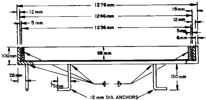
LONGITUDINAL SECTION THROUGH FRAME AND GRATE
