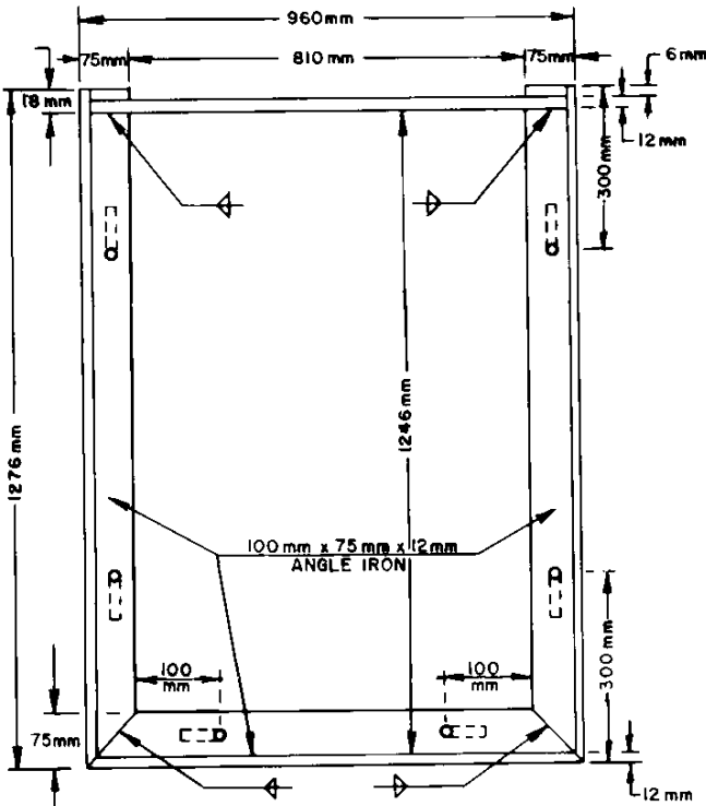
WELDED FRAME FOR GRATE
