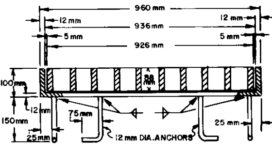
CROSS - SECTION THROUGH FRAME AND GRATE
