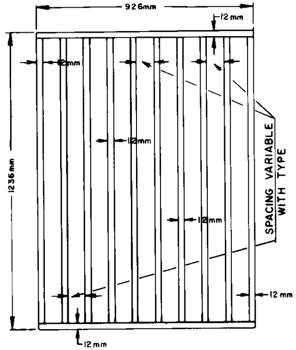
WELDED GRATE
