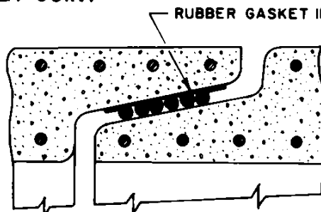
COMPLETED RUBBER GASKET JOINT
