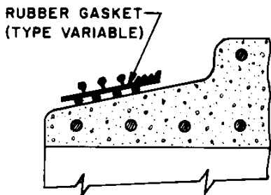
RUBBER GASKET IN POSITION ON TONGUE
