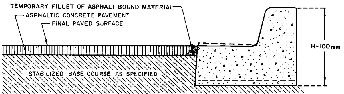
INTERMEDIATE SECTION
