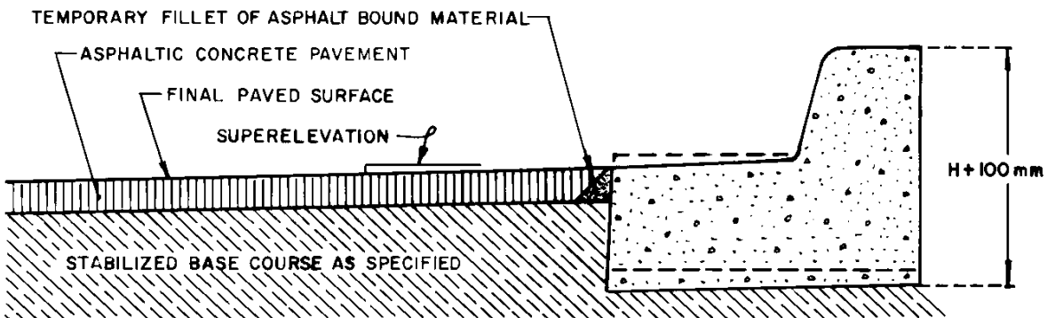
REVERSED SECTION
