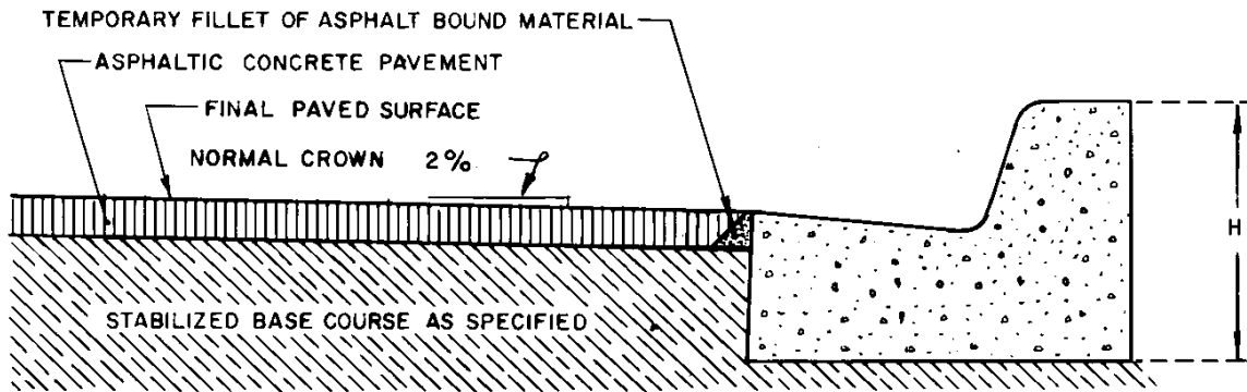
NORMAL SECTION
