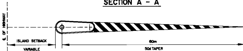
SIGN ISLAND LOCATION AND PAVEMENT MARKING
