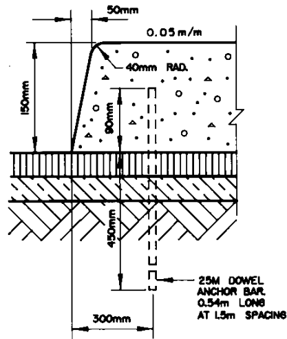
CURB DETAIL
