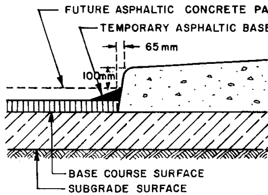
ASPHALTIC BASE COURSE FILLET DETAIL
