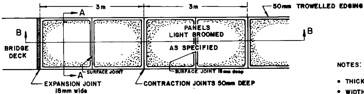
PLAN VIEW
