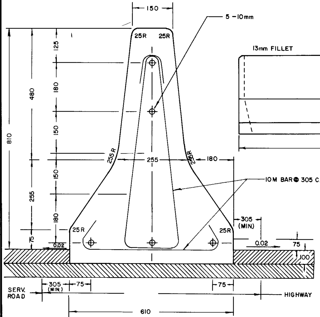
SECTION A-A VIEW
