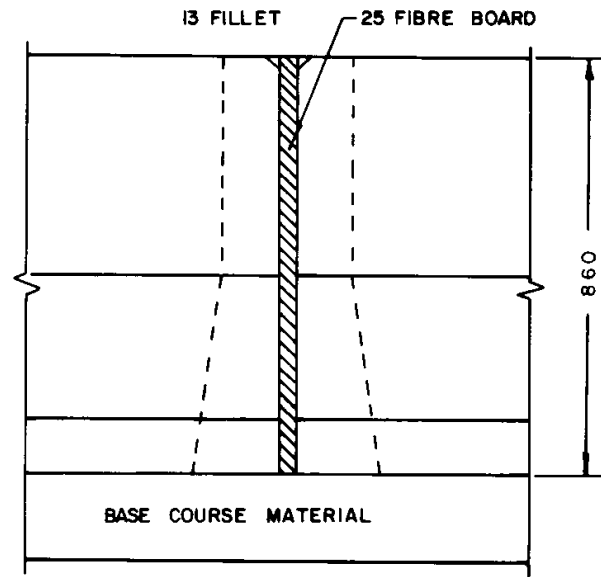
EXPANSION JOINT SIDE VIEW
