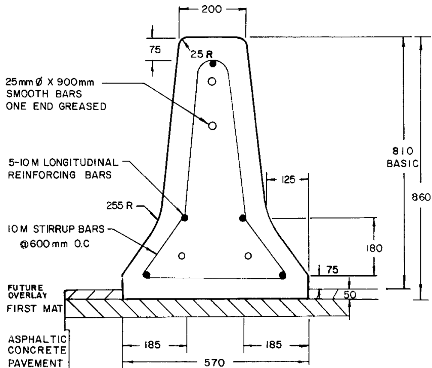
CROSS SECTION
