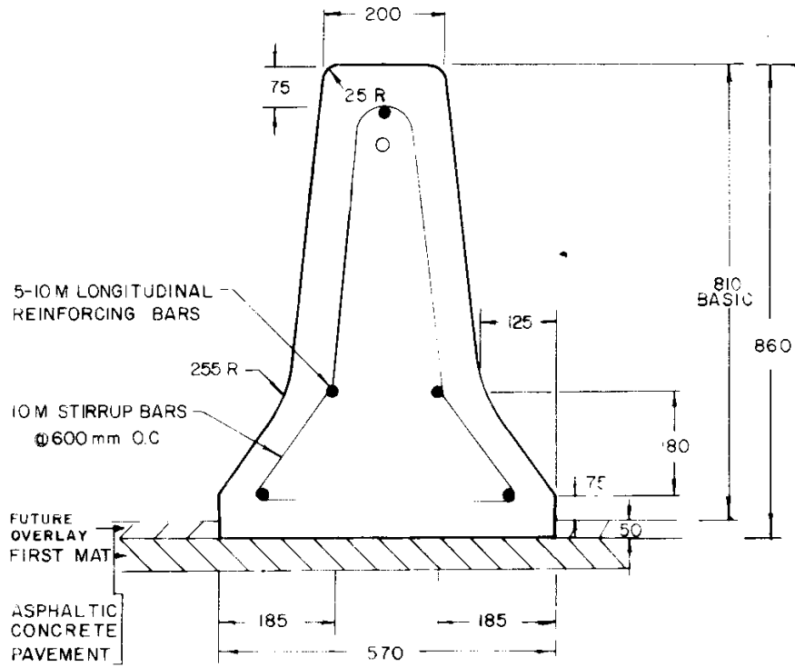
CROSS SECTION
