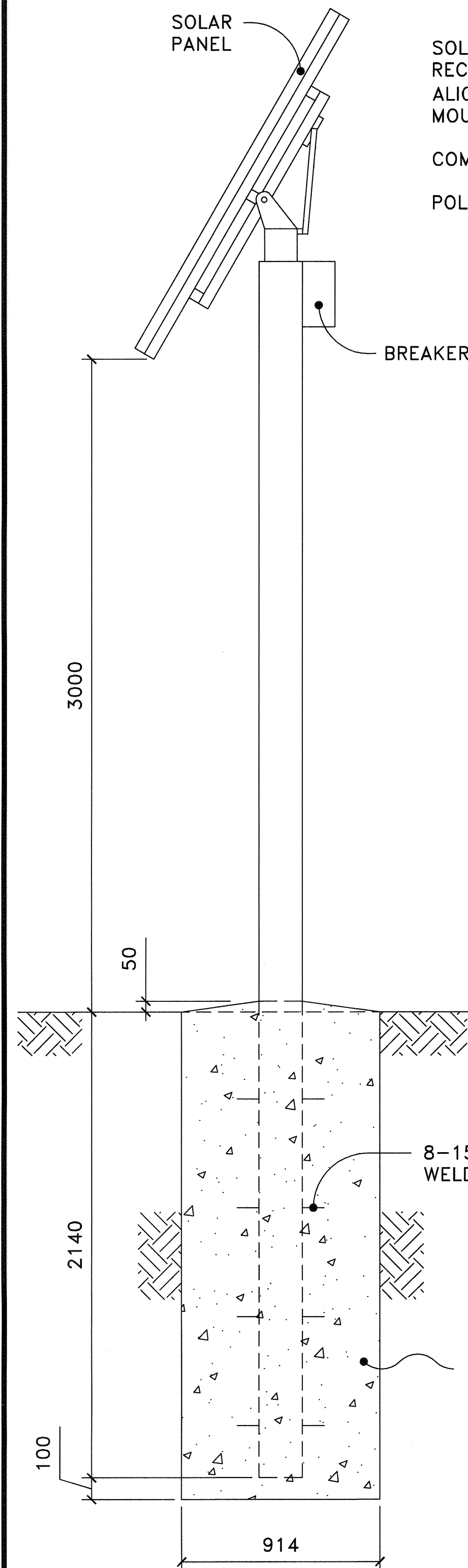
SOLAR POWER POLE DETAIL
