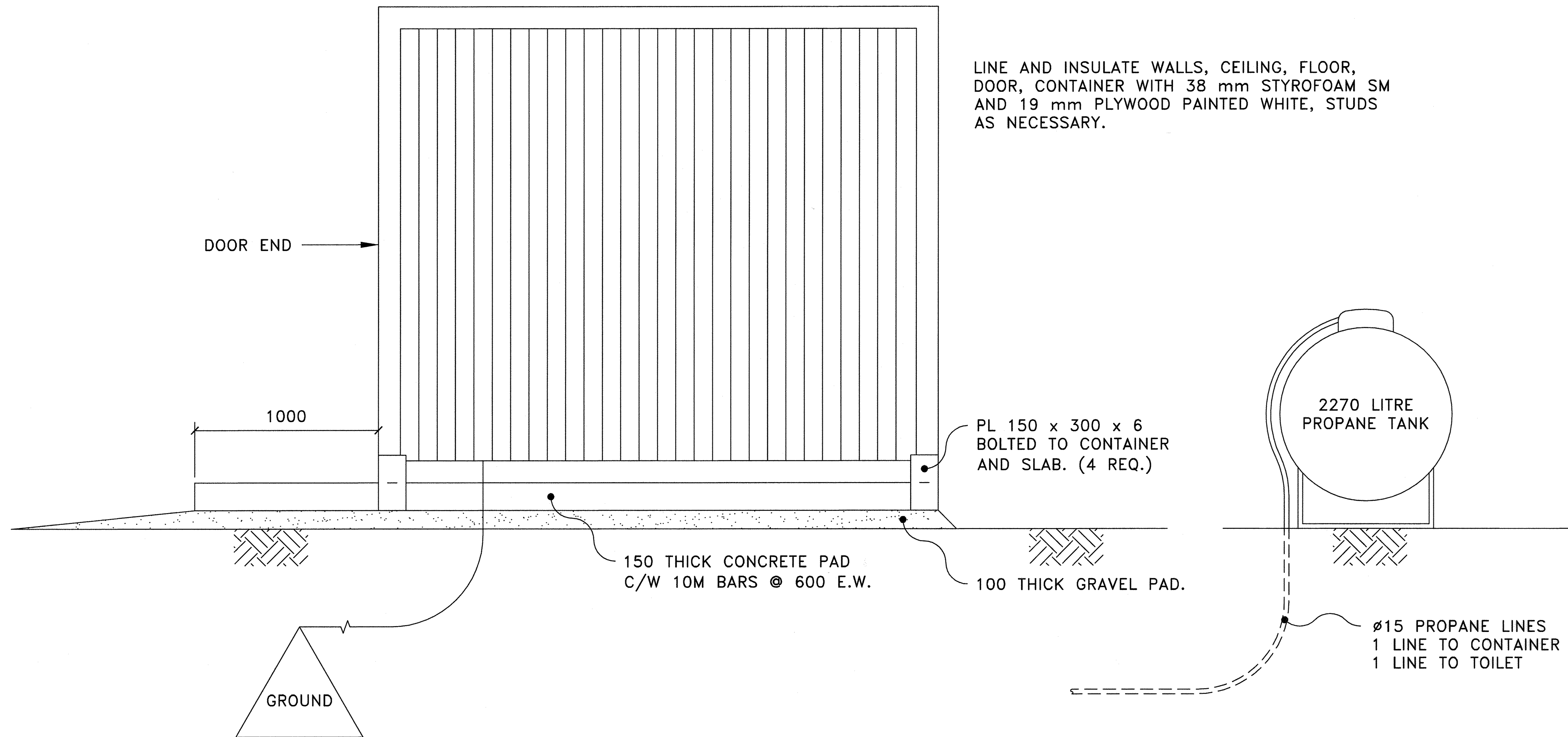
TOILET SOLAR POWER CONTAINER SIDE ELEVATION
