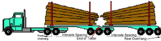
Diagram 2 - Tandem Drive-Double Pole B-Train– No Hinge
