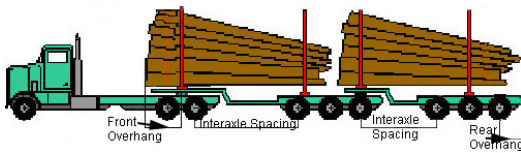
Diagram 2 - Tandem Drive-Double Pole B-Train– No Hinge
