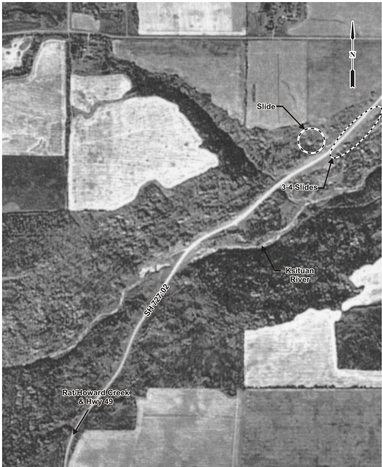
Figure 1 Site Plan
