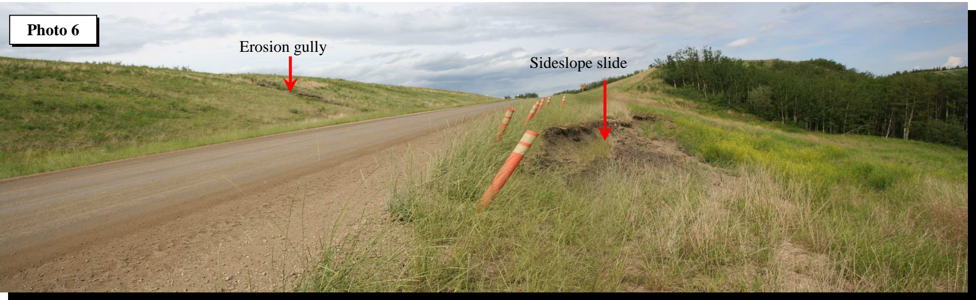
Looking upgrade north (away from Hwy. 49 Jct.) - Sideslope slides (right) has encroached to shoulder of northbound lane - Erosion gully formed at backslope (left) as a result of runoff from upland farm area
