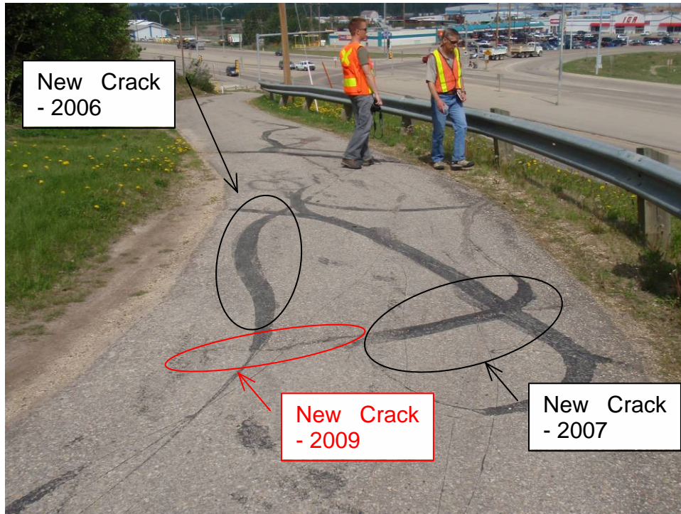
Photo 9 – Closer view of new crack to south of existing cracks (June 15, 2009).
