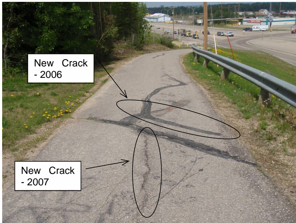
Photo 10 – Closer view of new crack to between existing cracks (June 15, 2009).
