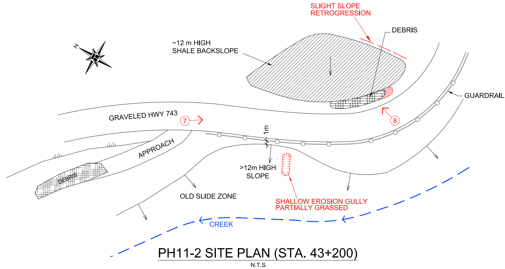
SITE MAP NOT TO SCALE
