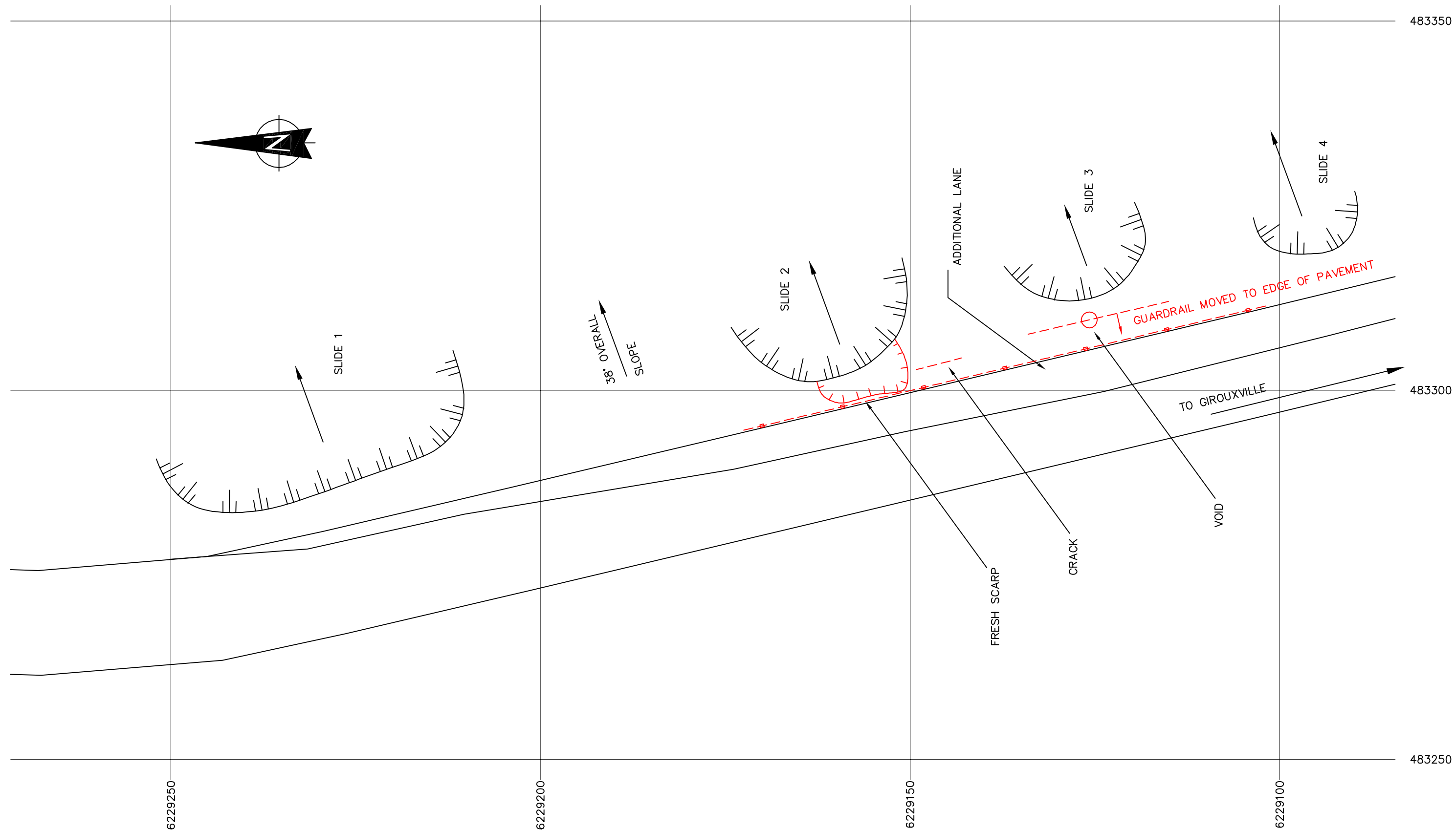
FIGURE PH12-2A PH12 JUDAH HILL HEART RIVER SLIDES SITE PLAN PEACE REGION (PEACE RIVER/HIGH LEVEL)
