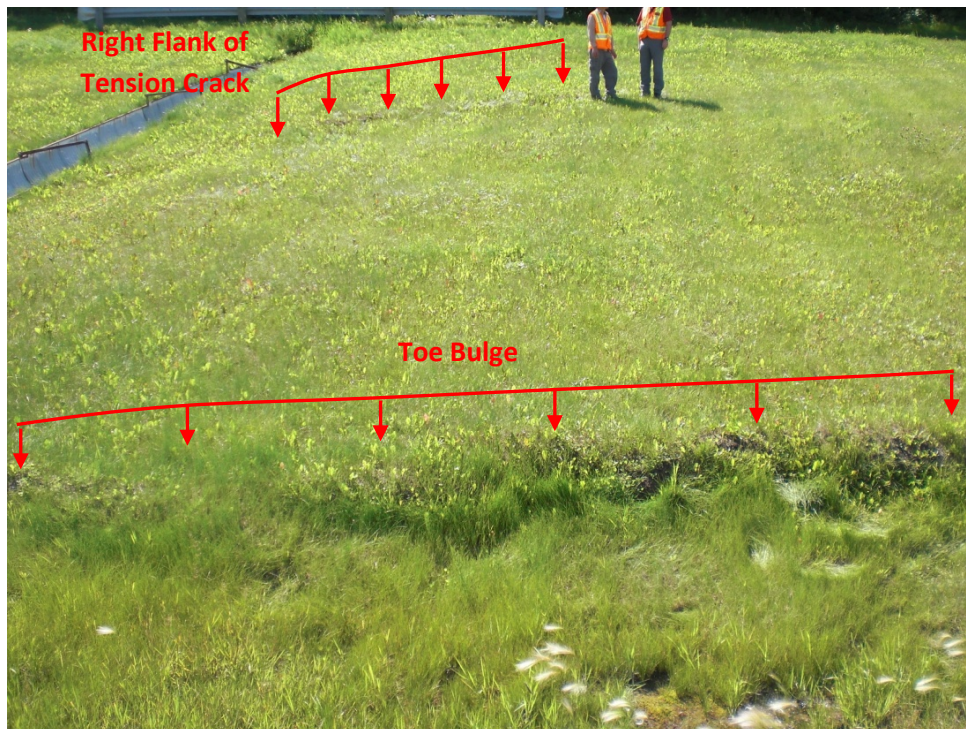
Photo 2: Tension crack and toe bulge, south of Highway 43.
