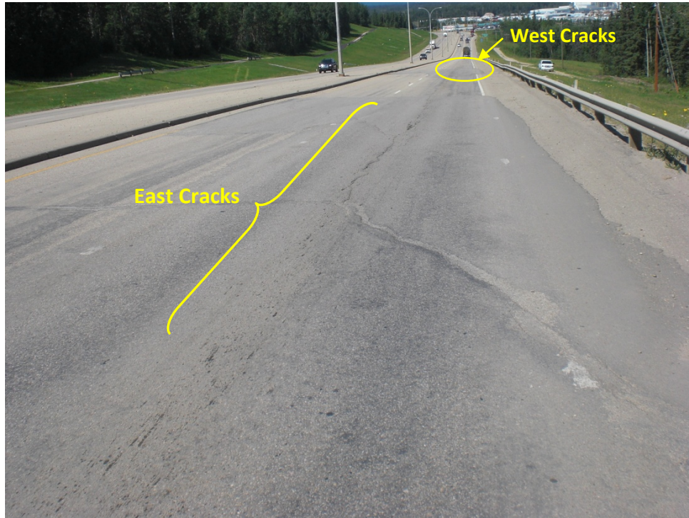
Photo 1: East crack (note west crack in distance).
