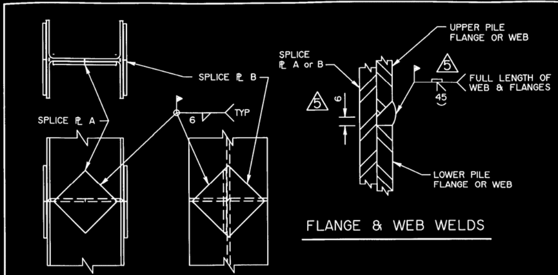
SPLICE DETAILS
