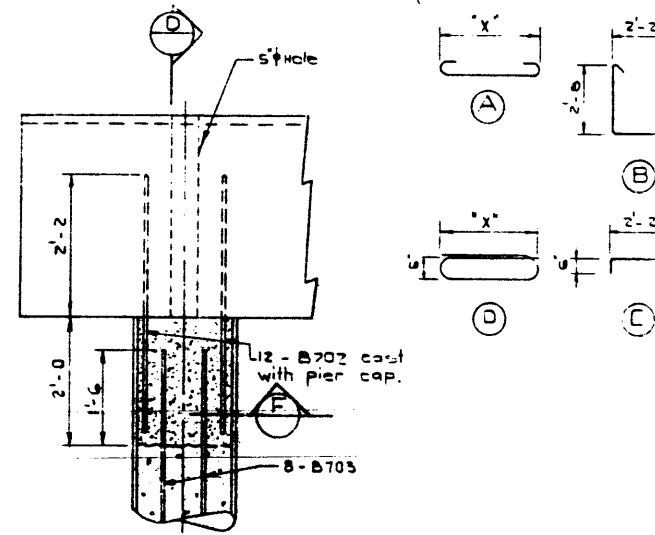
PART ELEVATION
