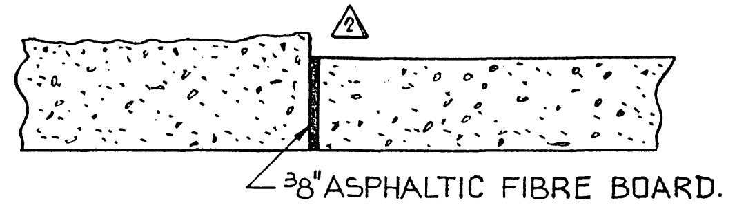
TYPE 1 JOINT
