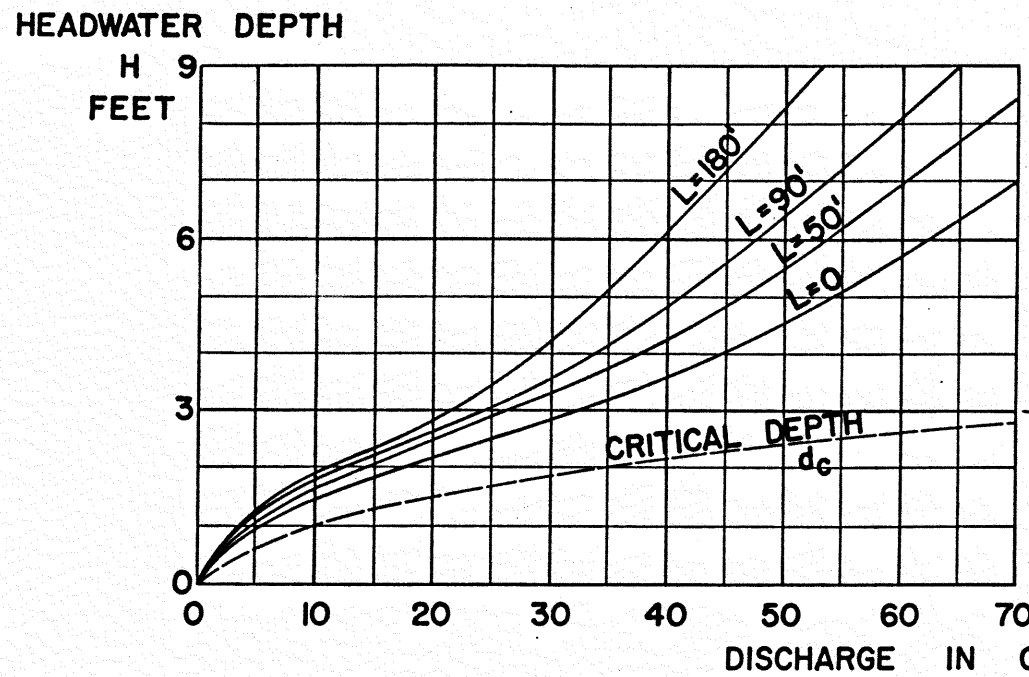
36" DIA; SLOPE 0
