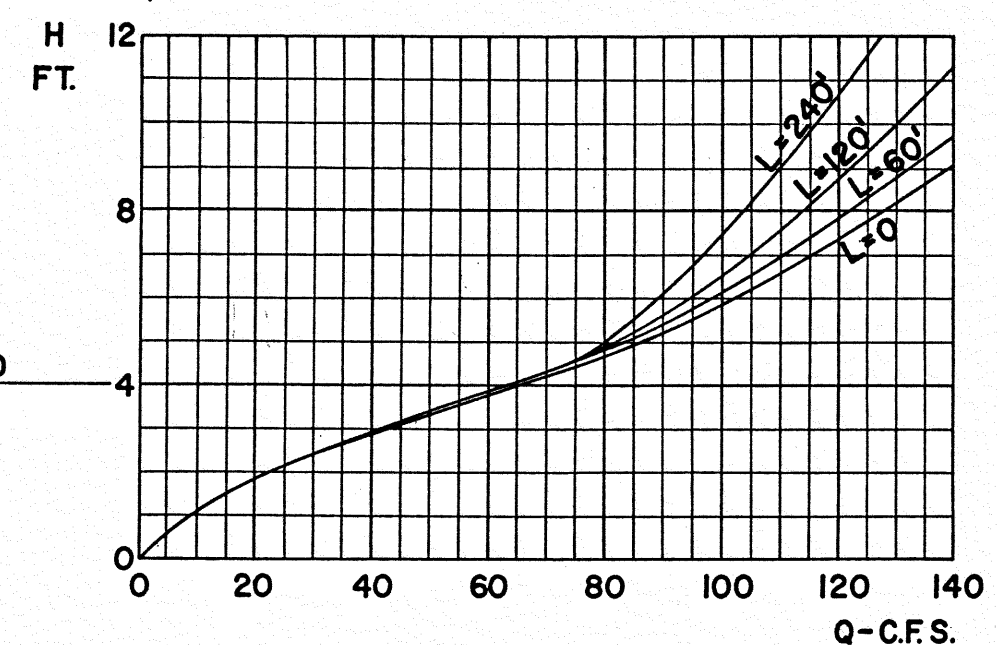
48" DIA; SLOPE 1%
