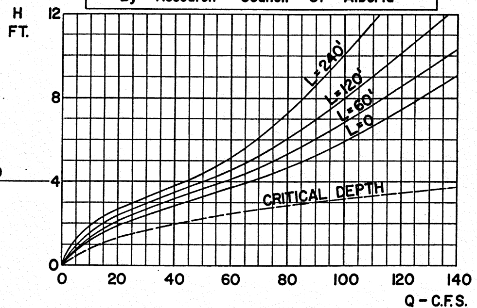
48" DIA; SLOPE 0
