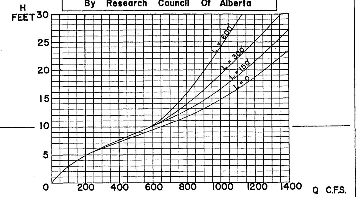
(b) SLOPE 1%
