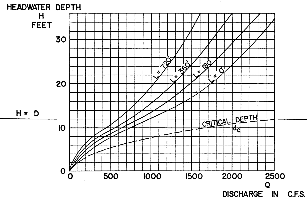
(a) SLOPE 0
