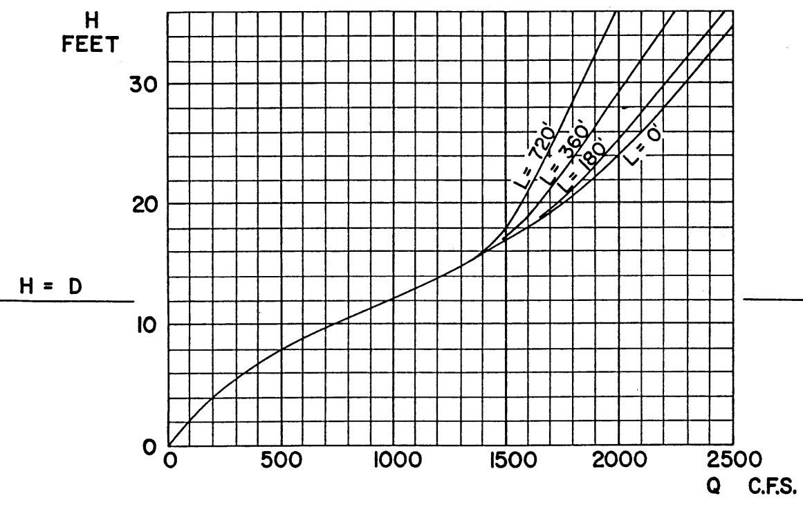
(c) SLOPE 2%
