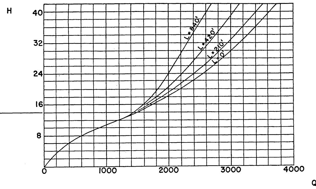
(b) SLOPE 1%
