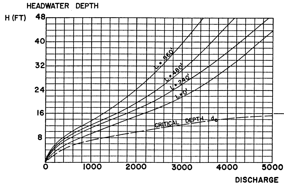
(a) SLOPE 0%
