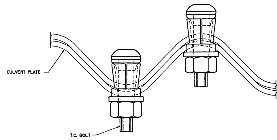
TYPICAL FIELD ASSEMBLY 1:1
