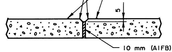
JOINT TYPE 2
