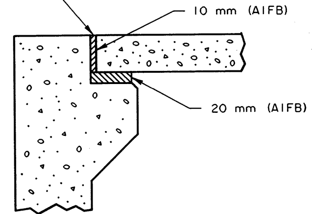
JOINT TYPE 3
