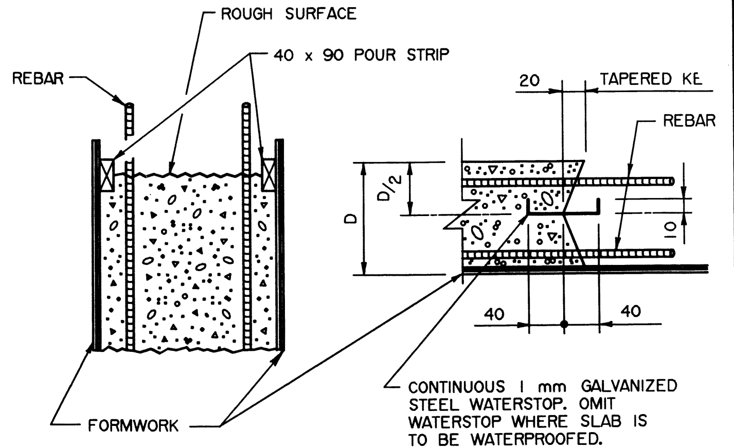
SLAB DETAIL
