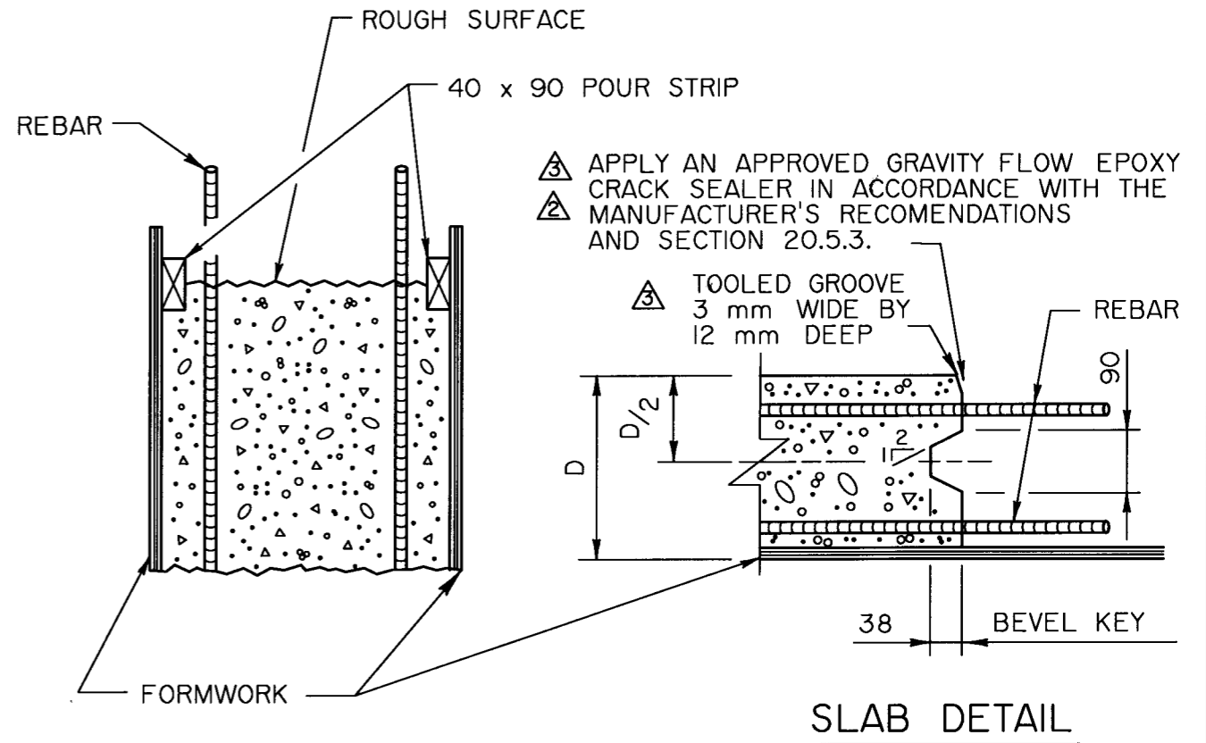
WALL OR PIER SHAFT DETAIL
