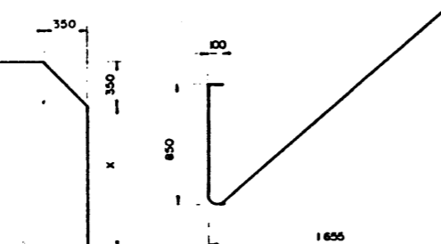
BAR TYPES NOTE: ALL BAR DIMENSIONS ARE OUT TO OUT
