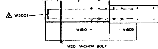
C SECTION SCALE 1/20
