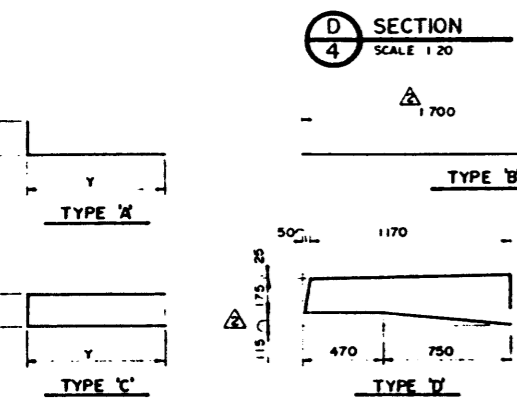
BAR TYPES NOTE: ALL BAR DIMENSIONS ARE OUT TO OUT
