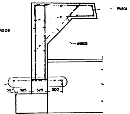
G SECTION SCALE 1/20
