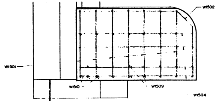
A SECTION SCALE 1/20
