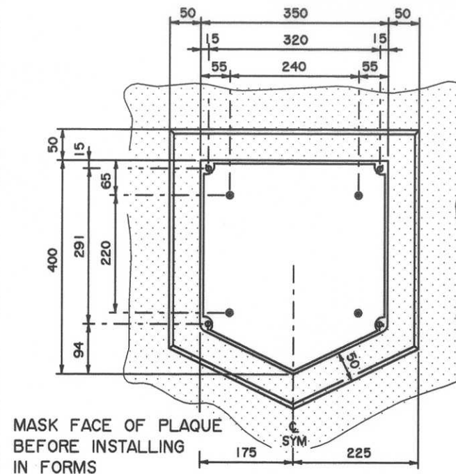
INSTALLATION DETAILS
