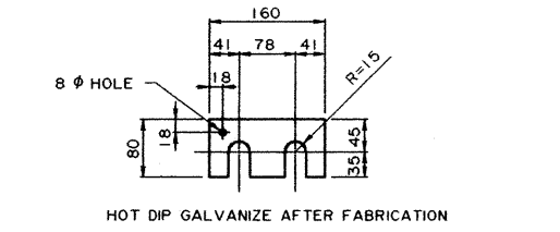
DROP-IN WASHER S-1603-94 1:5 FOR SC-510 GIRDER TO GIRDER CONNECTIONS IN 2 mm AND 4 mm THICKNESSES
