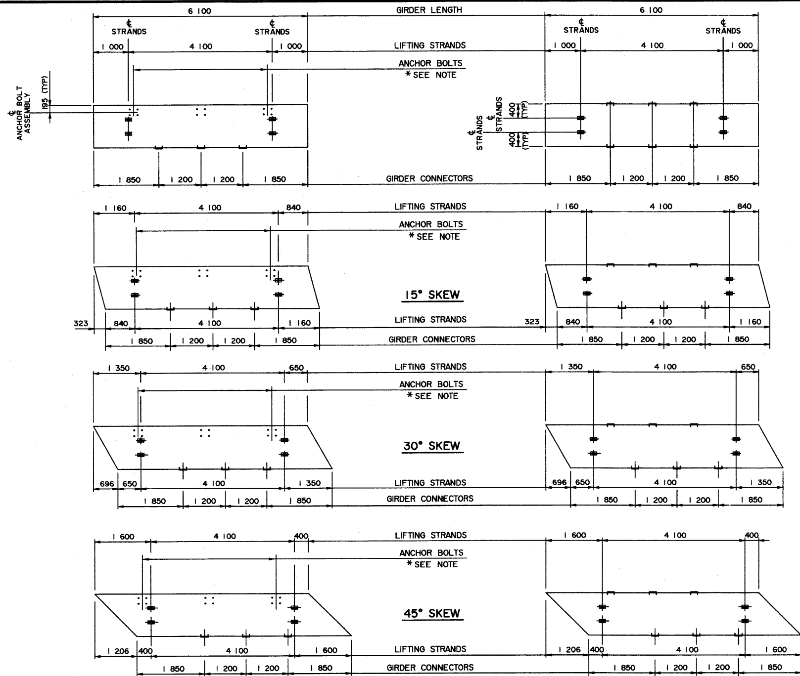
EXTERIOR GIRDER 1:50
