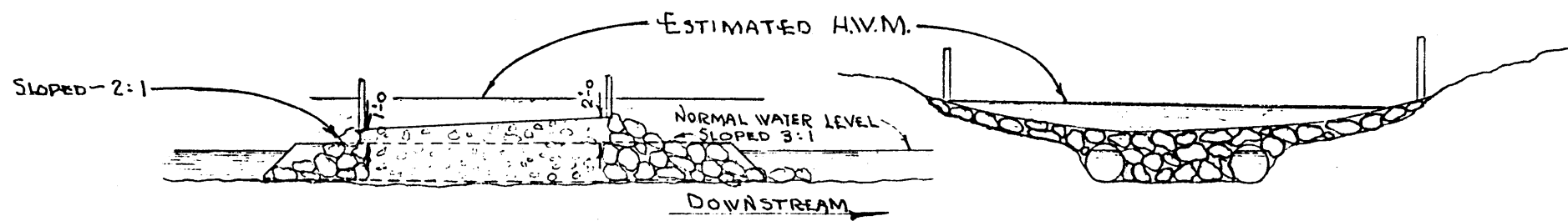
CROSS-SECTION
