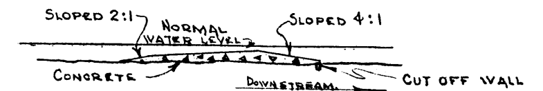
SECTION AA
