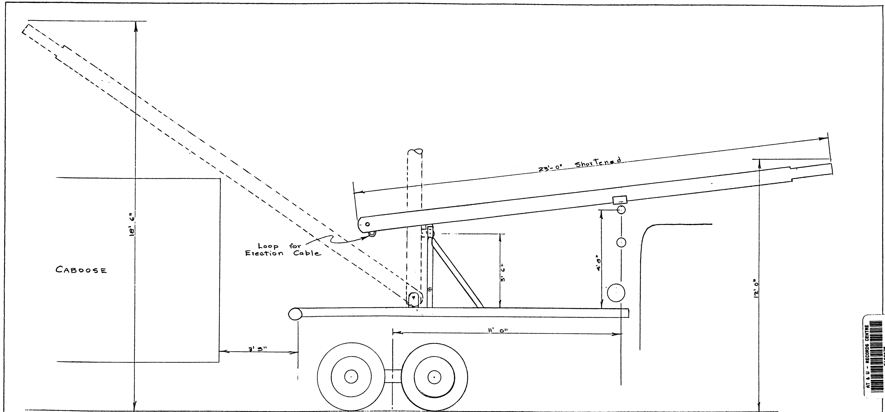
BOOM TRUCK PIVOT BRACKET SCALE 1/2" = 1'-0" D.G.L. 5-560 April 1, 1953
