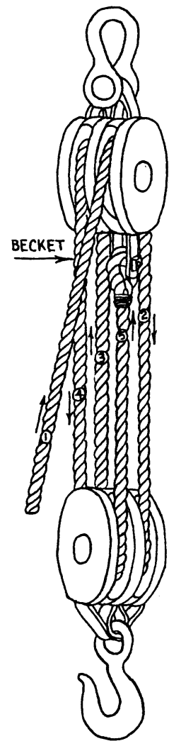
DOUBLE AND DOUBLE
