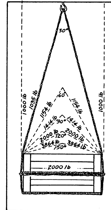
WEIGHTS OF PULL EXERTED ON SLINGS OF VARIOUS ANGLES
