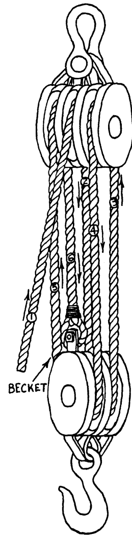
TRIPLE AND DOUBLE
