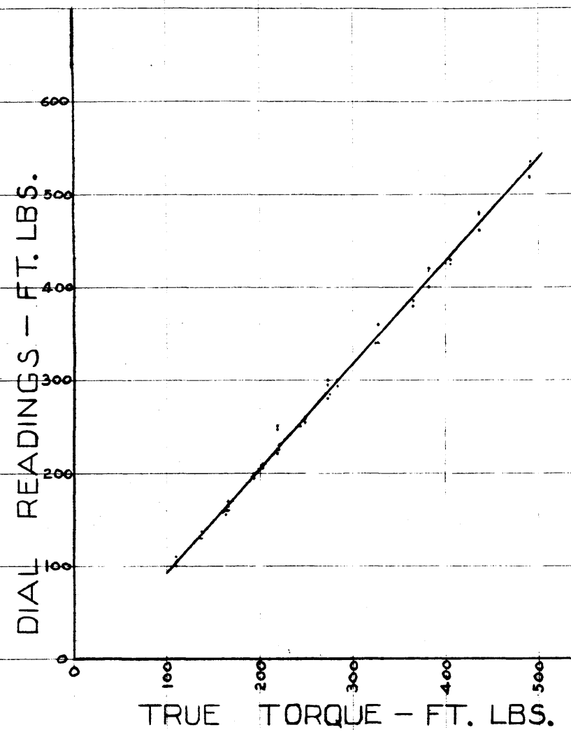
CALIBRATION CURVE FOR TORQUE WRENCH - Serial No. 1076
